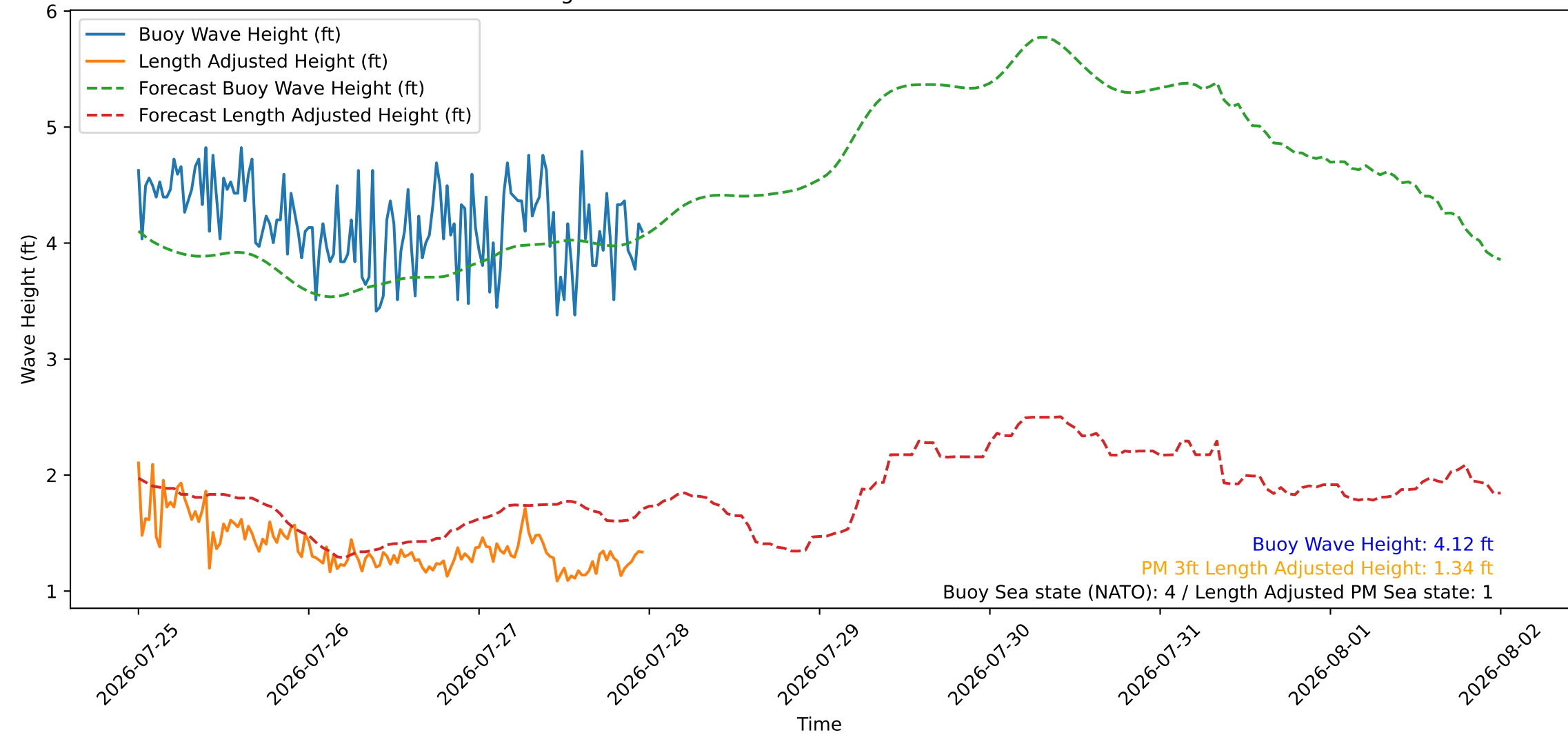
Wave Heights over Time for Green Beach at 2026-07-28 00:01:07
