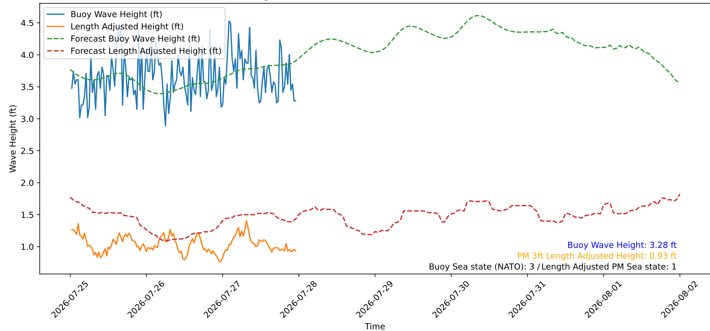
Wave Heights over Time for Red Beach at 2026-07-28 00:00:45
