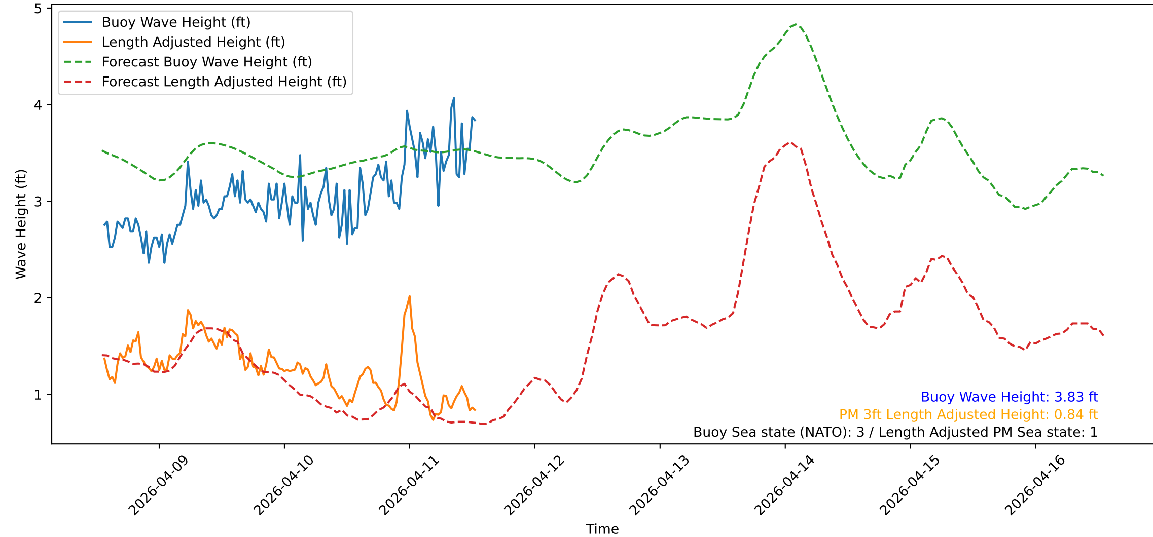
Wave Heights over Time for Green Beach at 2026-04-11 13:21:14
