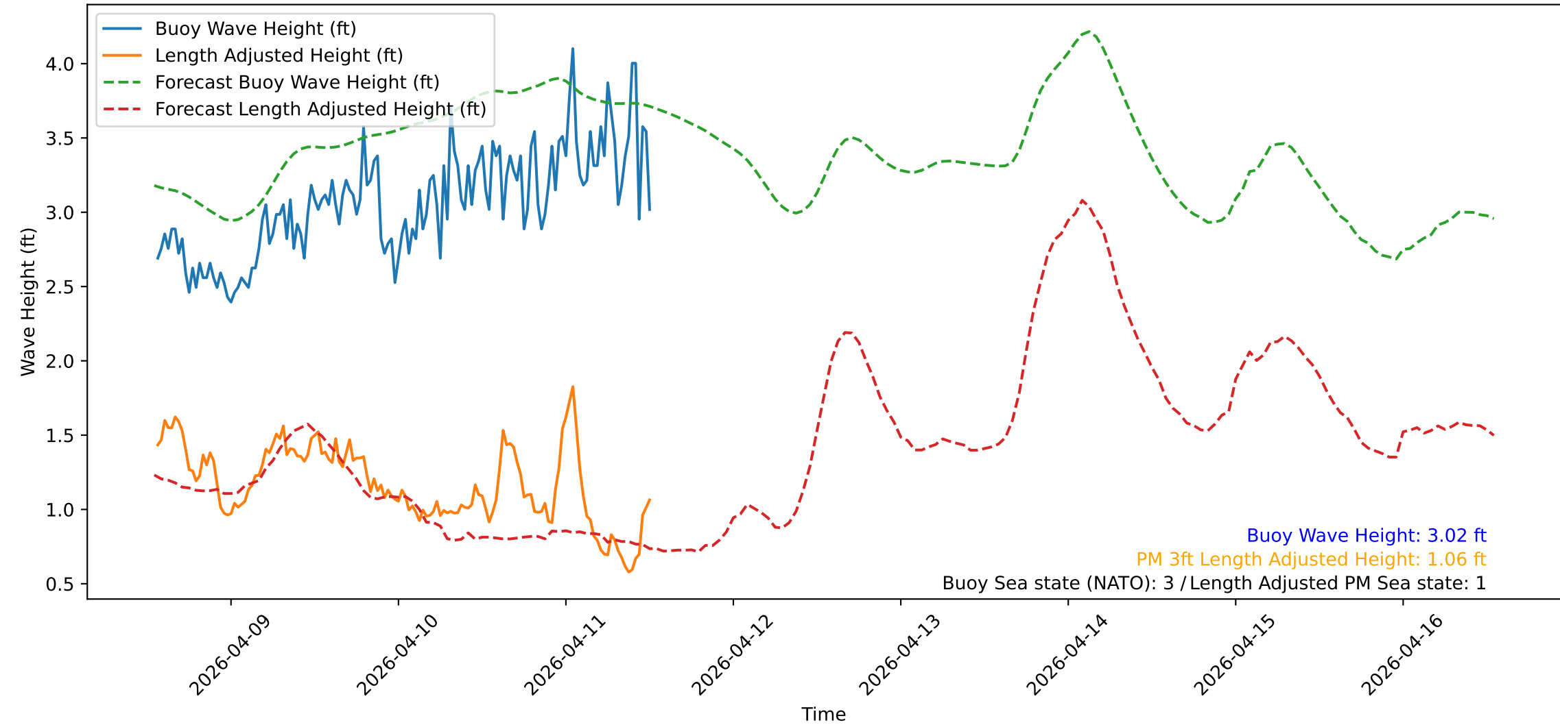
Wave Heights over Time for Red Beach at 2026-04-11 13:20:52
