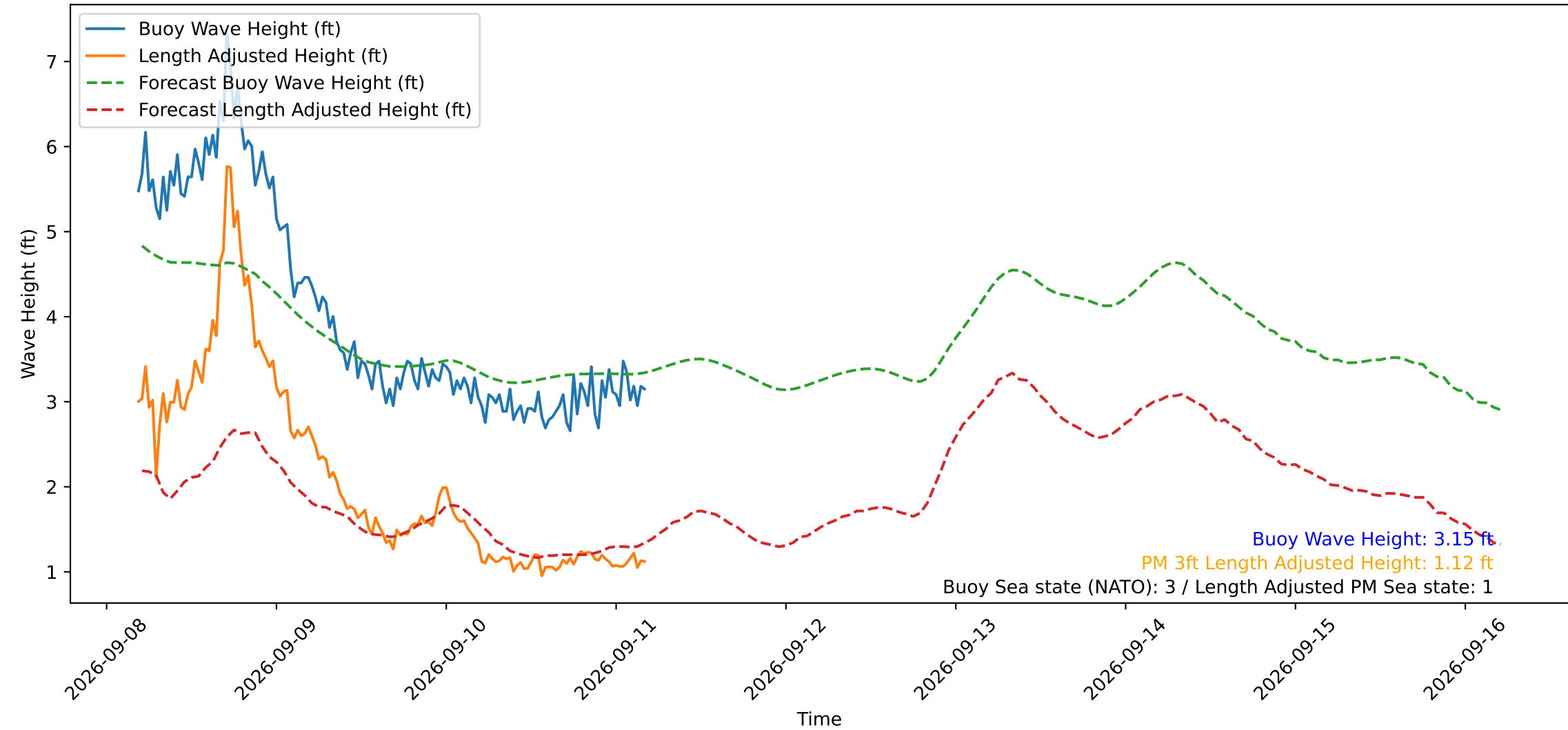
Wave Heights over Time for Oceanside Harbor at 2026-09-11 04:40:29
