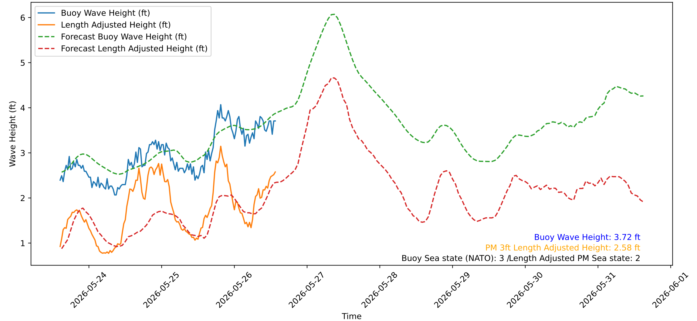
Wave Heights over Time for Green Beach at 2026-05-26 14:41:09
