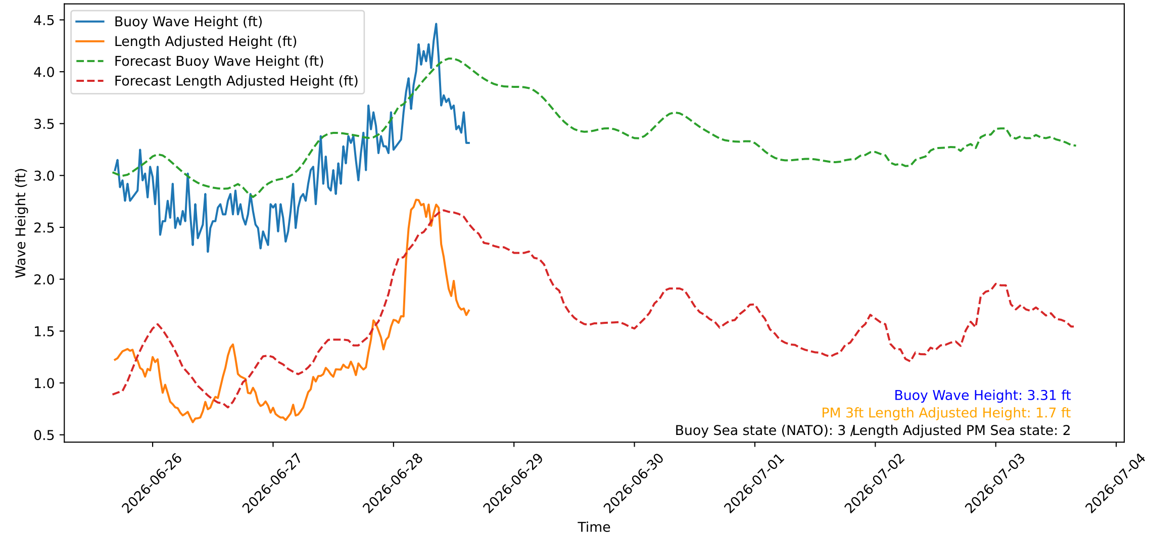
Wave Heights over Time for Red Beach at 2026-06-28 16:00:45
