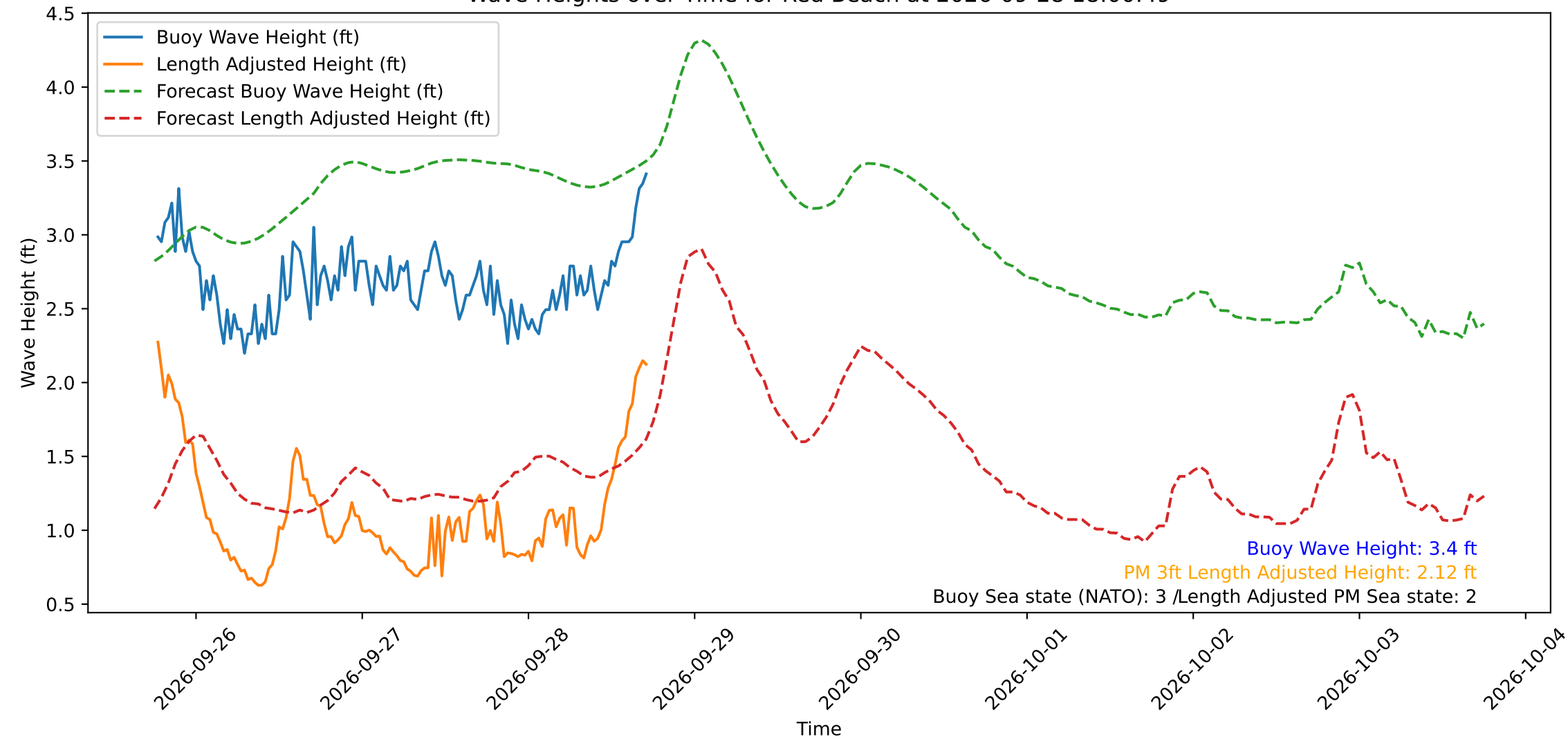
Wave Heights over Time for Red Beach at 2026-09-28 18:00:49
