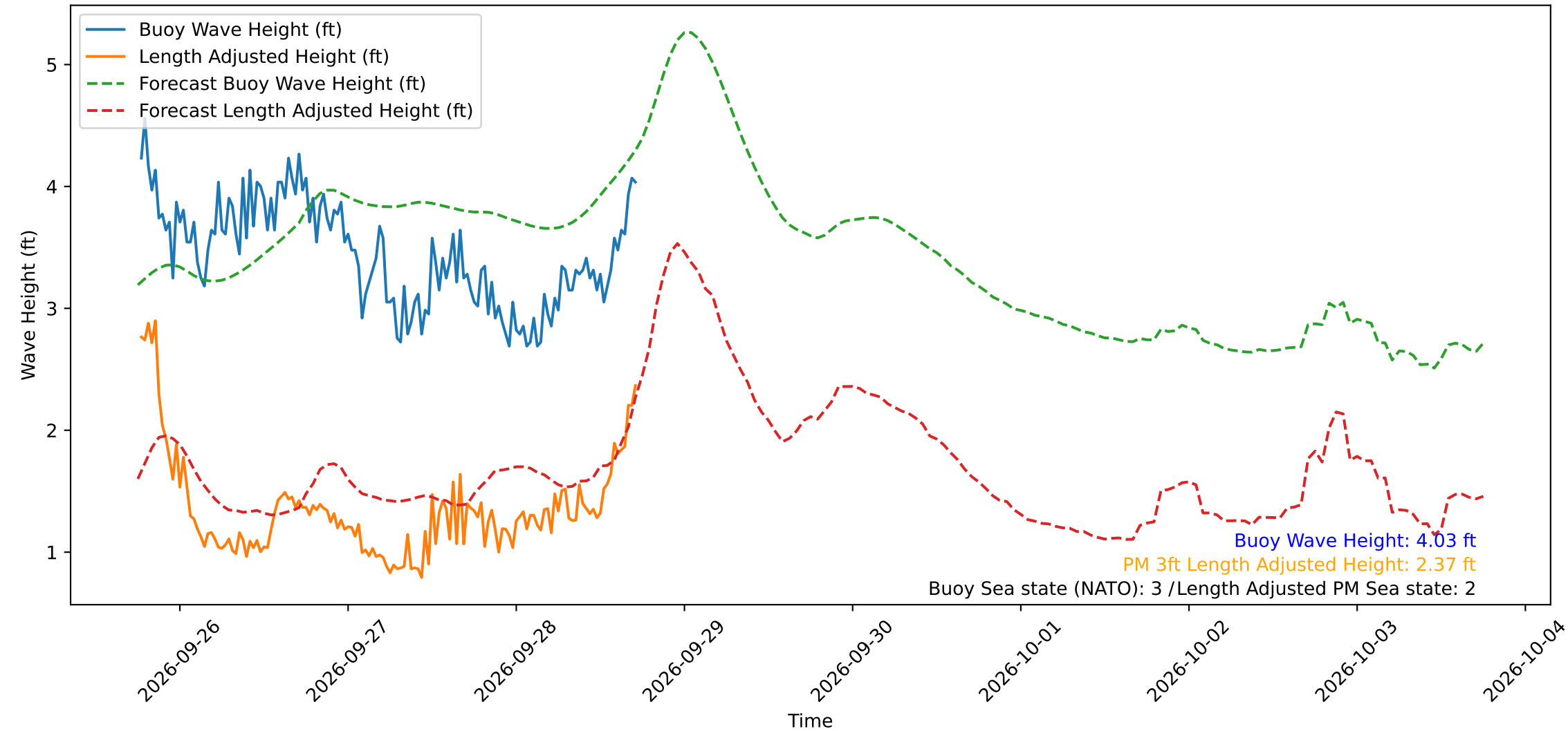
Wave Heights over Time for Green Beach at 2026-09-28 18:01:12
