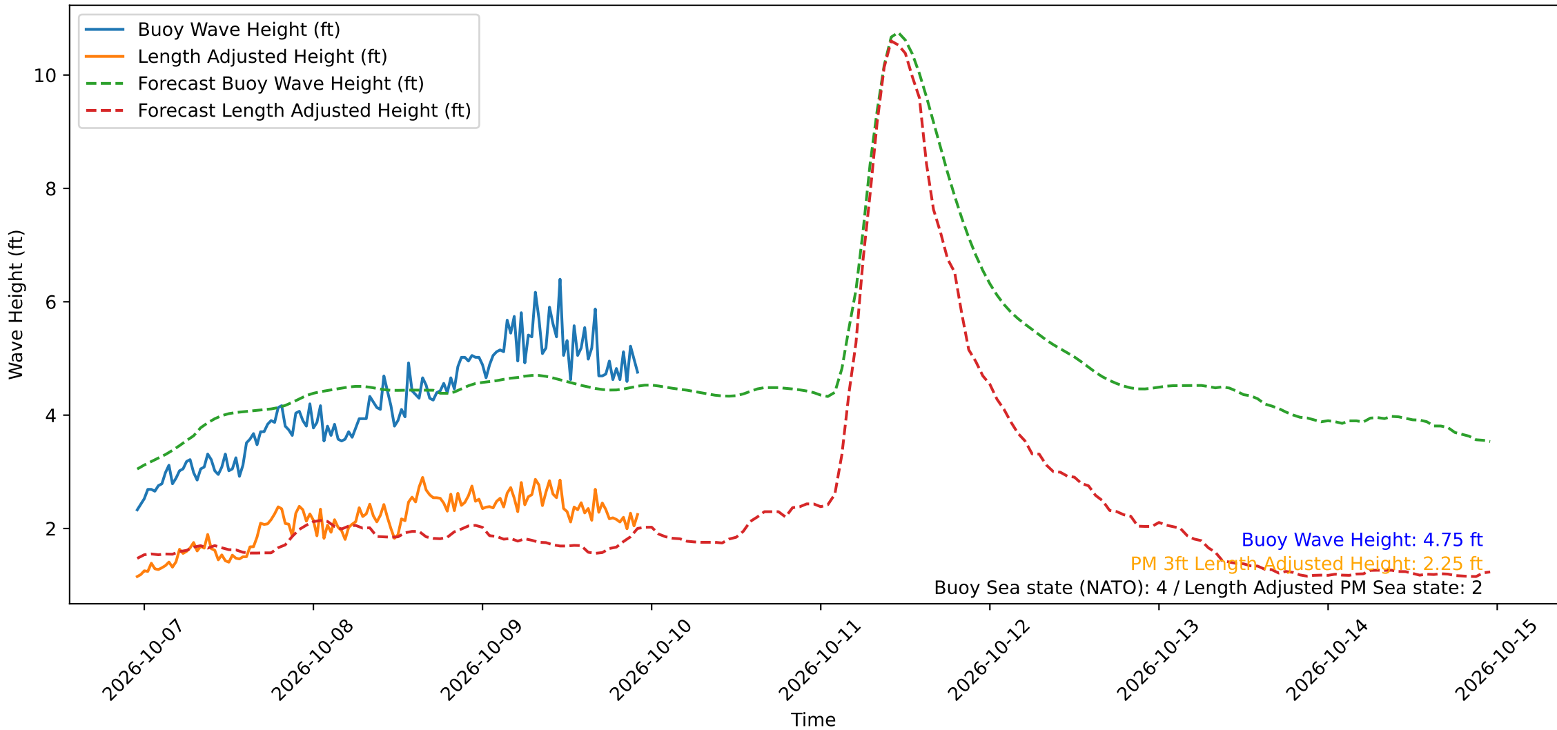
Wave Heights over Time for Oceanside Harbor at 2026-10-09 23:00:30
