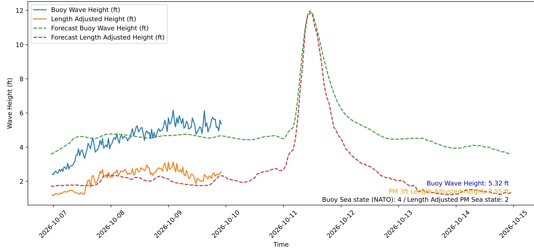
Wave Heights over Time for Green Beach at 2026-10-09 23:01:12
