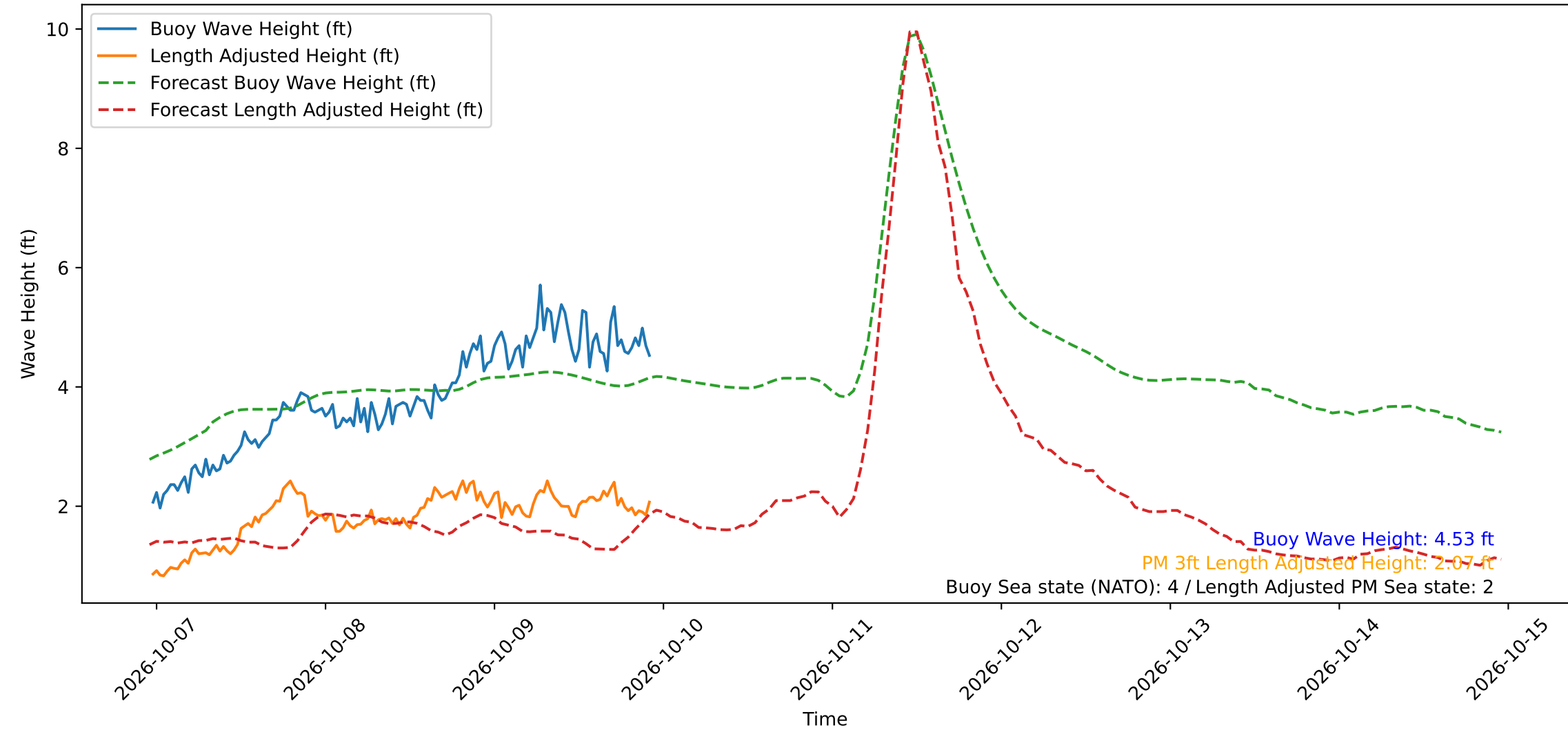
Wave Heights over Time for Red Beach at 2026-10-09 23:00:50
