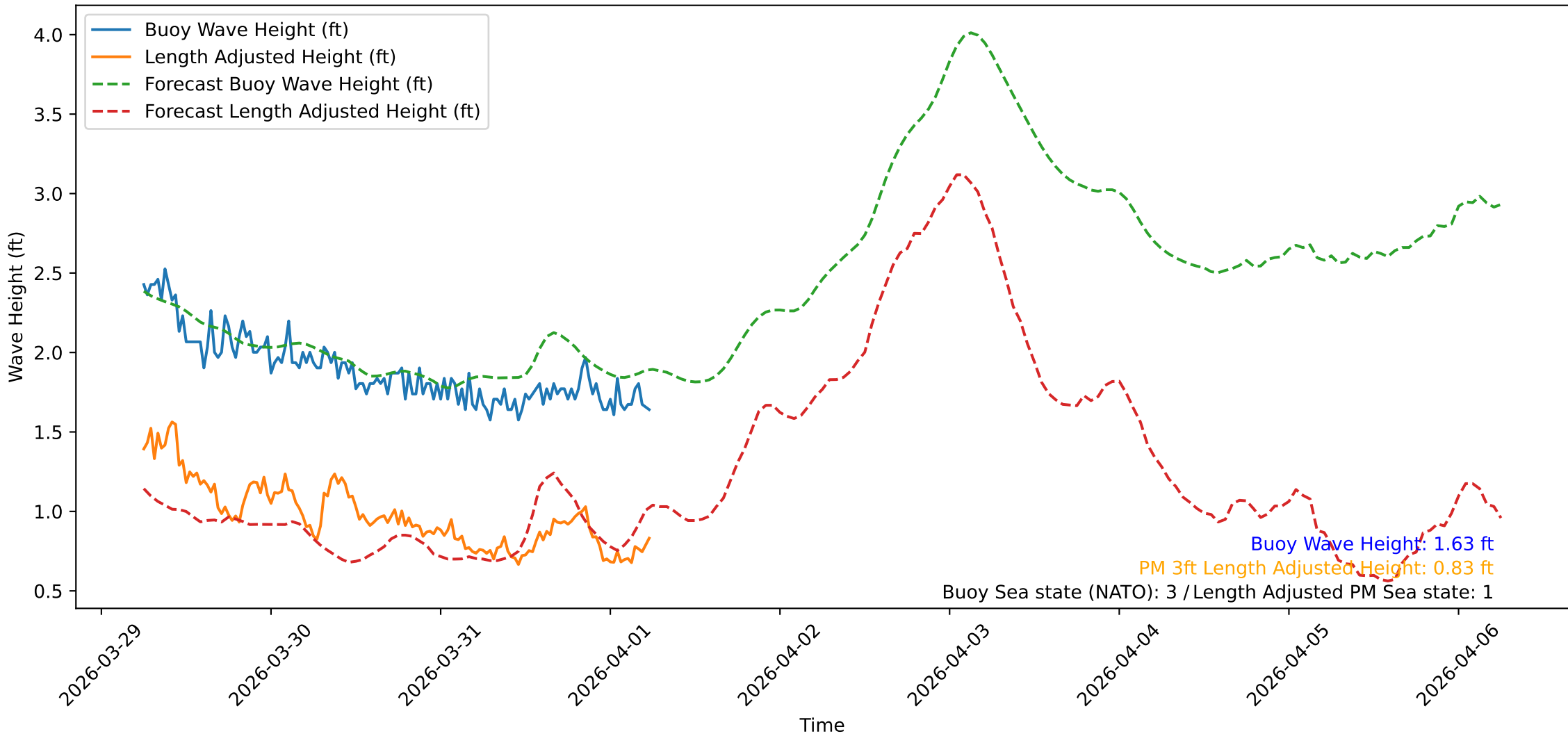
Wave Heights over Time for Oceanside Harbor at 2026-04-01 06:00:31
