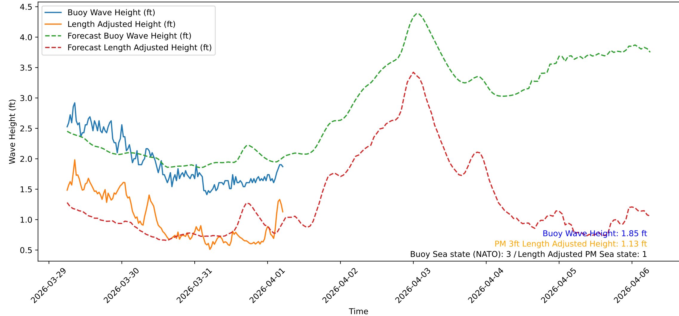
Wave Heights over Time for Green Beach at 2026-04-01 06:01:10
