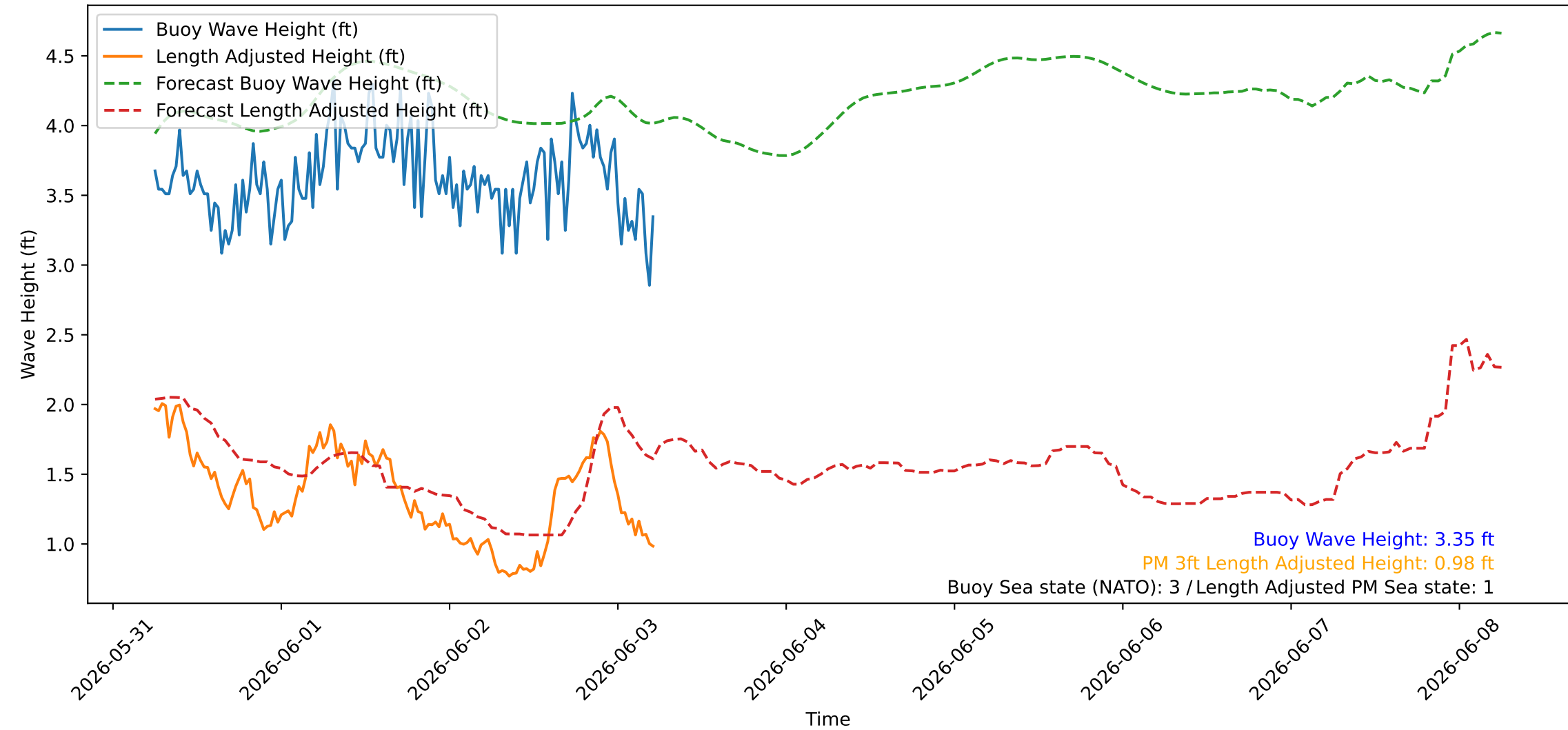
Wave Heights over Time for Green Beach at 2026-06-03 05:51:08
