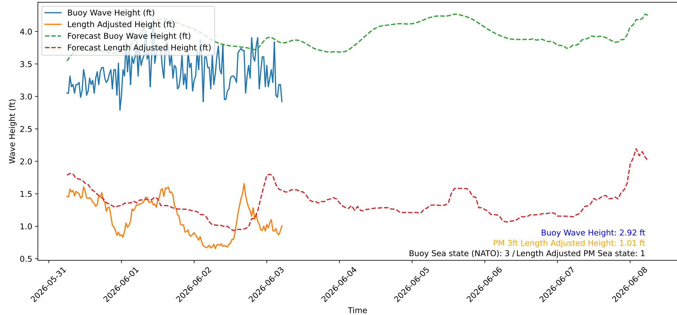
Wave Heights over Time for Red Beach at 2026-06-03 05:50:46
