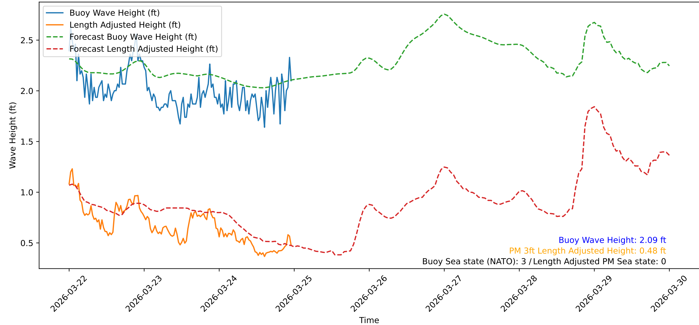
Wave Heights over Time for Red Beach at 2026-03-24 23:40:47
