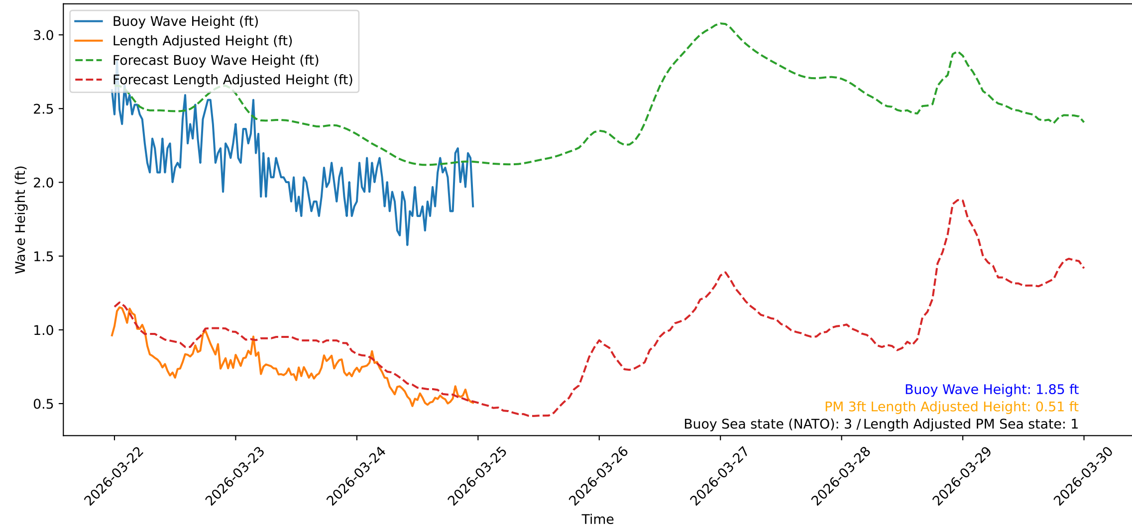
Wave Heights over Time for Oceanside Harbor at 2026-03-24 23:40:31
