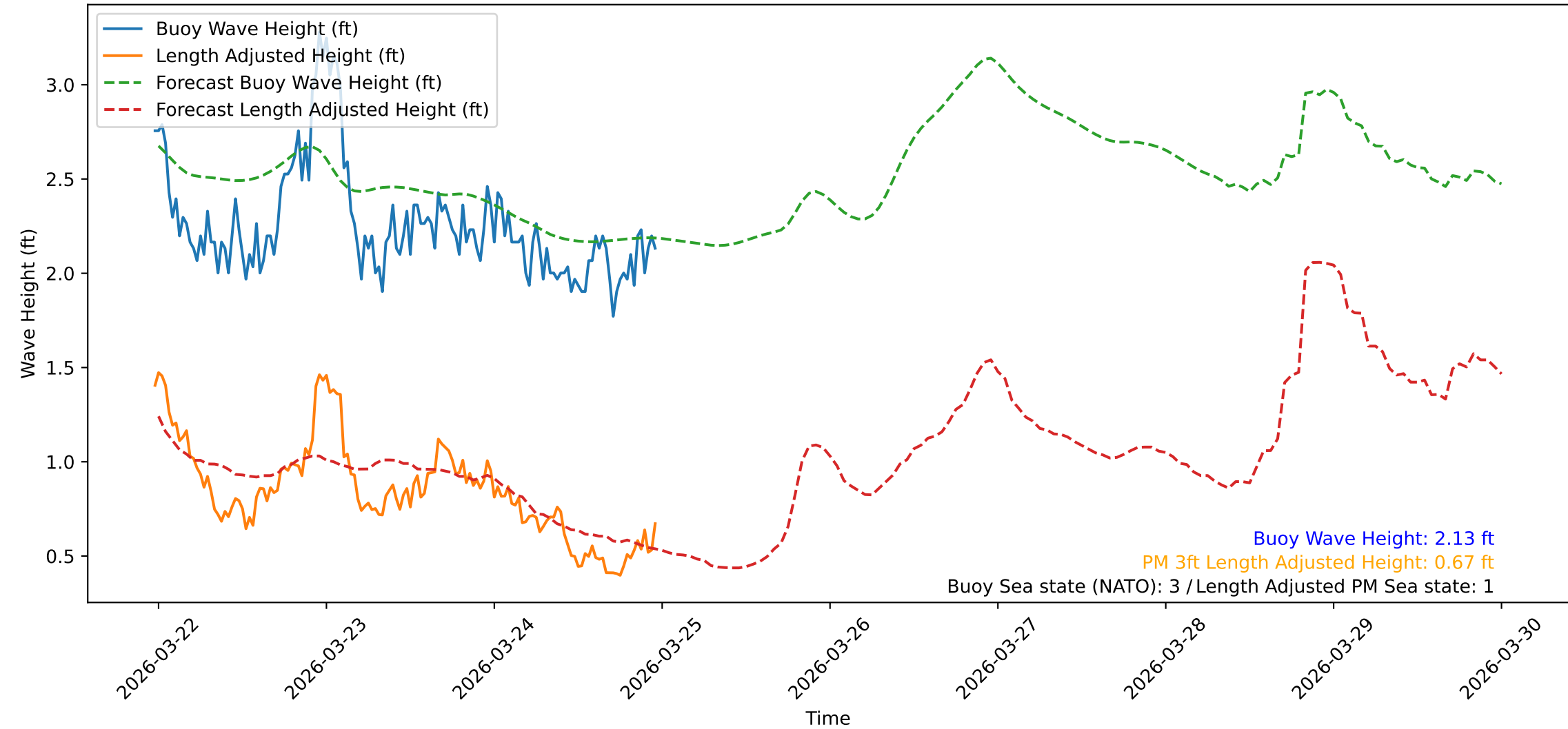
Wave Heights over Time for Green Beach at 2026-03-24 23:41:10
