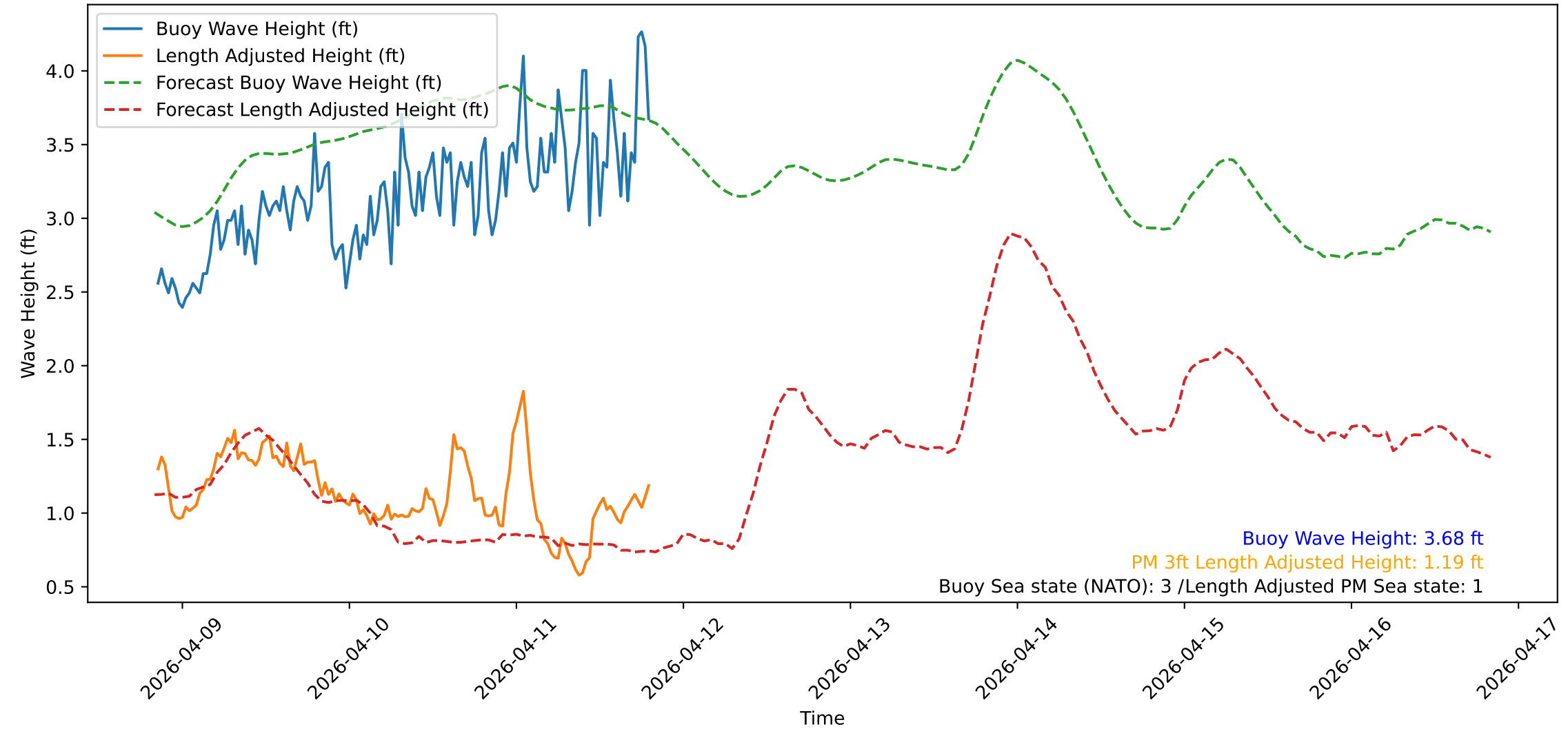
Wave Heights over Time for Red Beach at 2026-04-11 20:20:51
