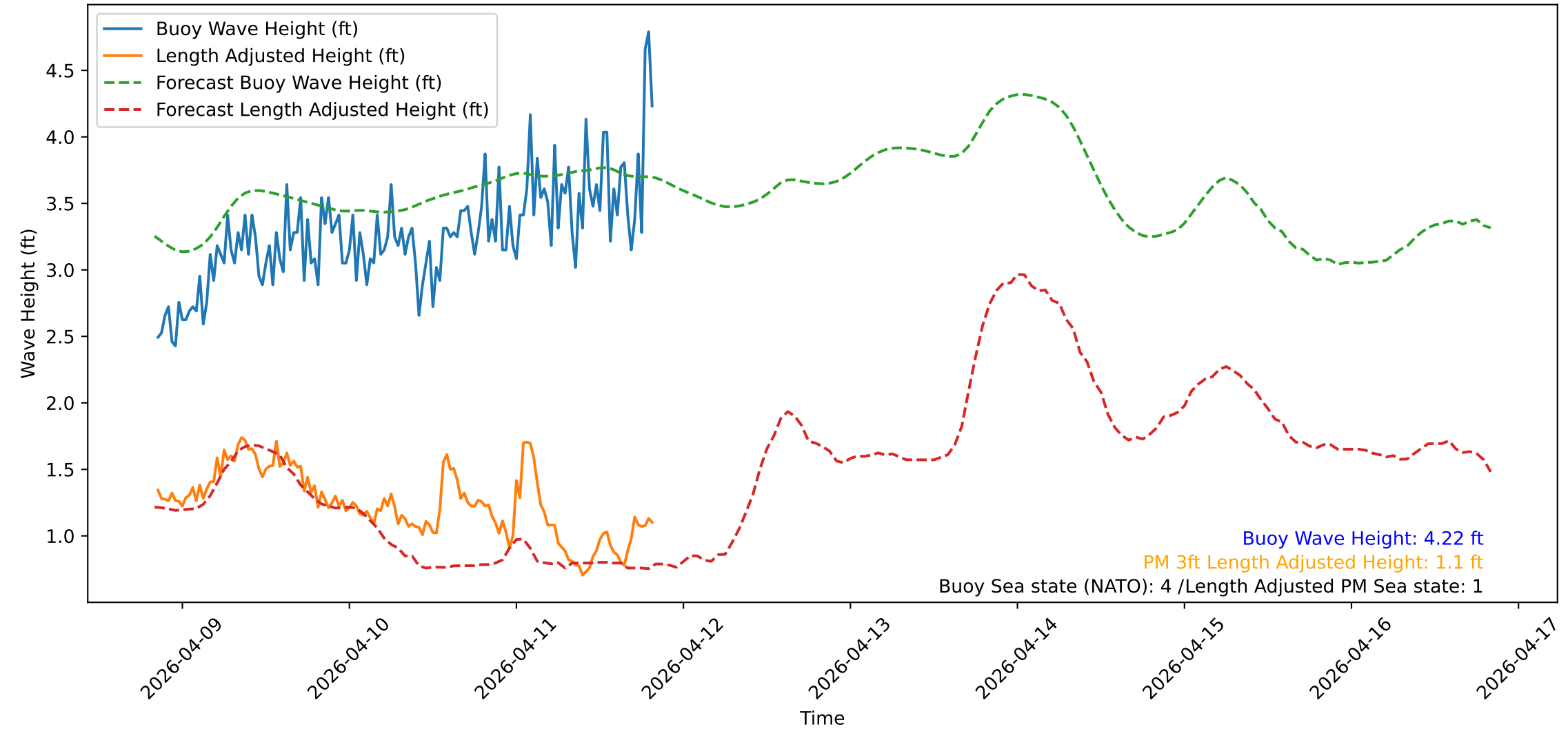
Wave Heights over Time for Oceanside Harbor at 2026-04-11 20:20:31
