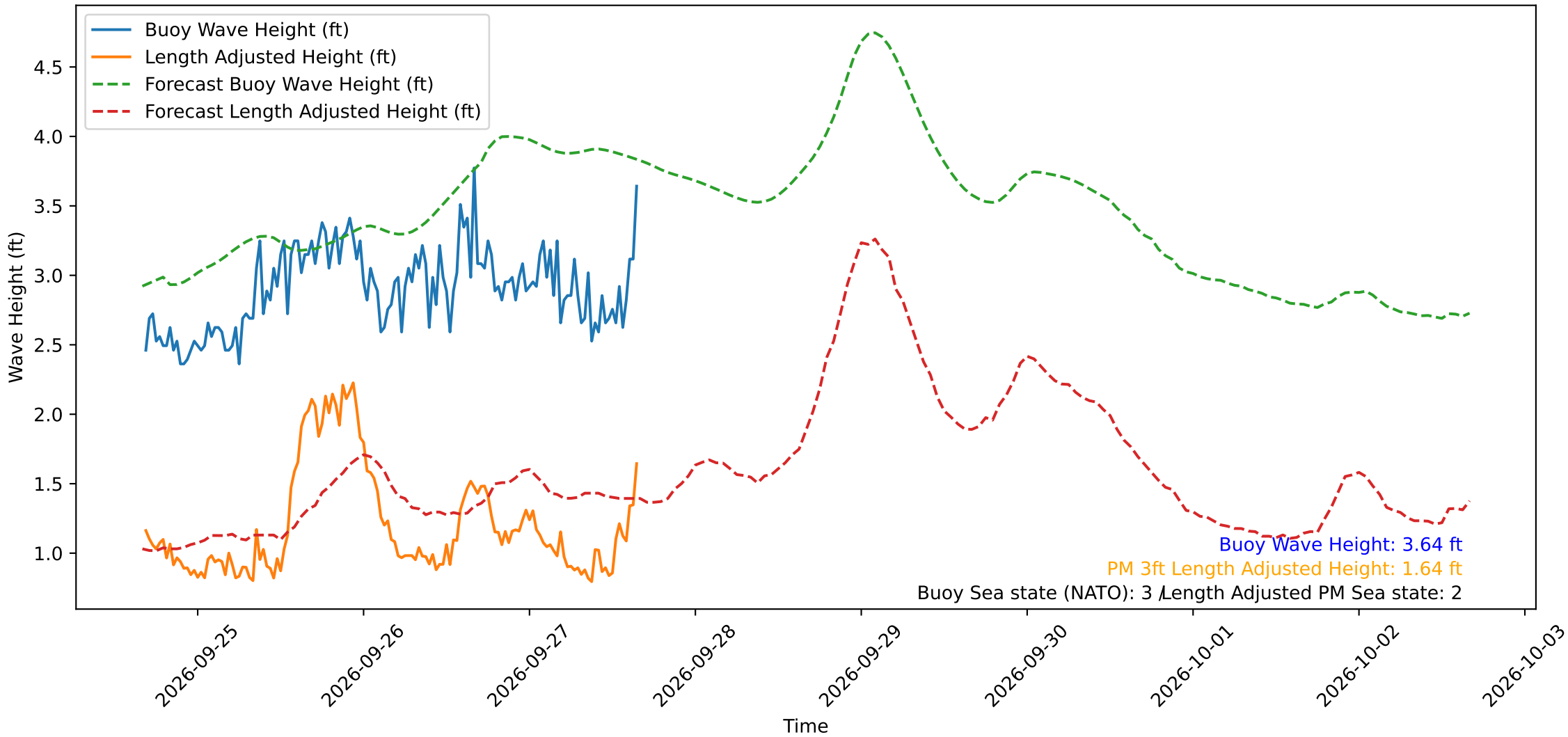
Wave Heights over Time for Oceanside Harbor at 2026-09-27 16:20:29
