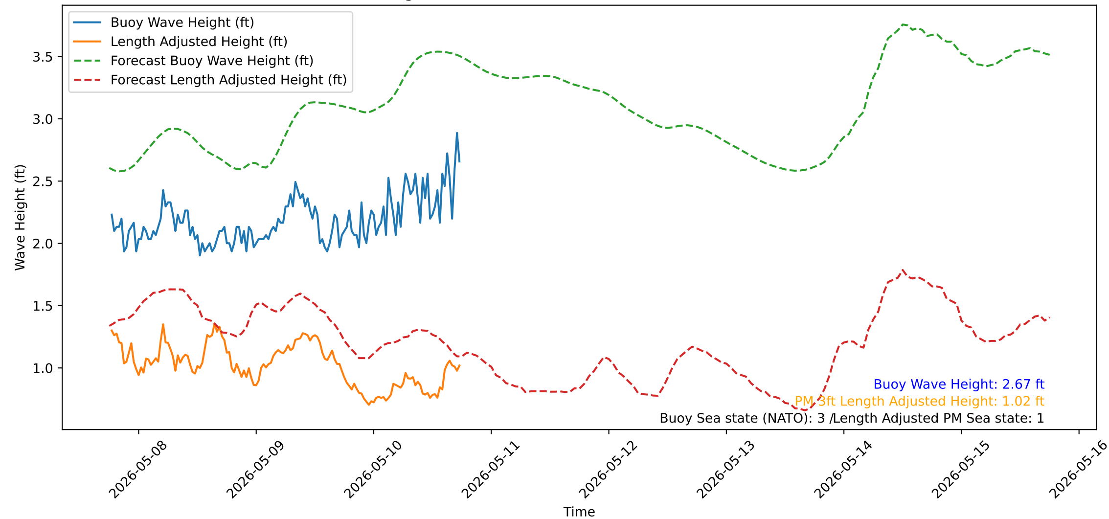
Wave Heights over Time for Red Beach at 2026-05-10 18:10:51
