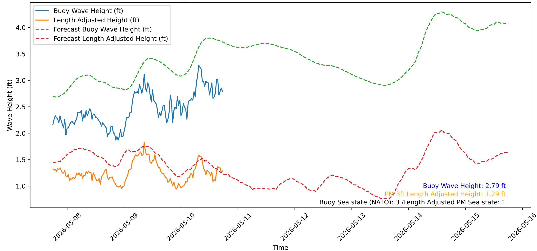
Wave Heights over Time for Oceanside Harbor at 2026-05-10 18:10:31
