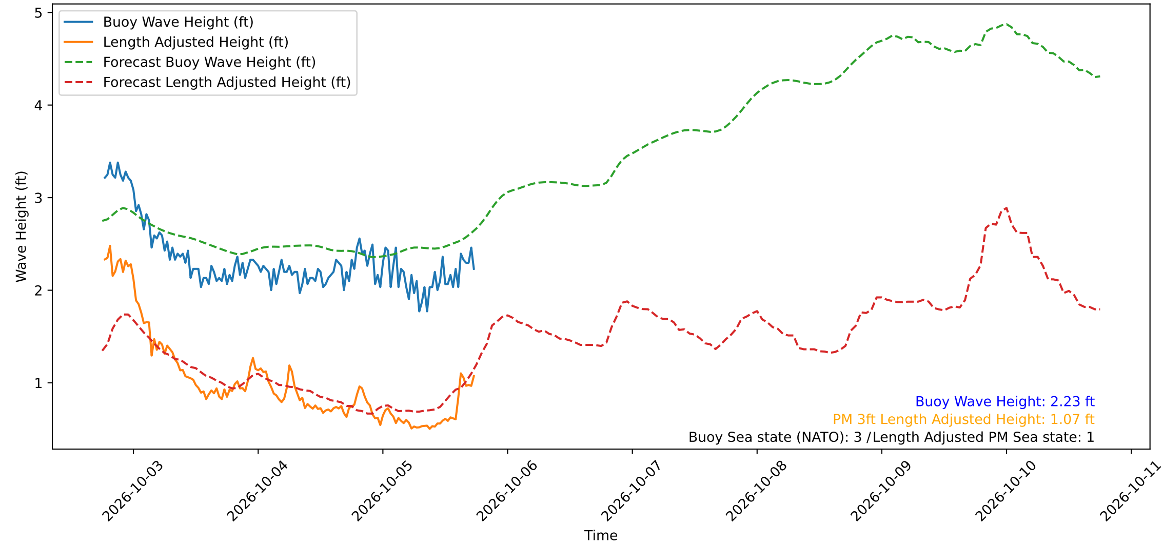
Wave Heights over Time for Green Beach at 2026-10-05 18:21:16
