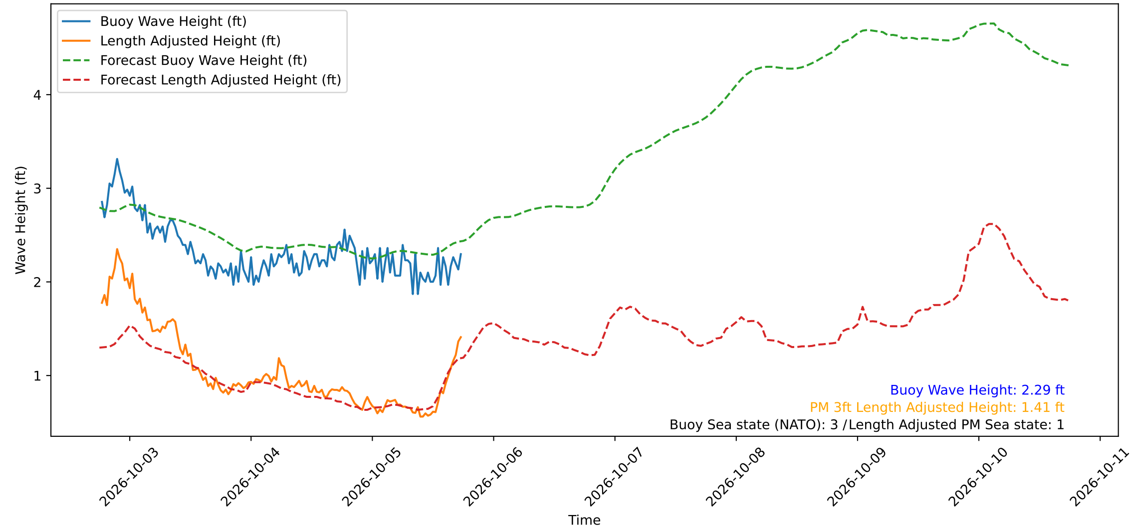
Wave Heights over Time for Oceanside Harbor at 2026-10-05 18:20:30
