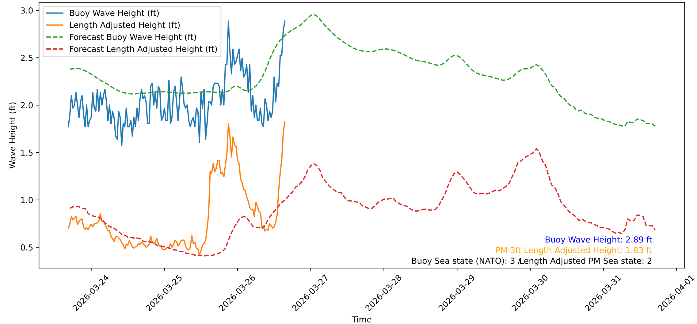
Wave Heights over Time for Oceanside Harbor at 2026-03-26 16:40:30
