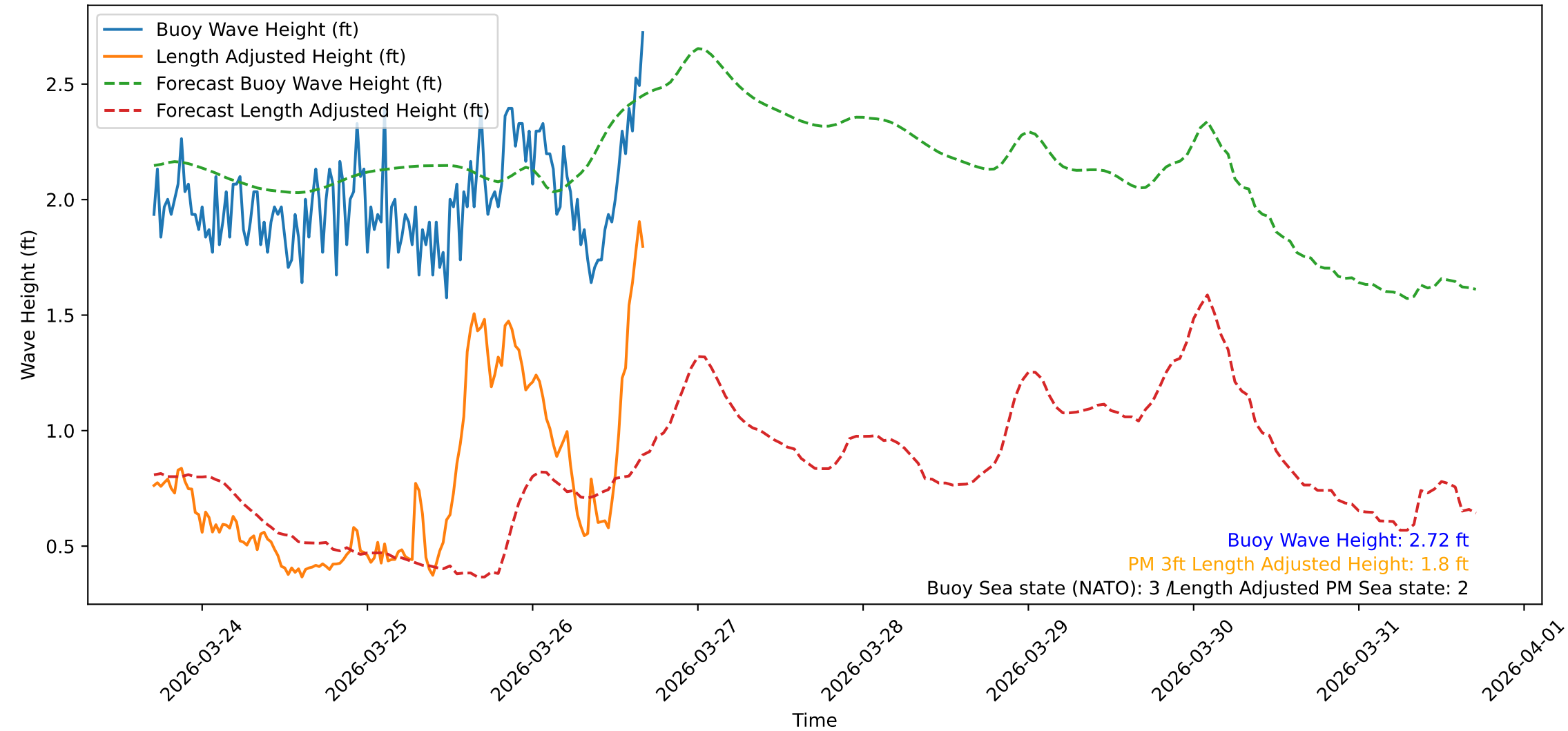
Wave Heights over Time for Red Beach at 2026-03-26 16:40:46
