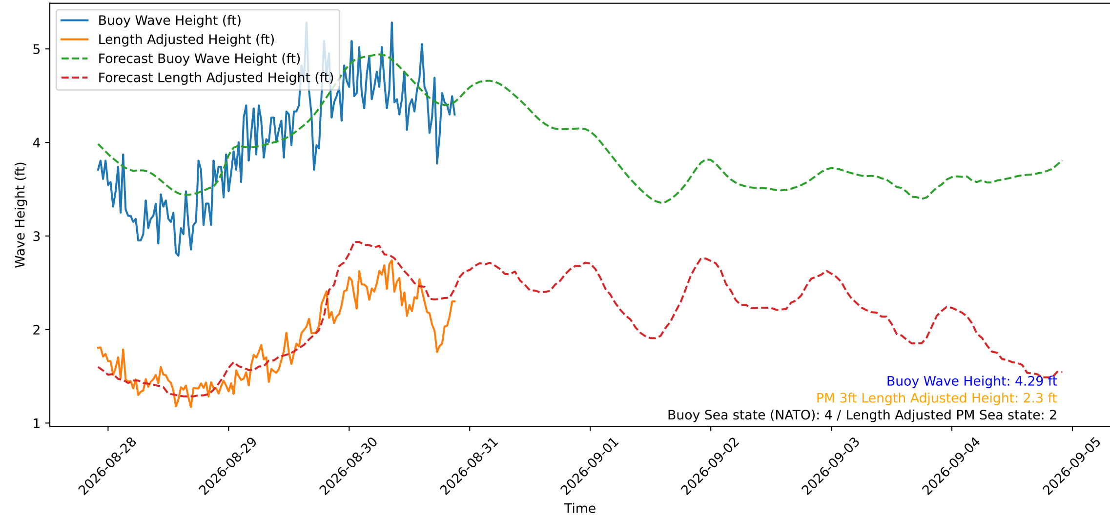
Wave Heights over Time for Oceanside Harbor at 2026-08-30 21:50:30
