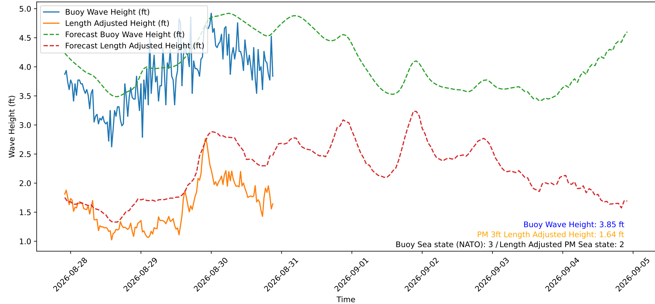
Wave Heights over Time for Green Beach at 2026-08-30 21:51:14
