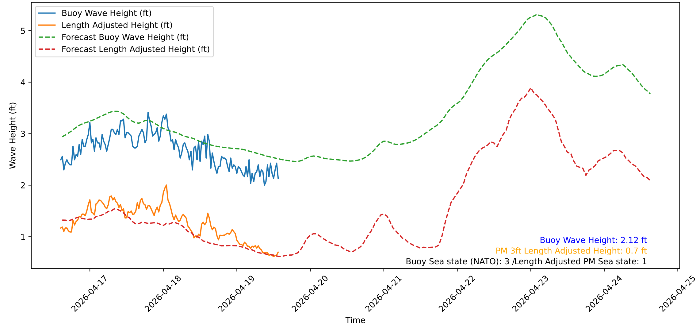
Wave Heights over Time for Oceanside Harbor at 2026-04-19 14:30:32
