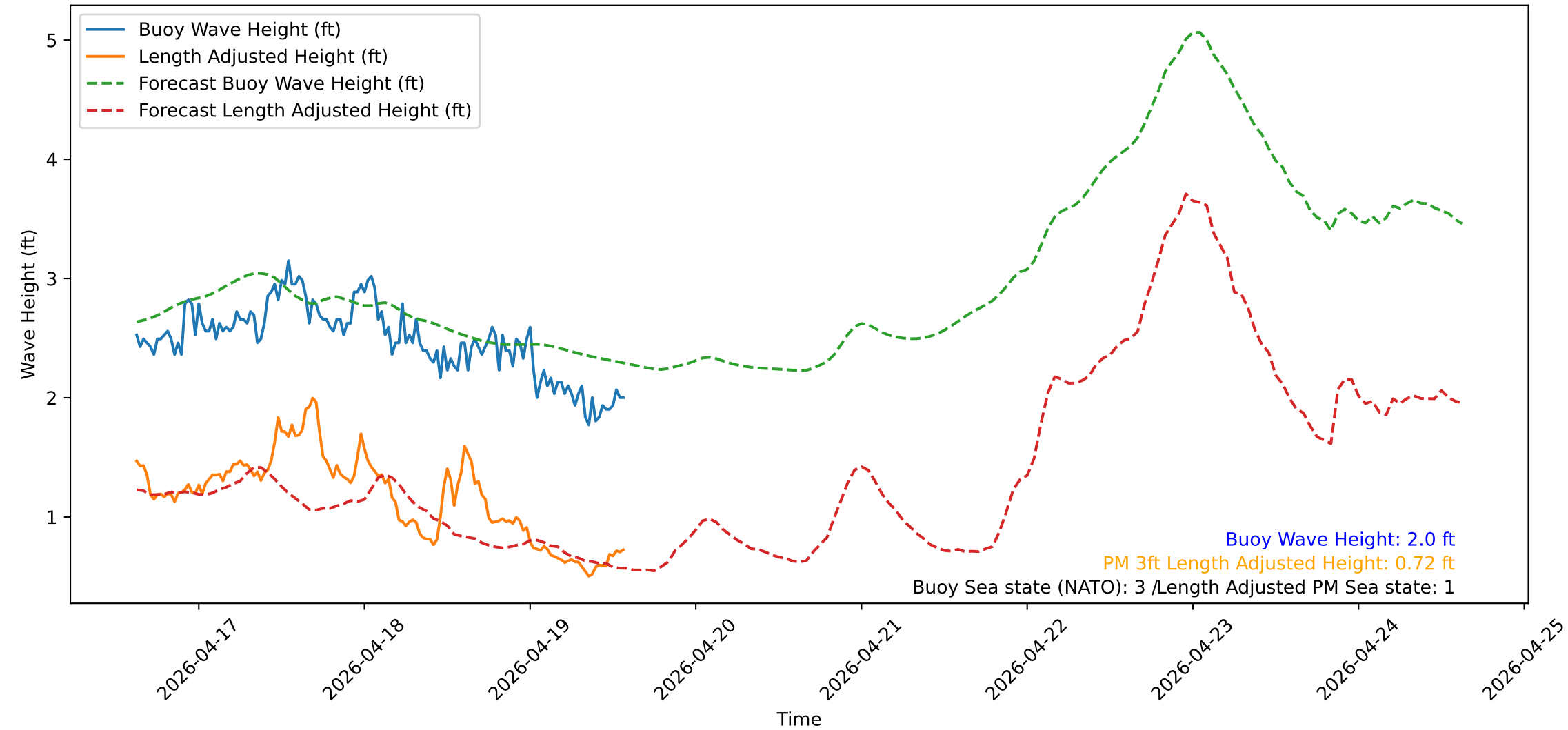
Wave Heights over Time for Red Beach at 2026-04-19 14:30:51
