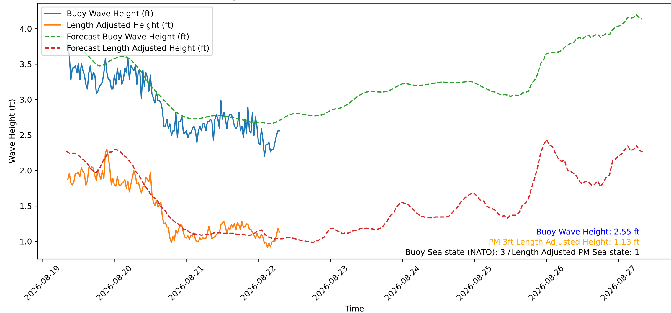
Wave Heights over Time for Oceanside Harbor at 2026-08-22 08:20:30
