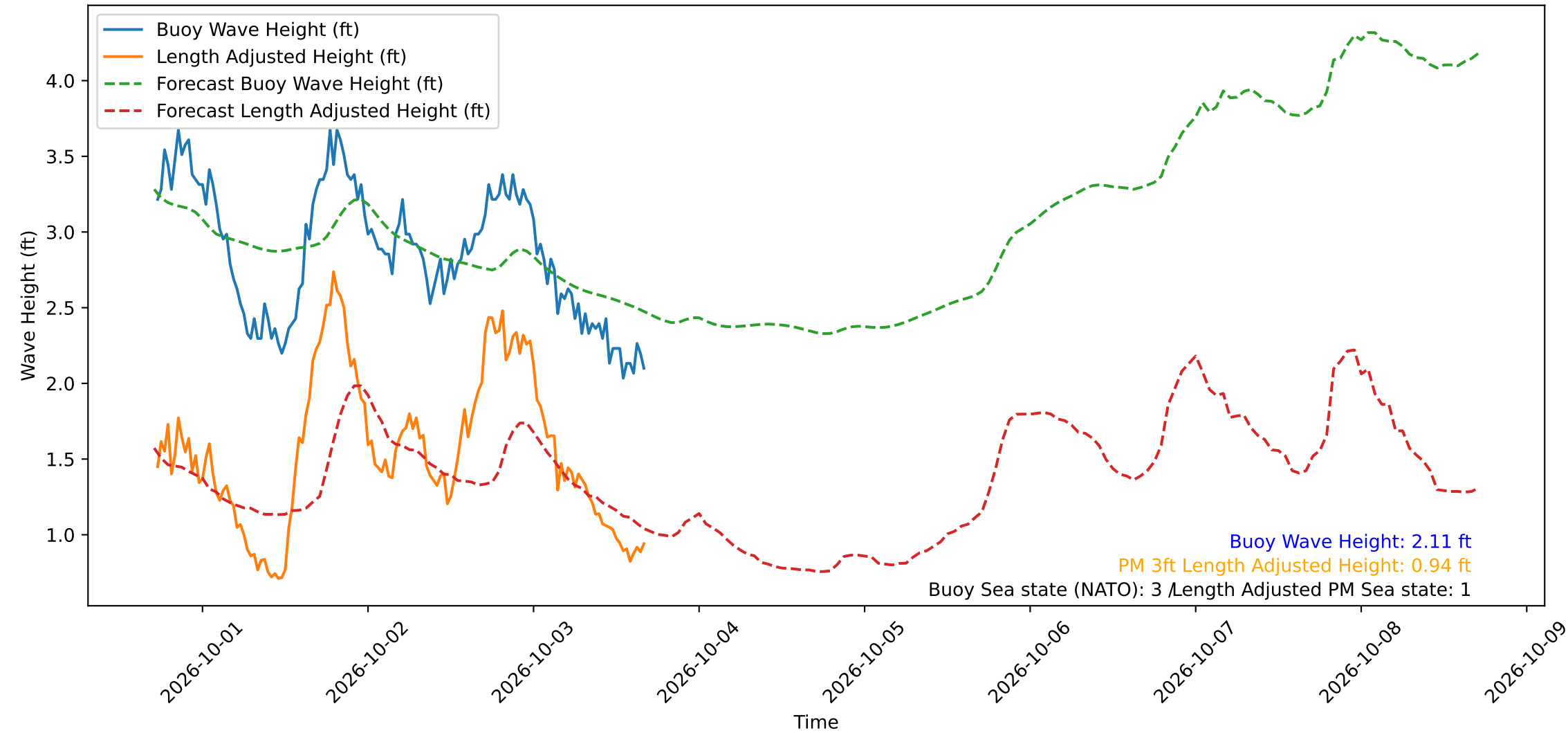
Wave Heights over Time for Green Beach at 2026-10-03 17:01:12
