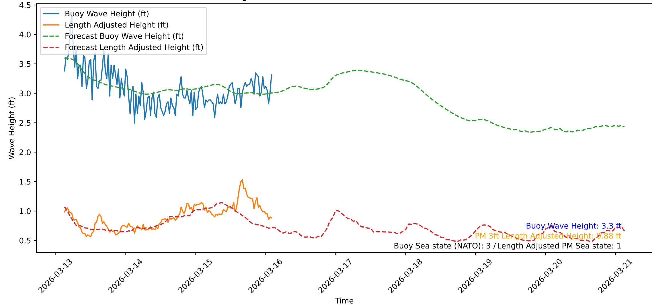
Wave Heights over Time for Red Beach at 2026-03-16 02:51:29
