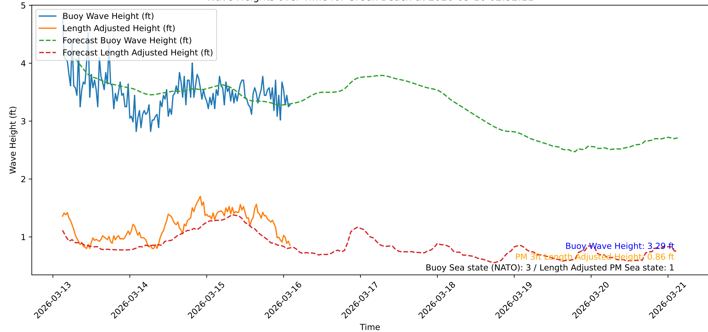
Wave Heights over Time for Green Beach at 2026-03-16 02:52:11
