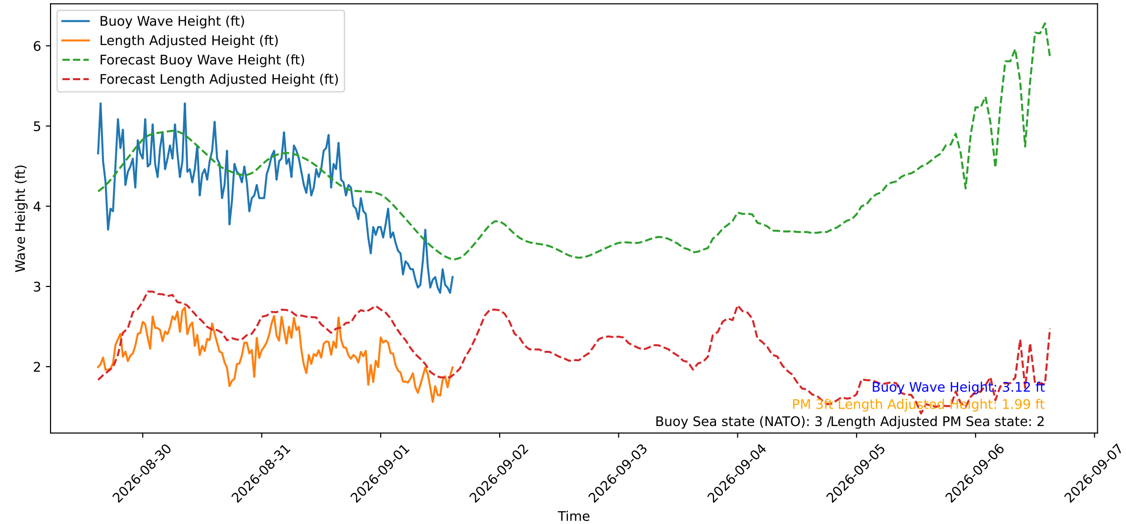
Wave Heights over Time for Oceanside Harbor at 2026-09-01 15:00:30
