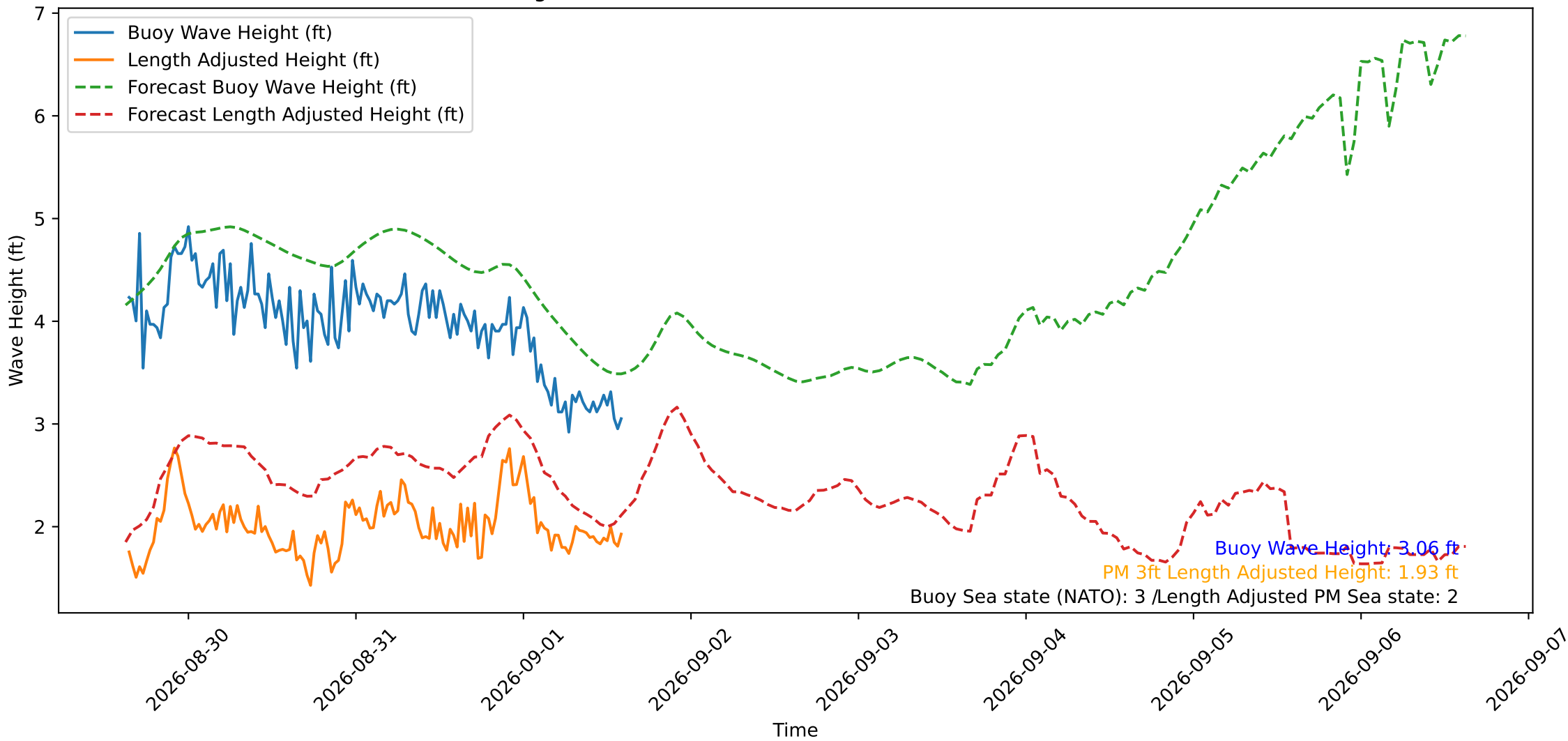
Wave Heights over Time for Green Beach at 2026-09-01 15:01:13
