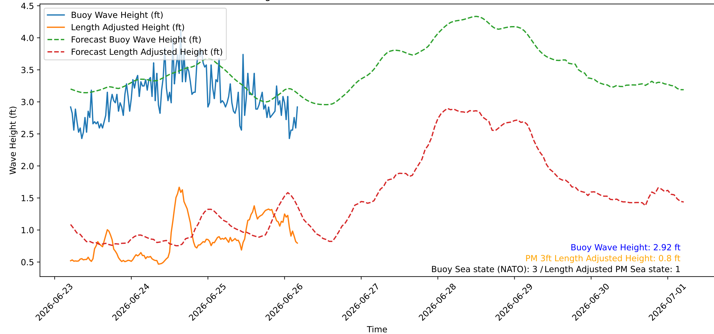
Wave Heights over Time for Red Beach at 2026-06-26 04:50:46
