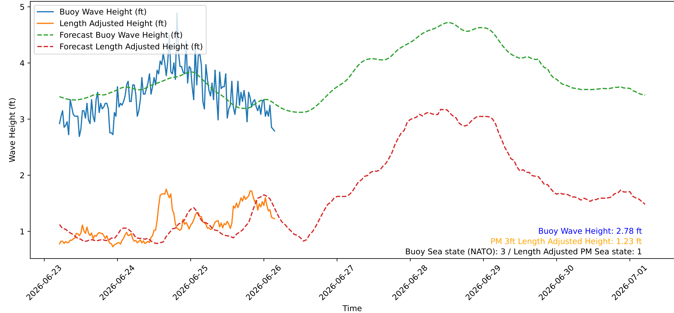
Wave Heights over Time for Oceanside Harbor at 2026-06-26 04:50:26
