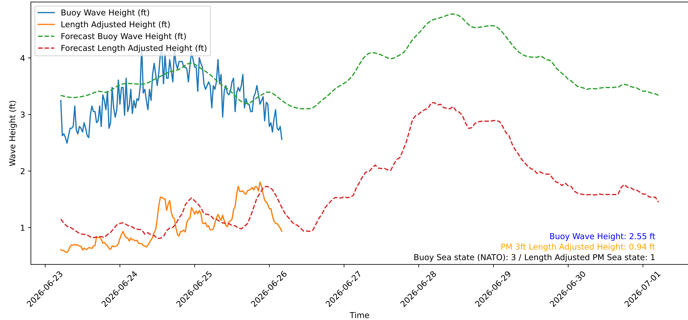
Wave Heights over Time for Green Beach at 2026-06-26 04:51:09
