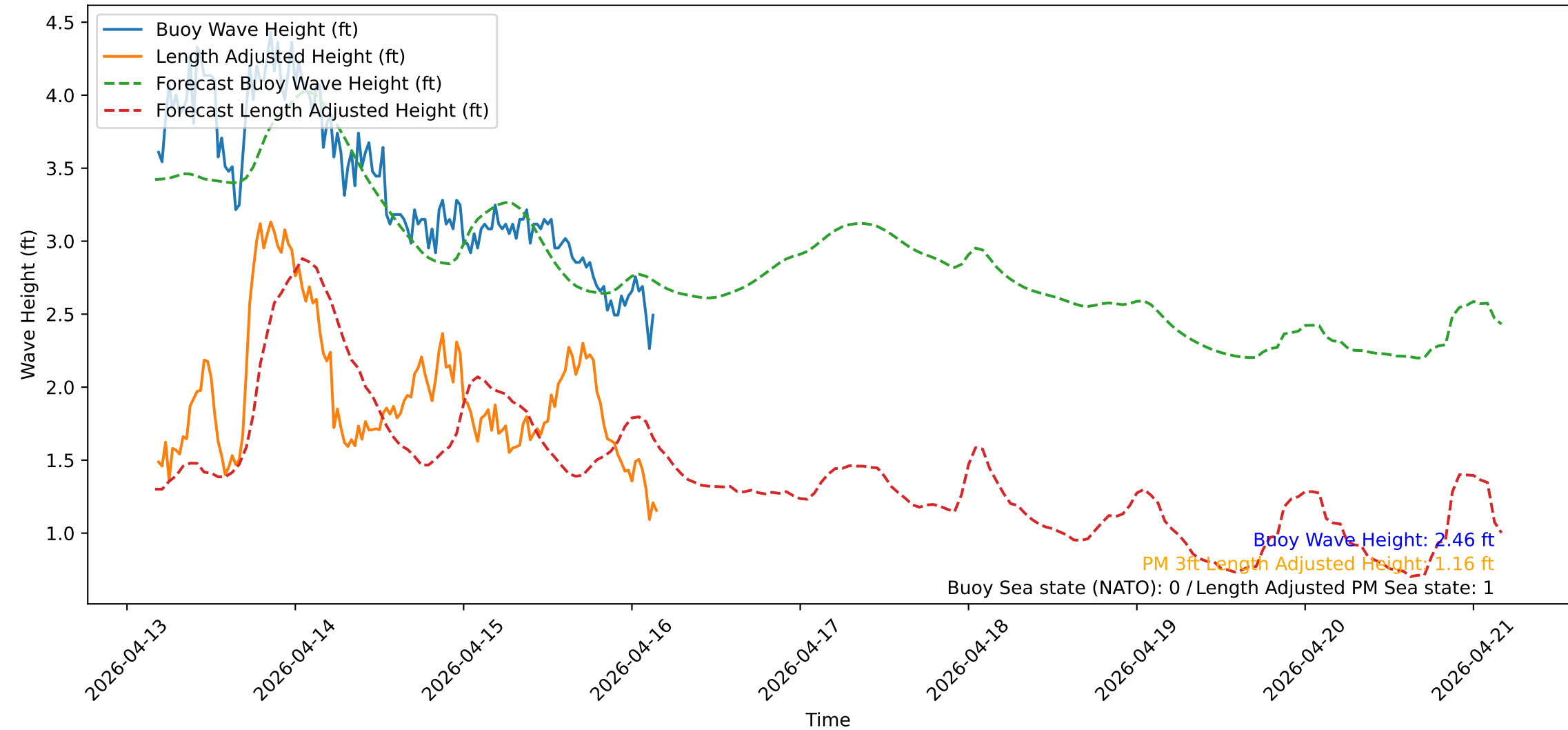
Wave Heights over Time for Red Beach at 2026-04-16 04:20:51
