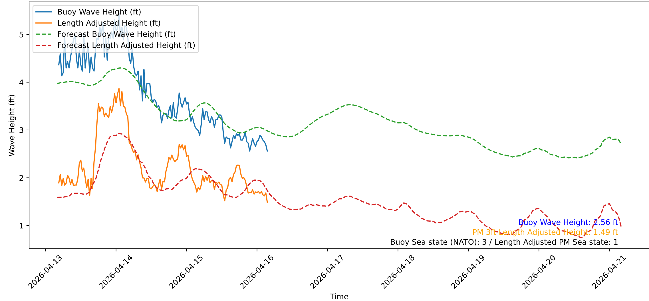
Wave Heights over Time for Oceanside Harbor at 2026-04-16 04:20:31
