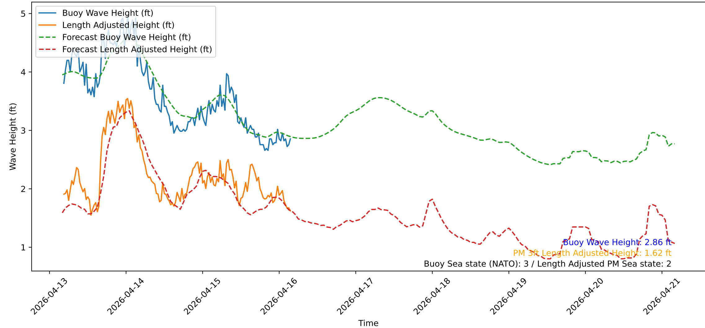
Wave Heights over Time for Green Beach at 2026-04-16 04:21:13
