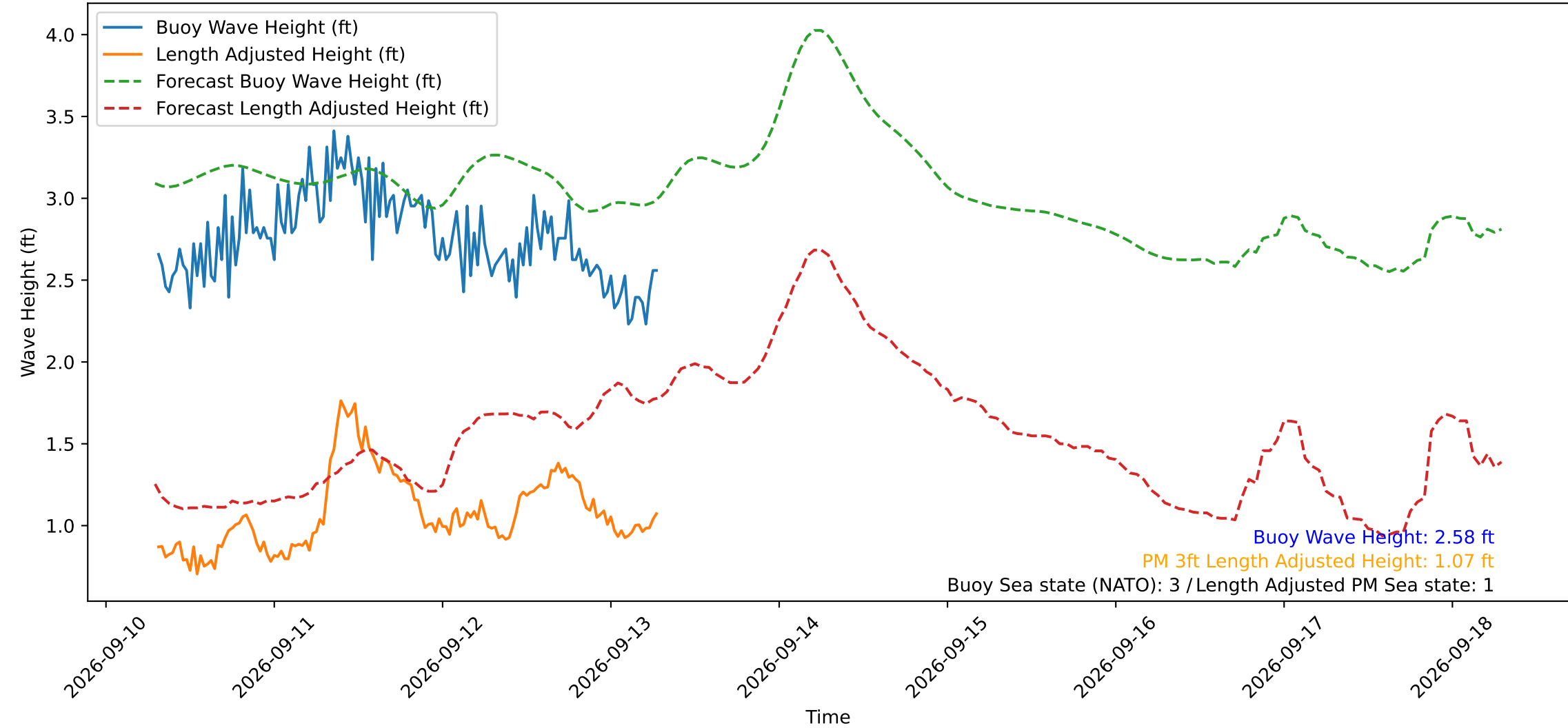
Wave Heights over Time for Red Beach at 2026-09-13 07:10:49
