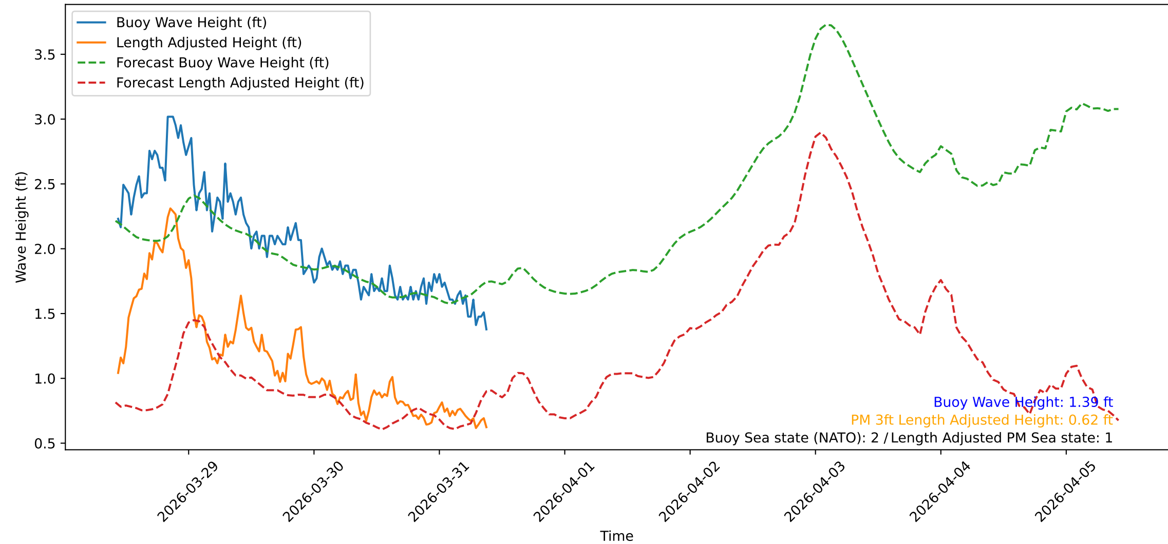
Wave Heights over Time for Red Beach at 2026-03-31 10:00:47
