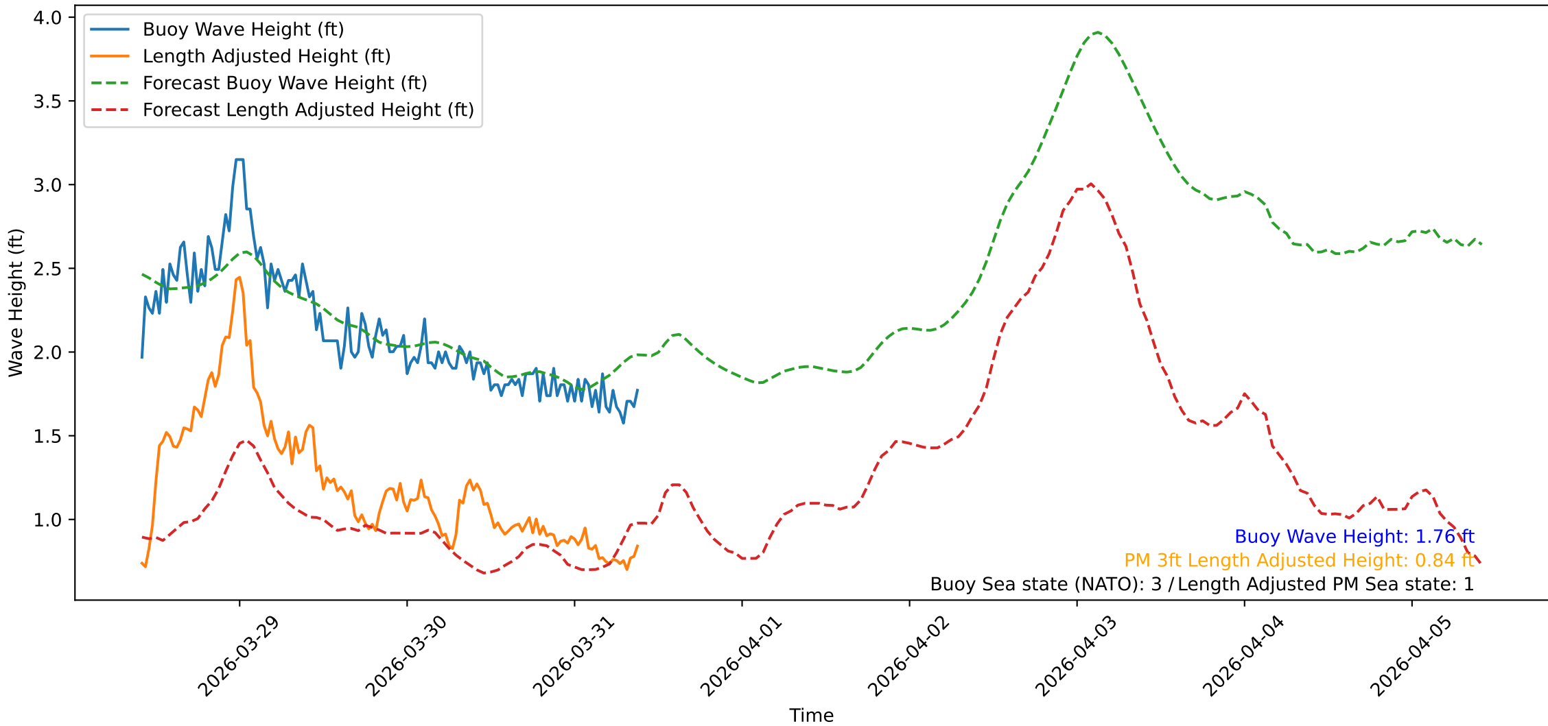
Wave Heights over Time for Oceanside Harbor at 2026-03-31 10:00:31
