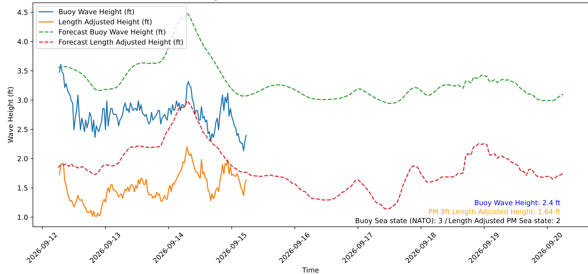
Wave Heights over Time for Green Beach at 2026-09-15 06:21:14
