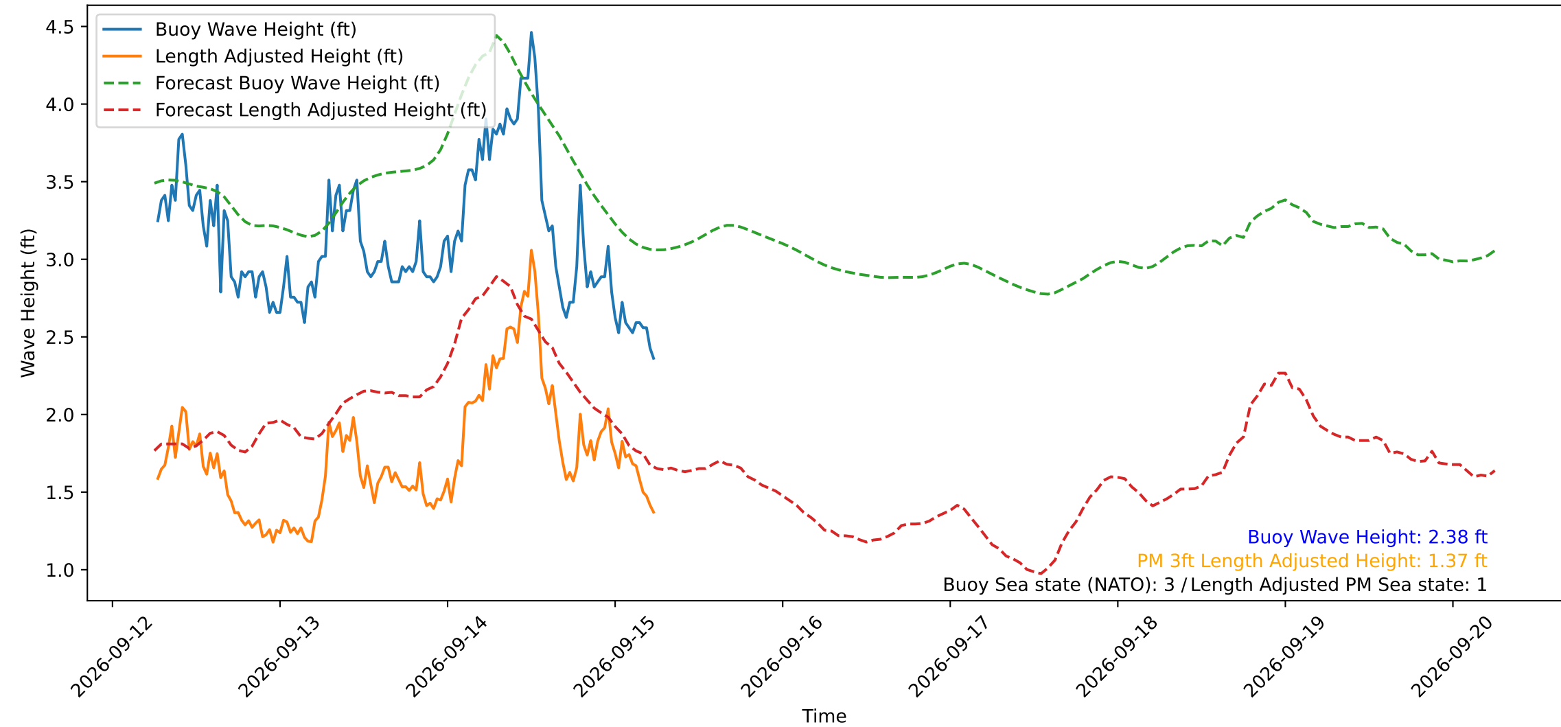
Wave Heights over Time for Oceanside Harbor at 2026-09-15 06:20:29
