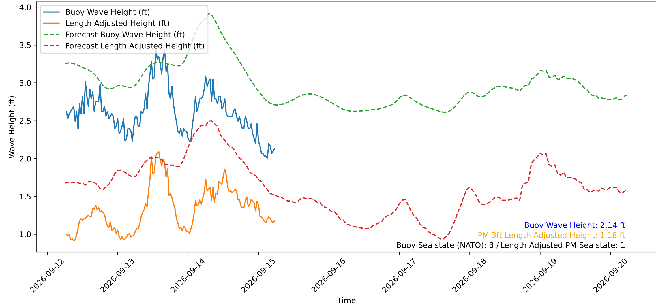
Wave Heights over Time for Red Beach at 2026-09-15 06:20:50
