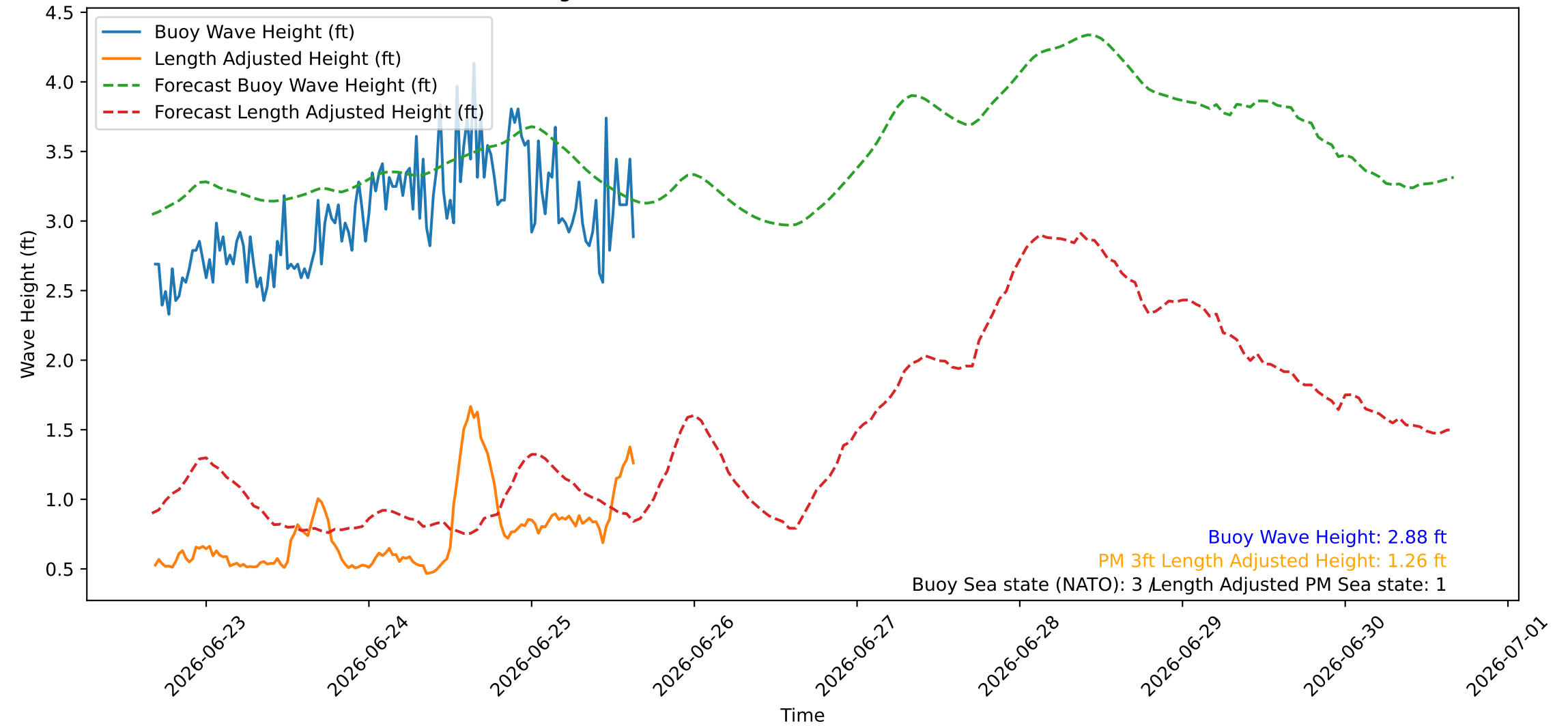
Wave Heights over Time for Red Beach at 2026-06-25 16:00:45
