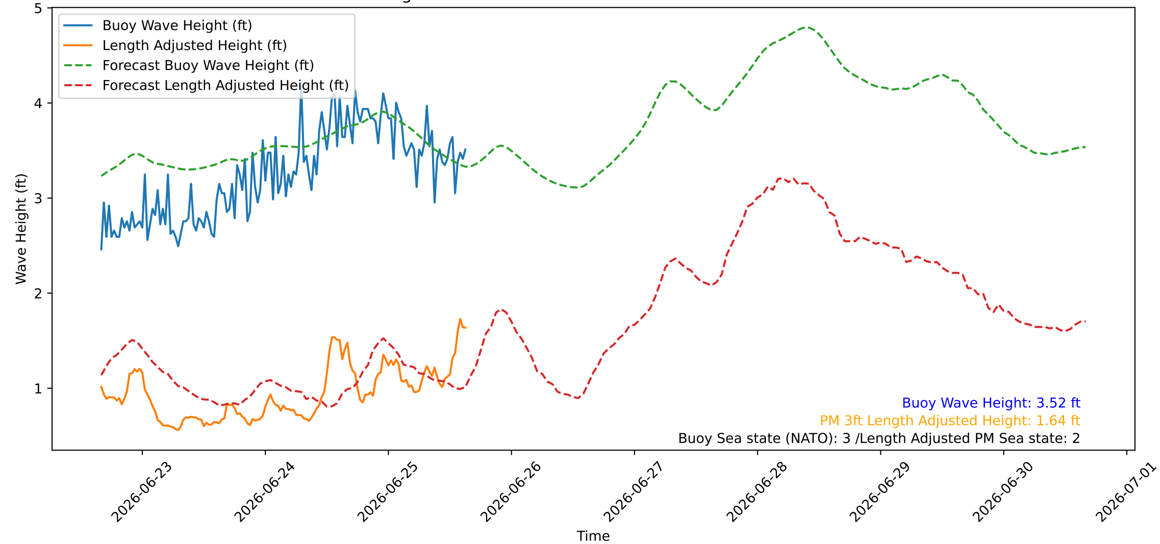
Wave Heights over Time for Green Beach at 2026-06-25 16:01:08
