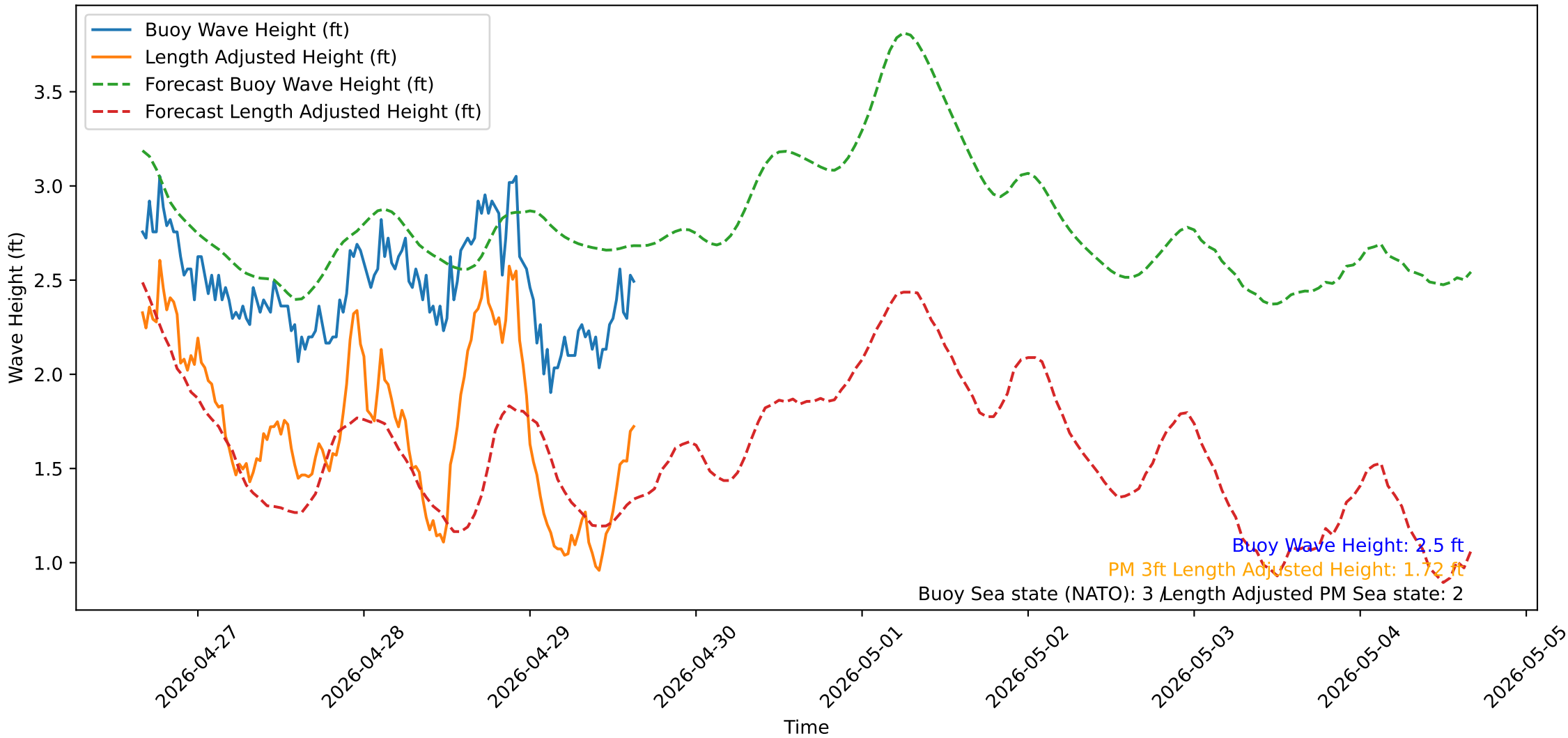
Wave Heights over Time for Oceanside Harbor at 2026-04-29 15:50:31
