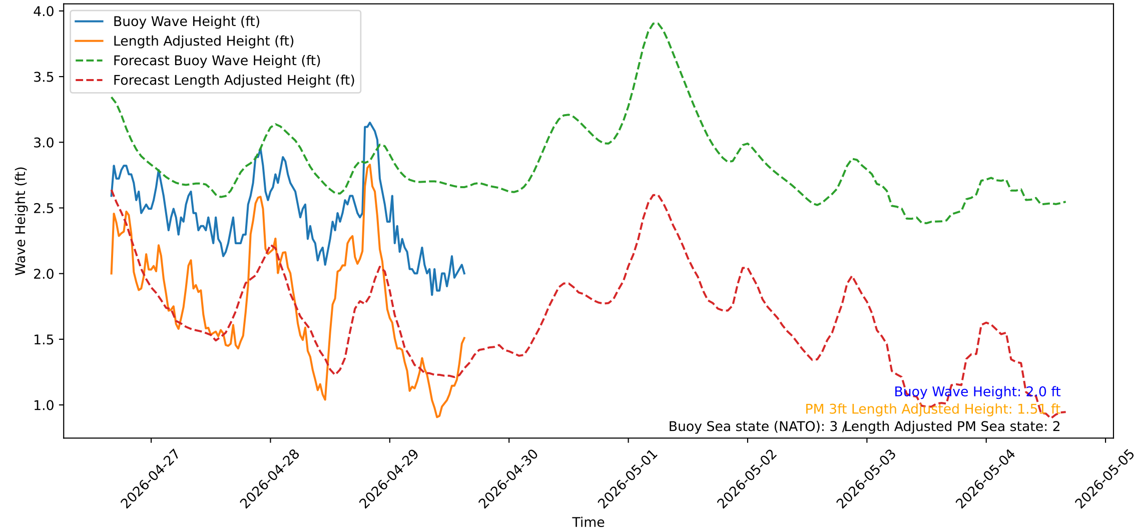
Wave Heights over Time for Green Beach at 2026-04-29 15:51:14
