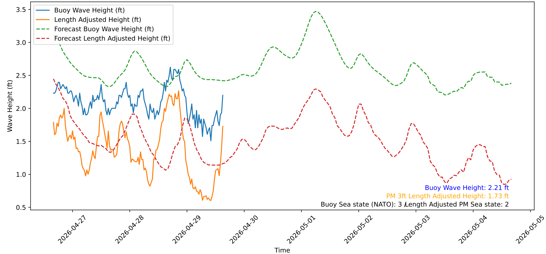
Wave Heights over Time for Red Beach at 2026-04-29 15:50:51
