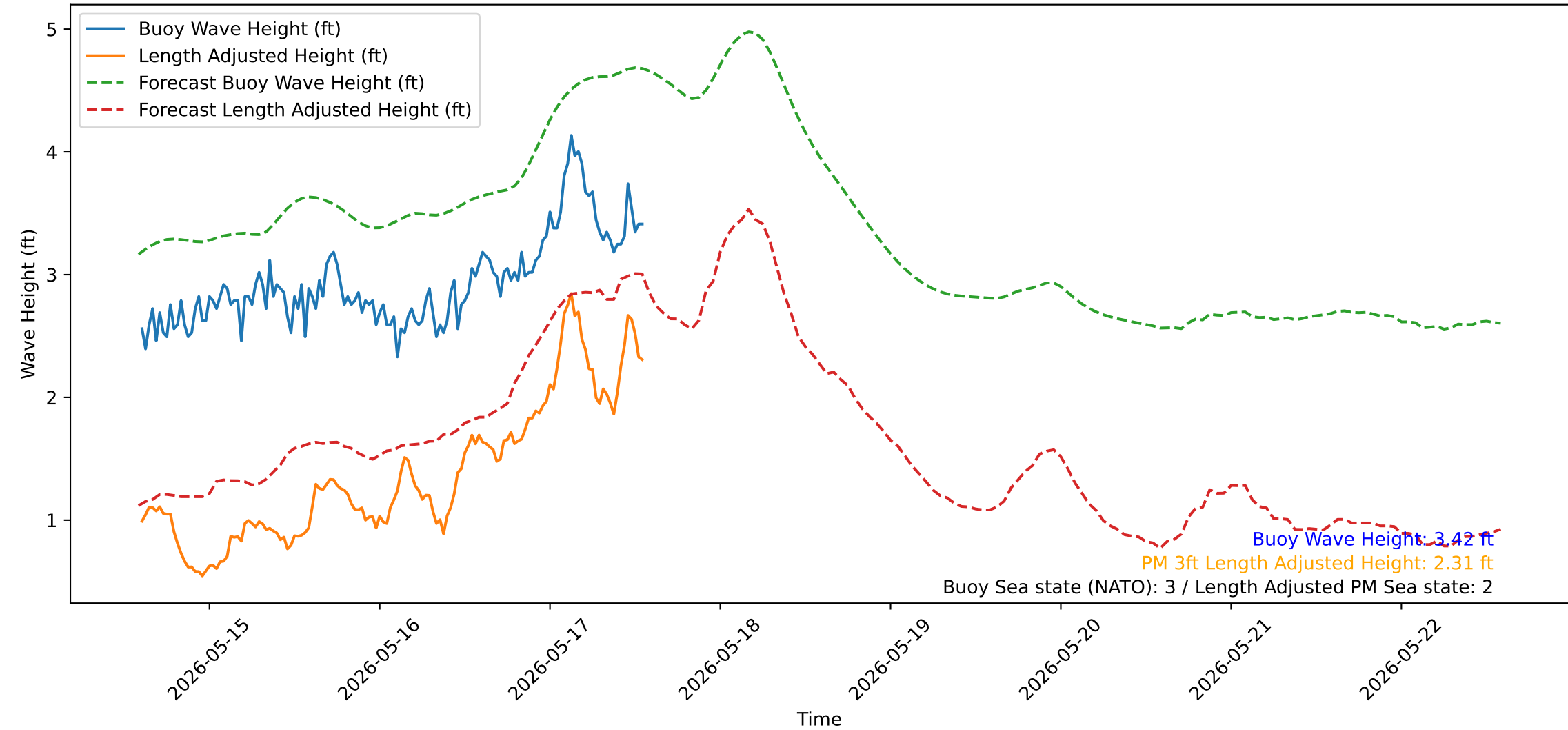
Wave Heights over Time for Red Beach at 2026-05-17 14:00:51
