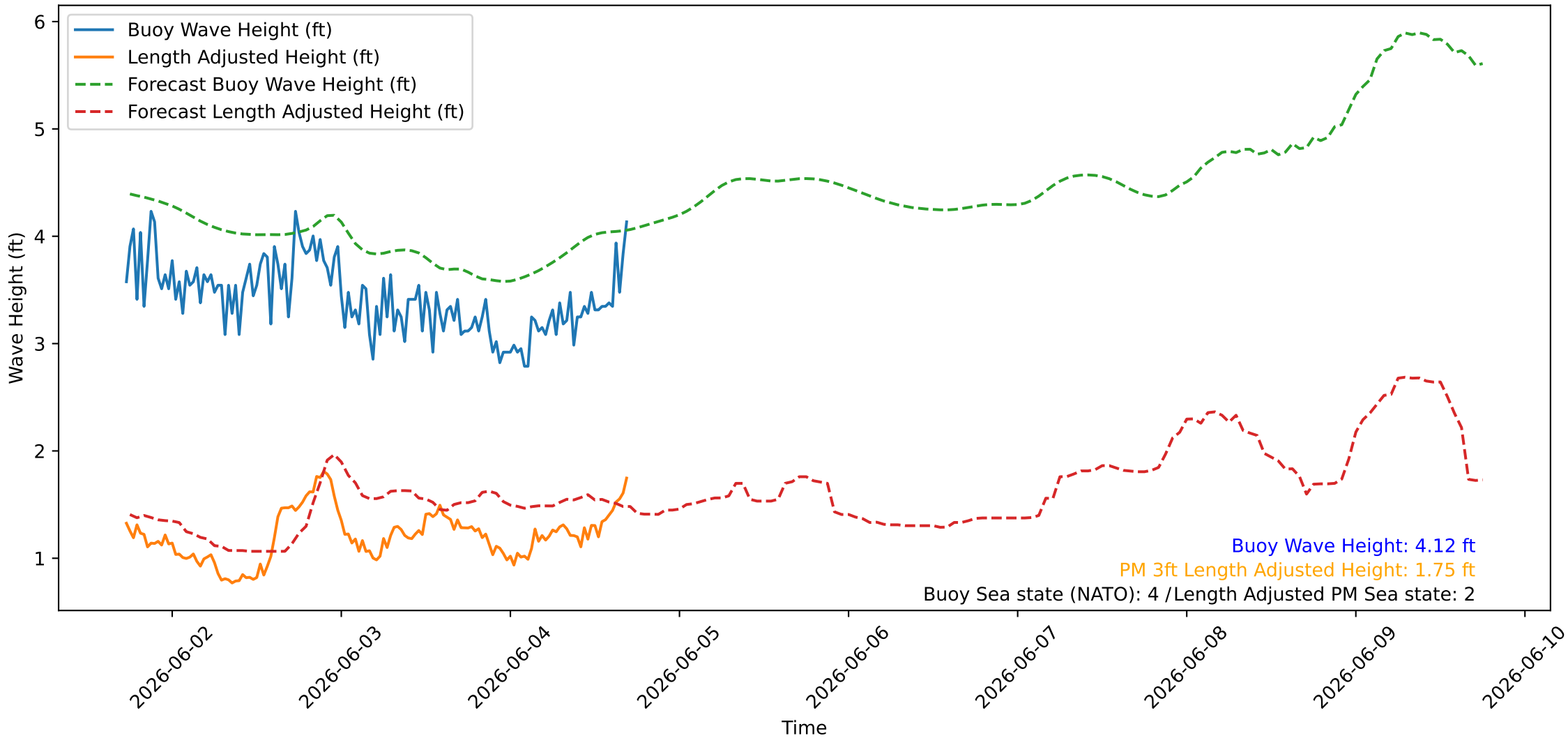
Wave Heights over Time for Green Beach at 2026-06-04 17:31:09
