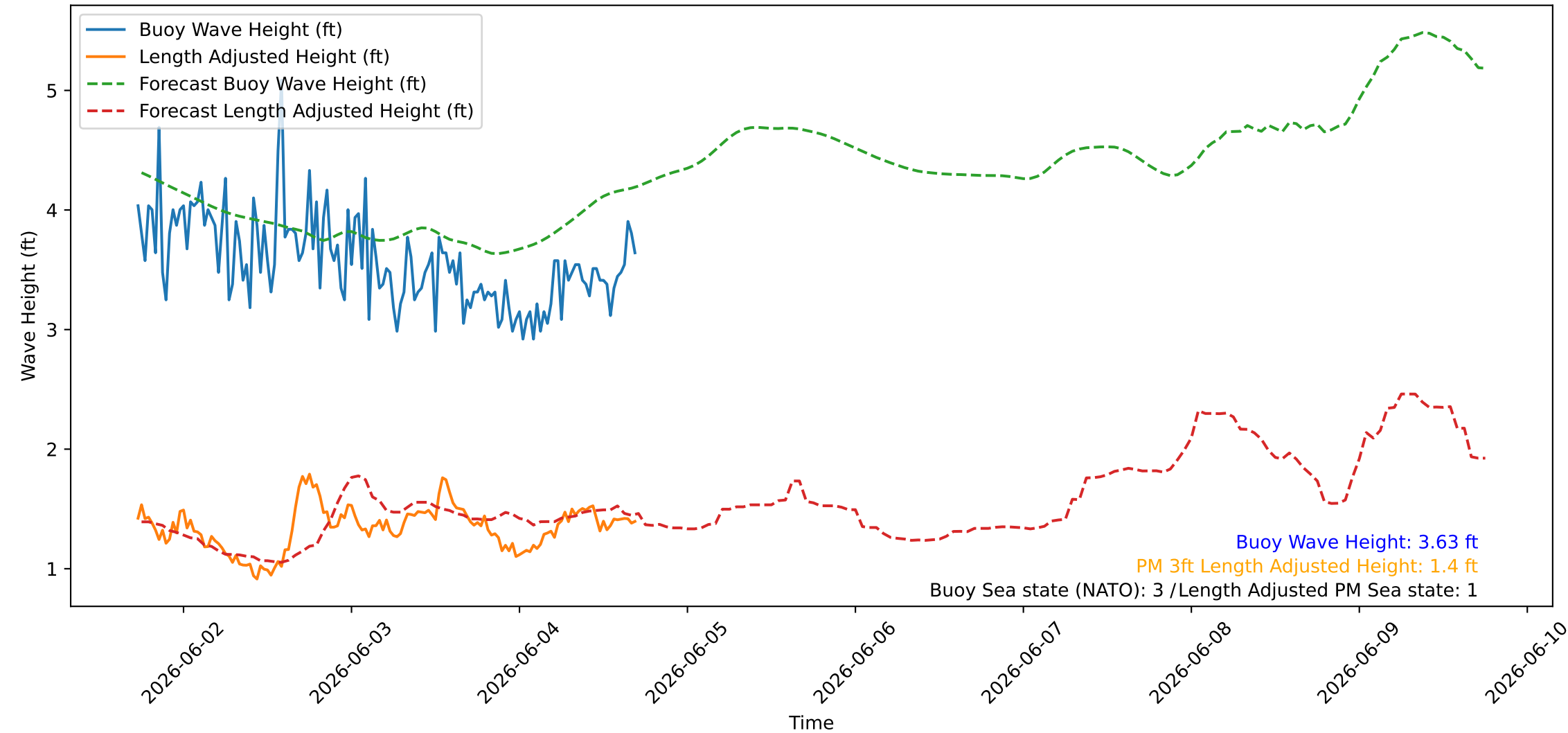
Wave Heights over Time for Oceanside Harbor at 2026-06-04 17:30:26
