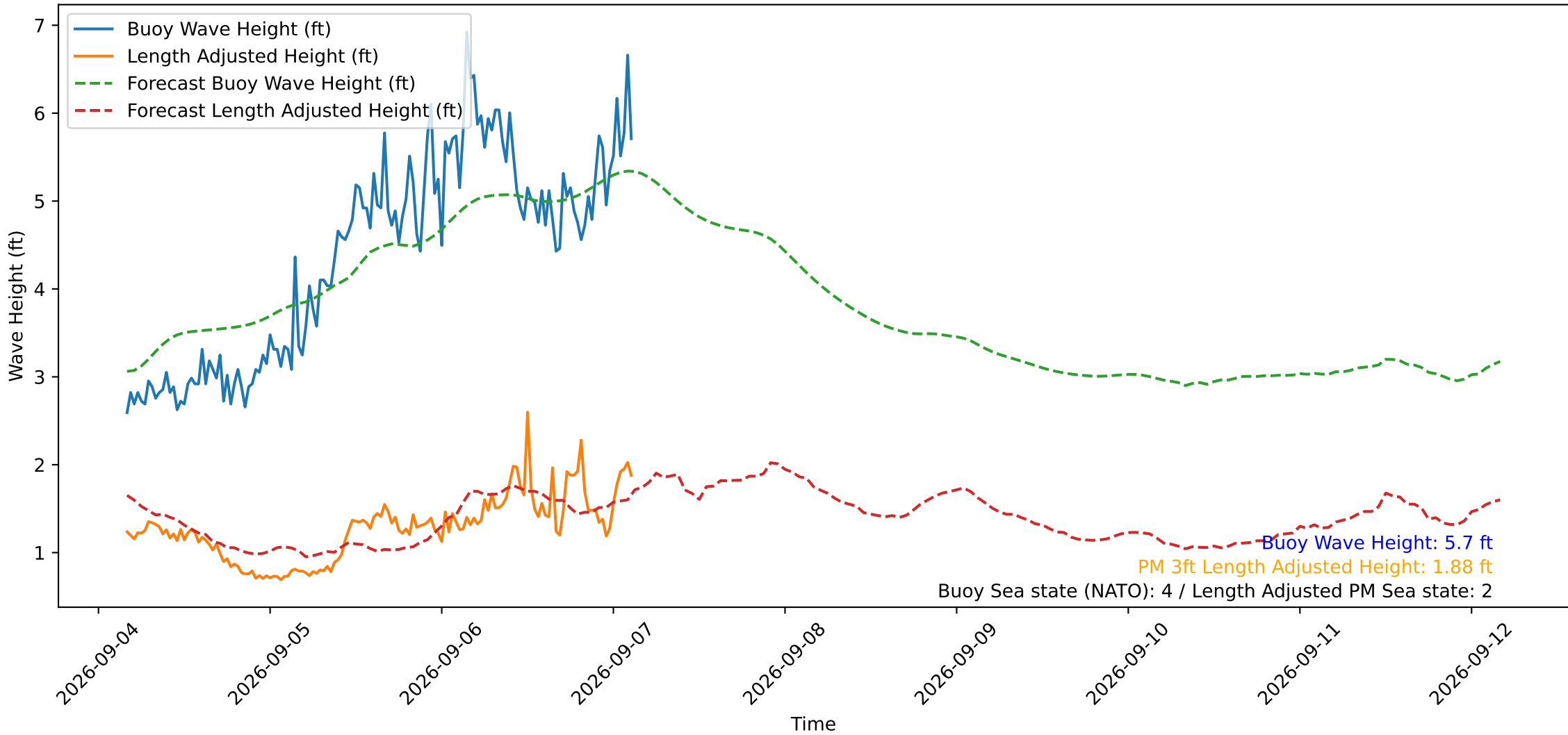
Wave Heights over Time for Red Beach at 2026-09-07 03:30:50
