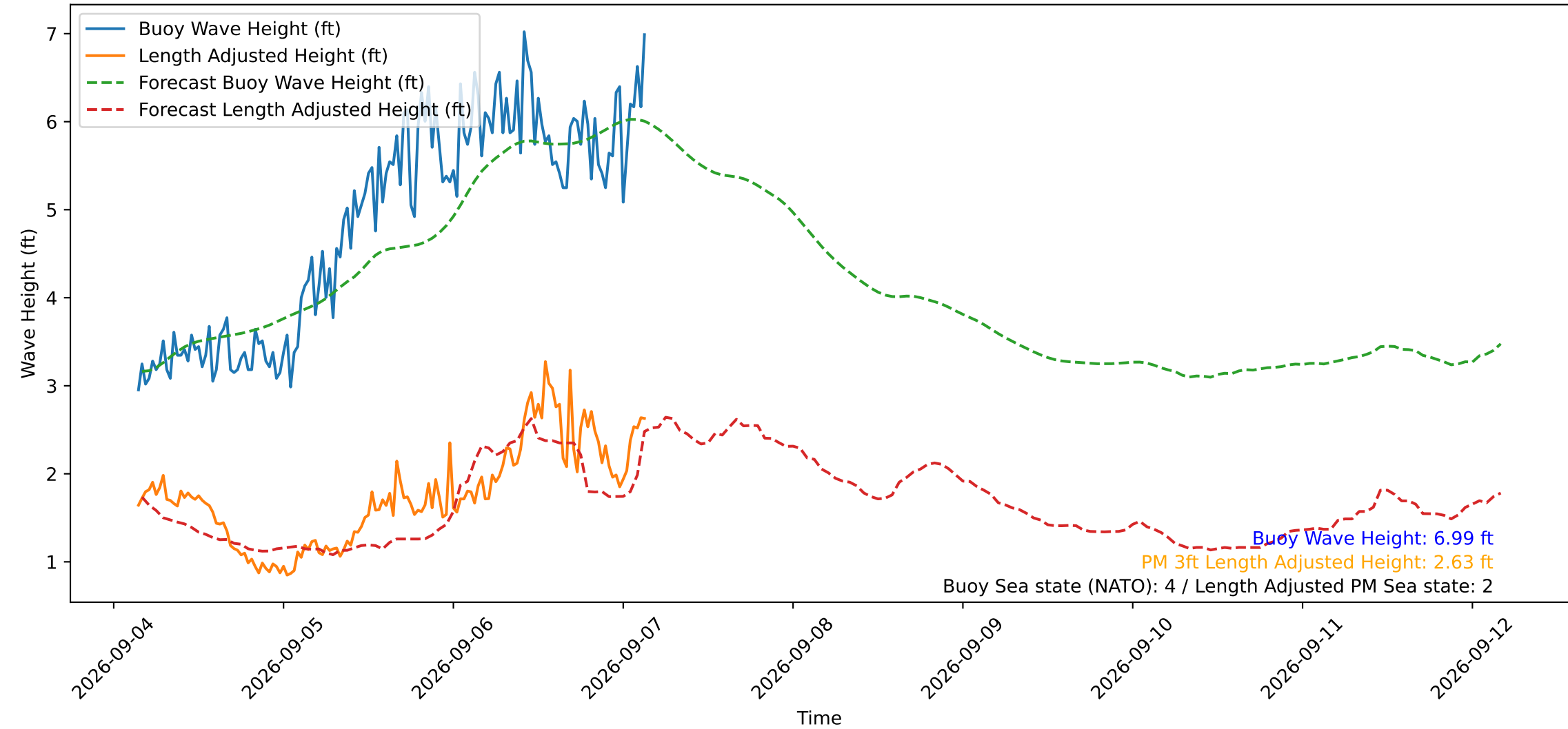
Wave Heights over Time for Oceanside Harbor at 2026-09-07 03:30:30
