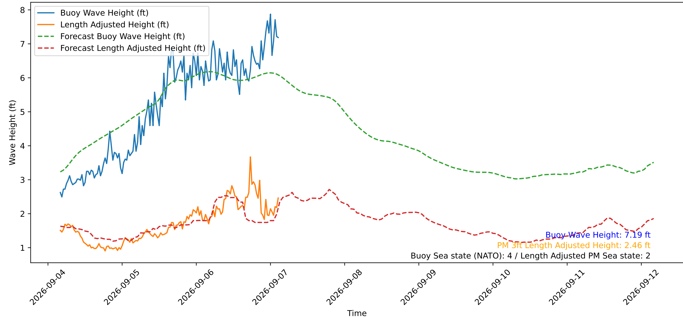
Wave Heights over Time for Green Beach at 2026-09-07 03:31:12
