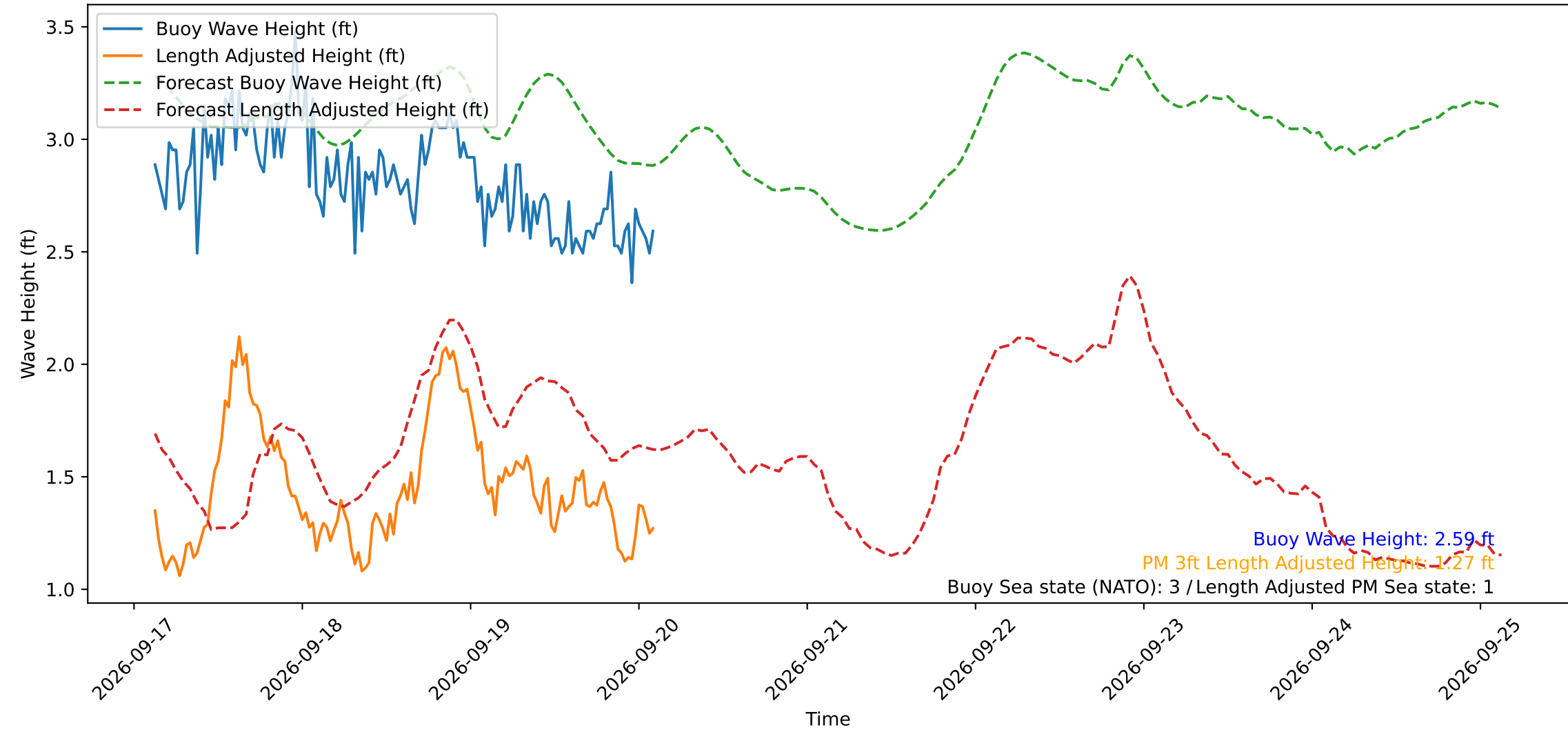
Wave Heights over Time for Green Beach at 2026-09-20 02:51:13
