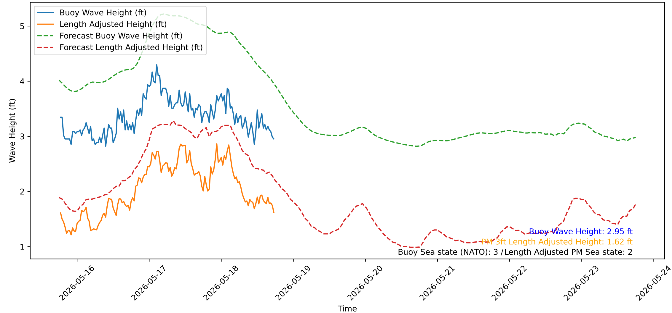
Wave Heights over Time for Oceanside Harbor at 2026-05-18 18:20:32
