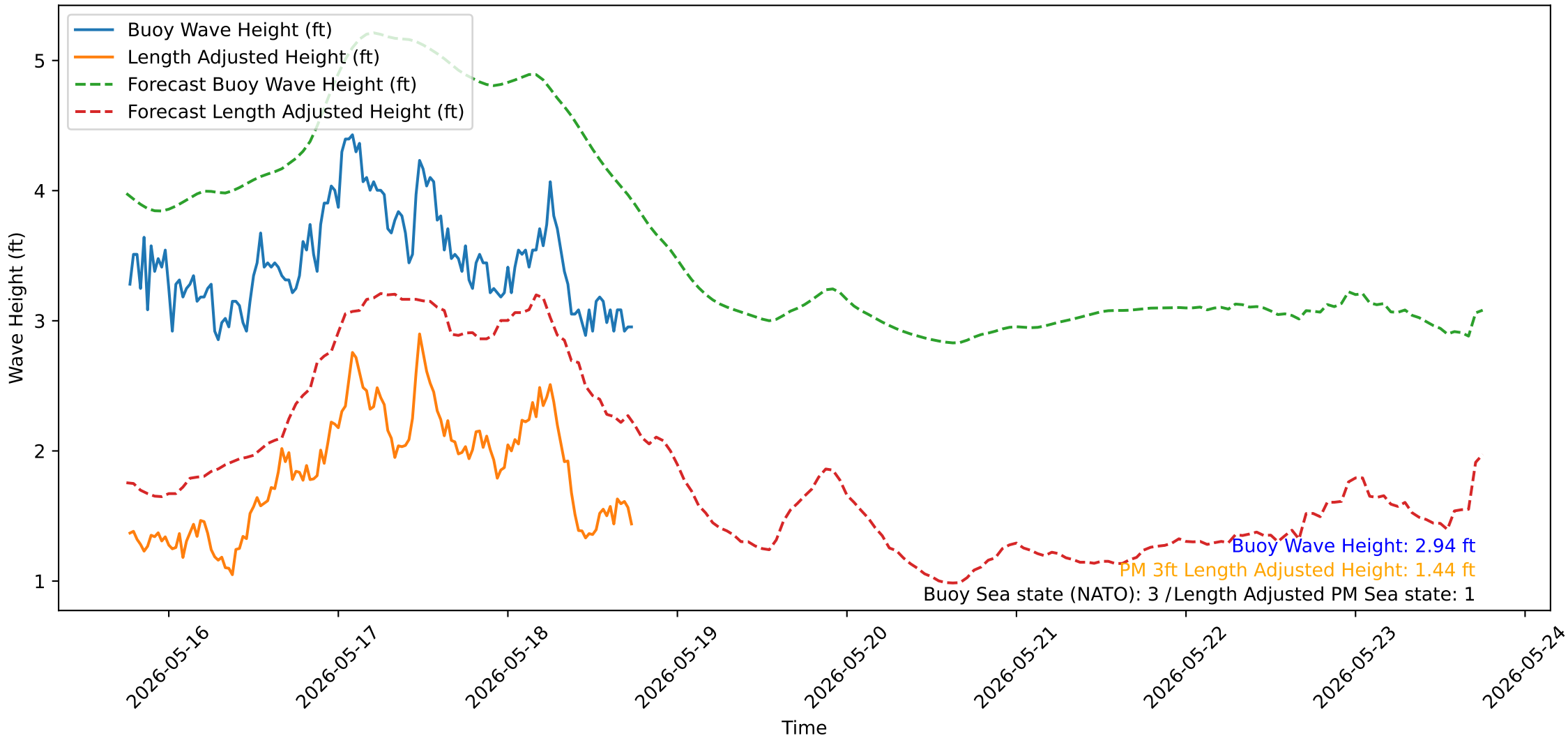
Wave Heights over Time for Green Beach at 2026-05-18 18:21:15
