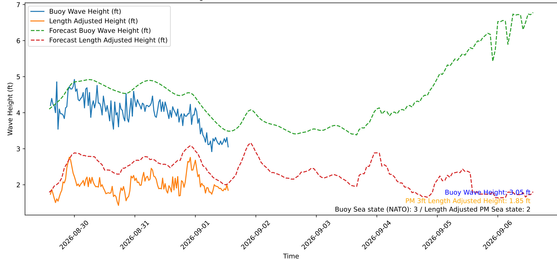
Wave Heights over Time for Green Beach at 2026-09-01 14:01:12
