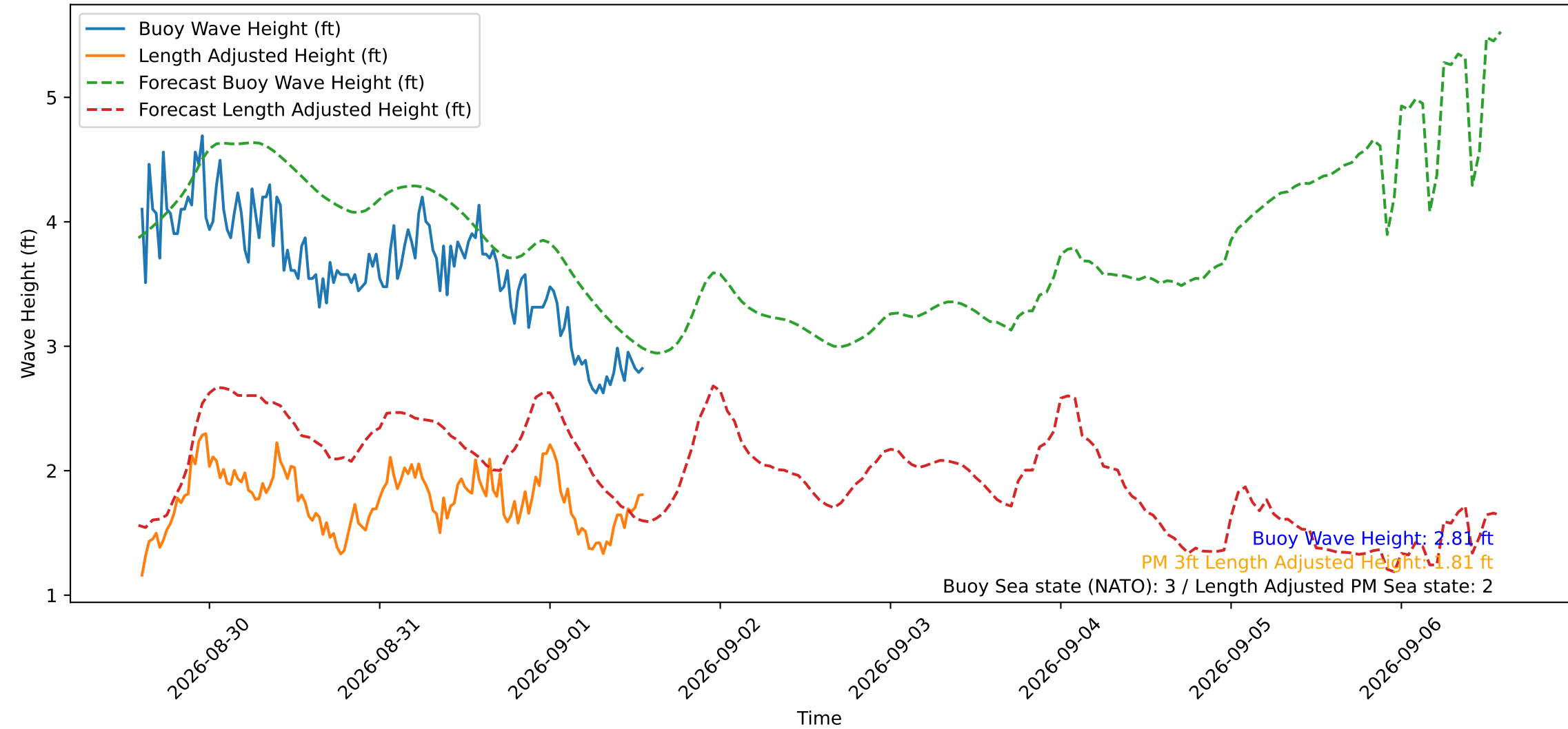
Wave Heights over Time for Red Beach at 2026-09-01 14:00:50
