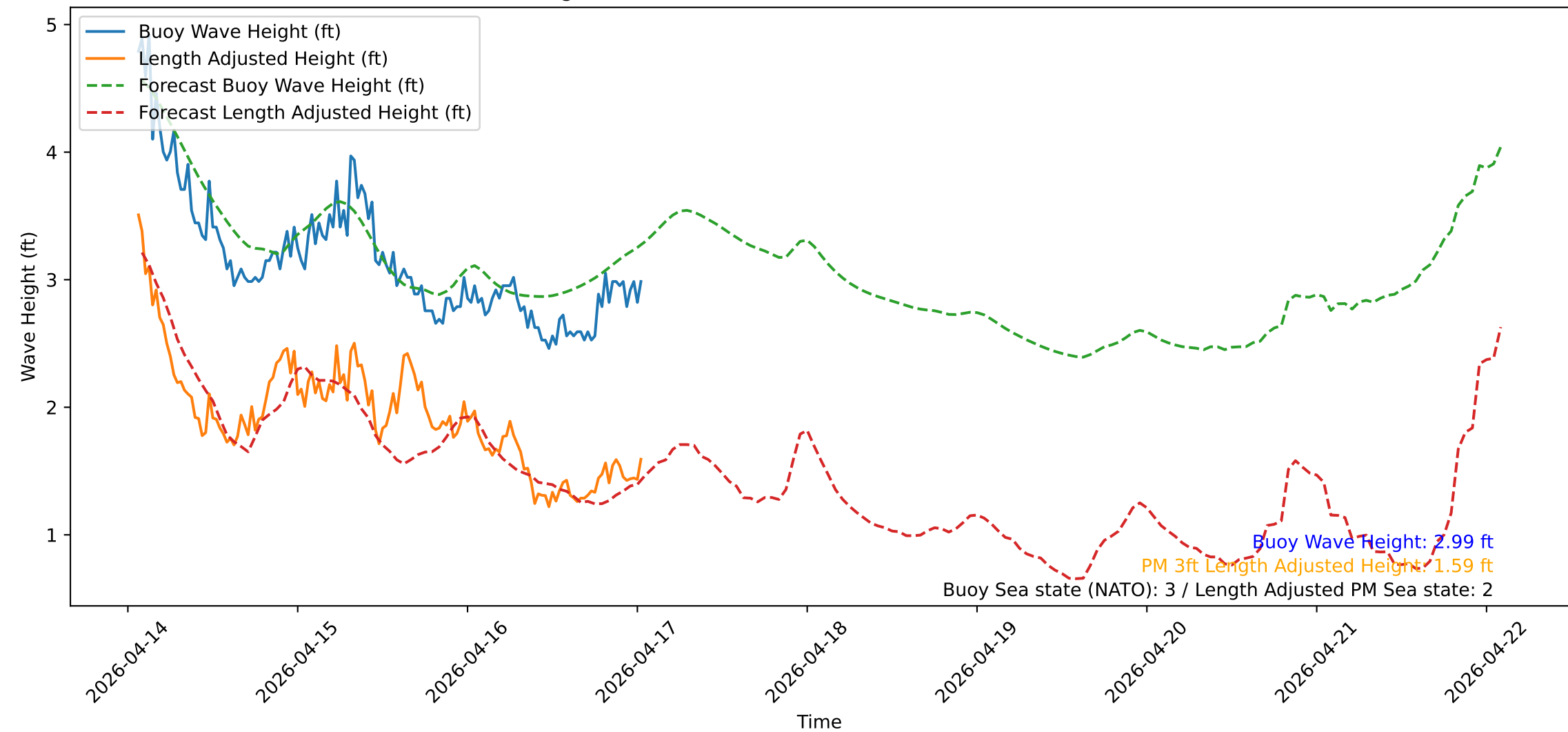
Wave Heights over Time for Green Beach at 2026-04-17 01:31:13
