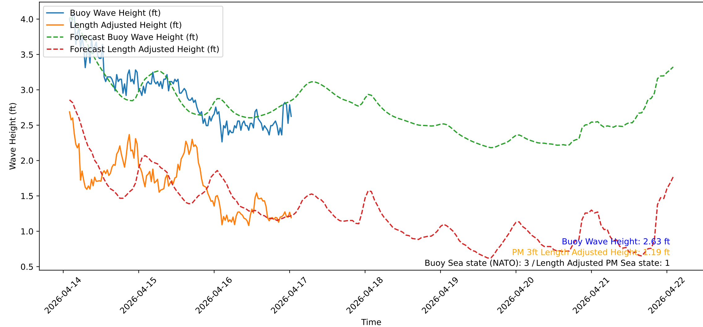
Wave Heights over Time for Red Beach at 2026-04-17 01:30:50
