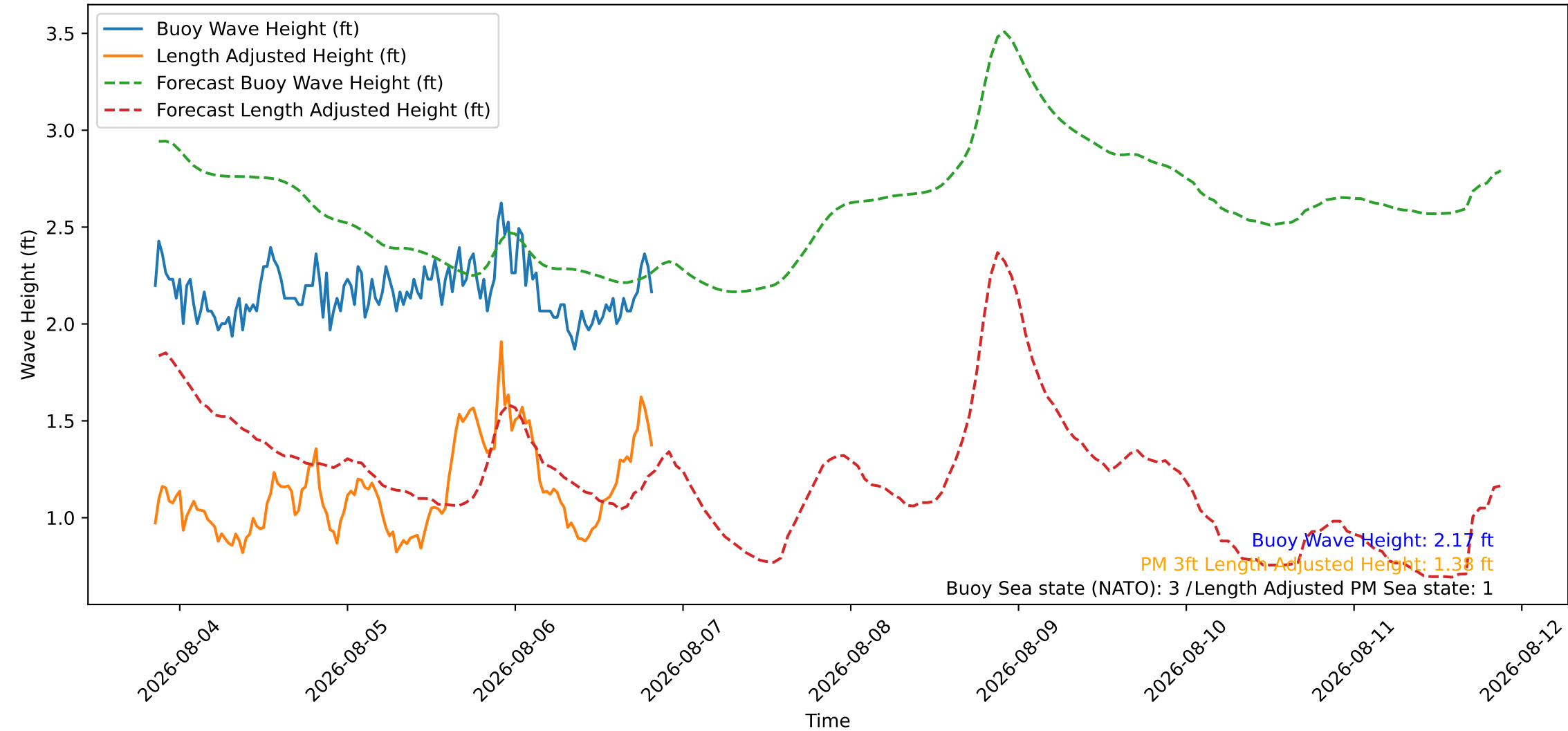
Wave Heights over Time for Green Beach at 2026-08-06 20:31:07
