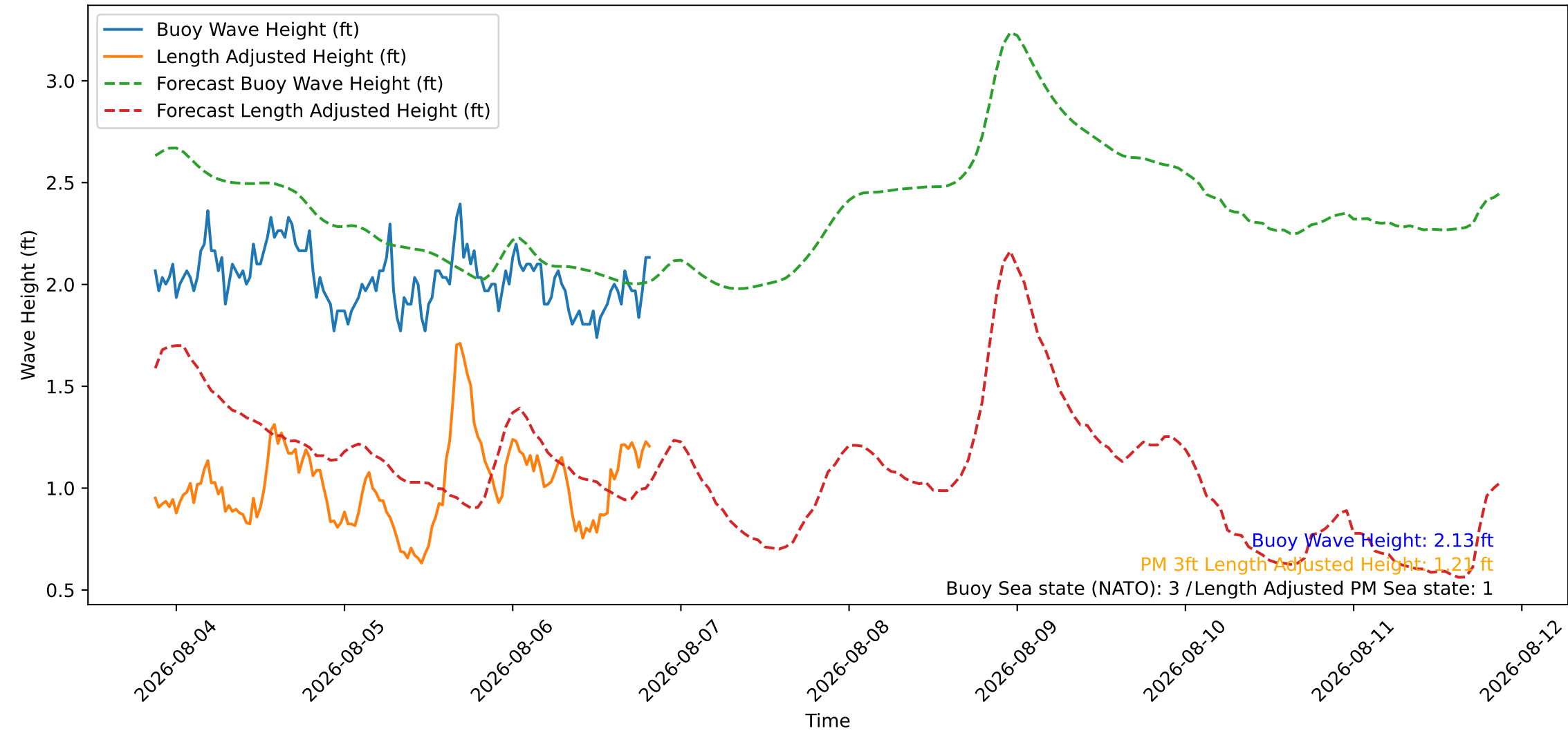
Wave Heights over Time for Red Beach at 2026-08-06 20:30:45
