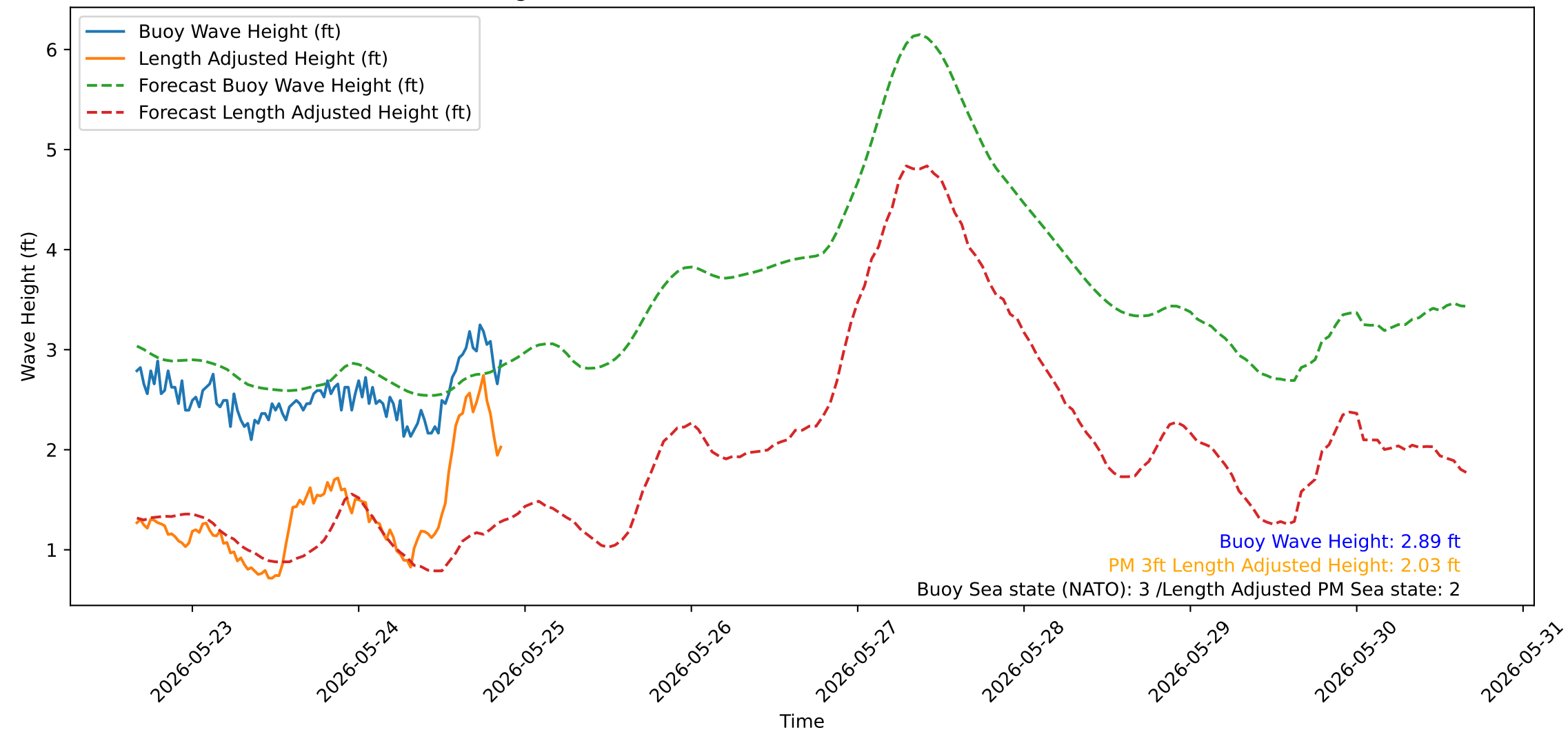
Wave Heights over Time for Oceanside Harbor at 2026-05-25 16:00:30
