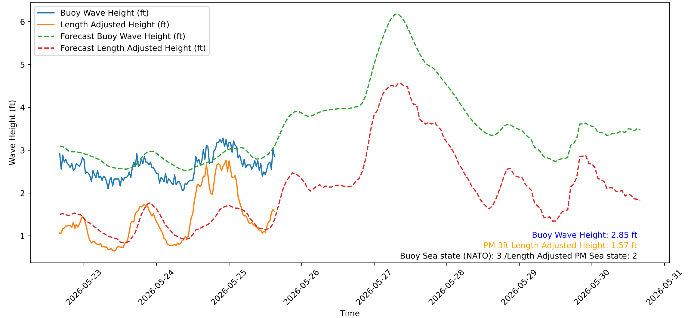
Wave Heights over Time for Green Beach at 2026-05-25 16:01:12
