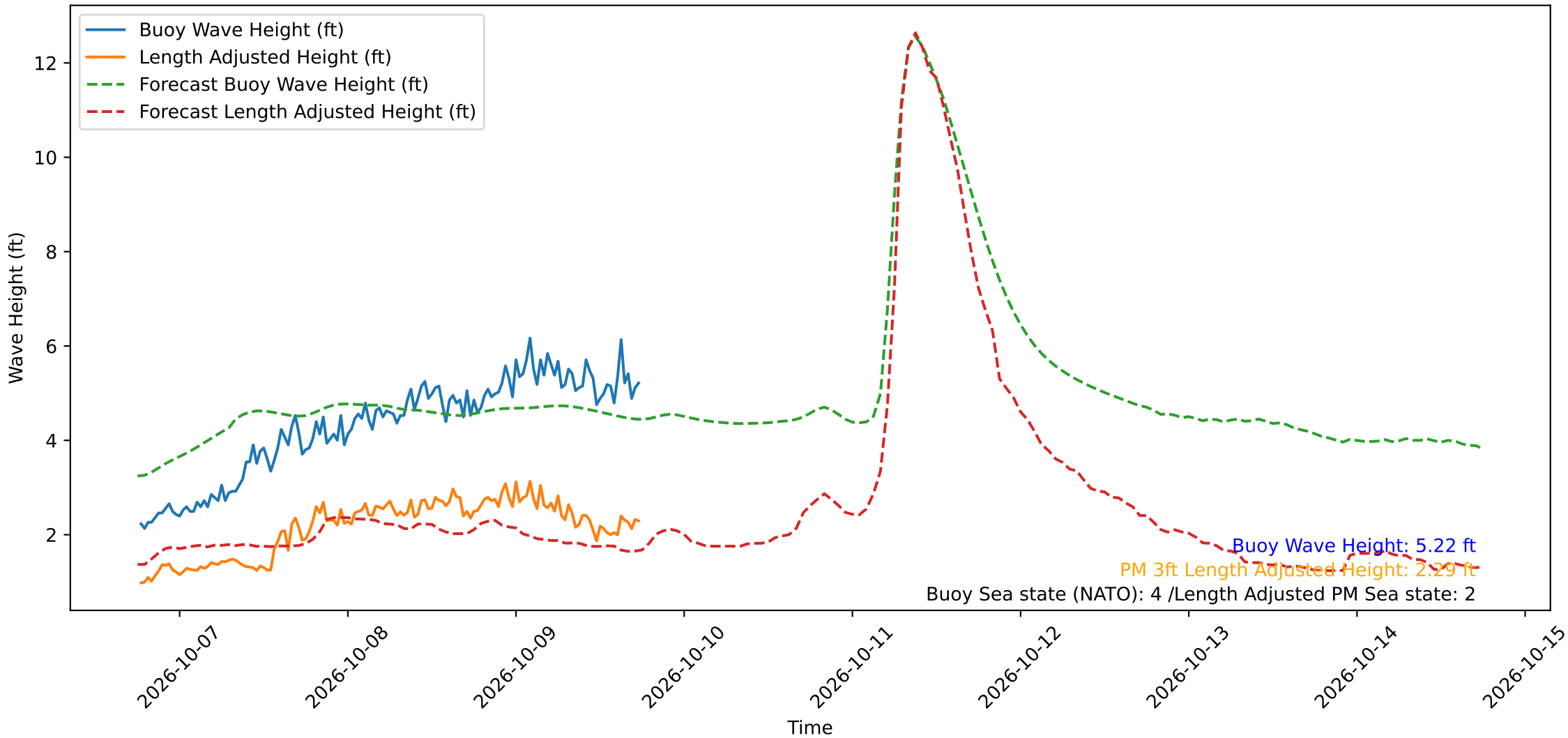
Wave Heights over Time for Green Beach at 2026-10-09 18:21:15
