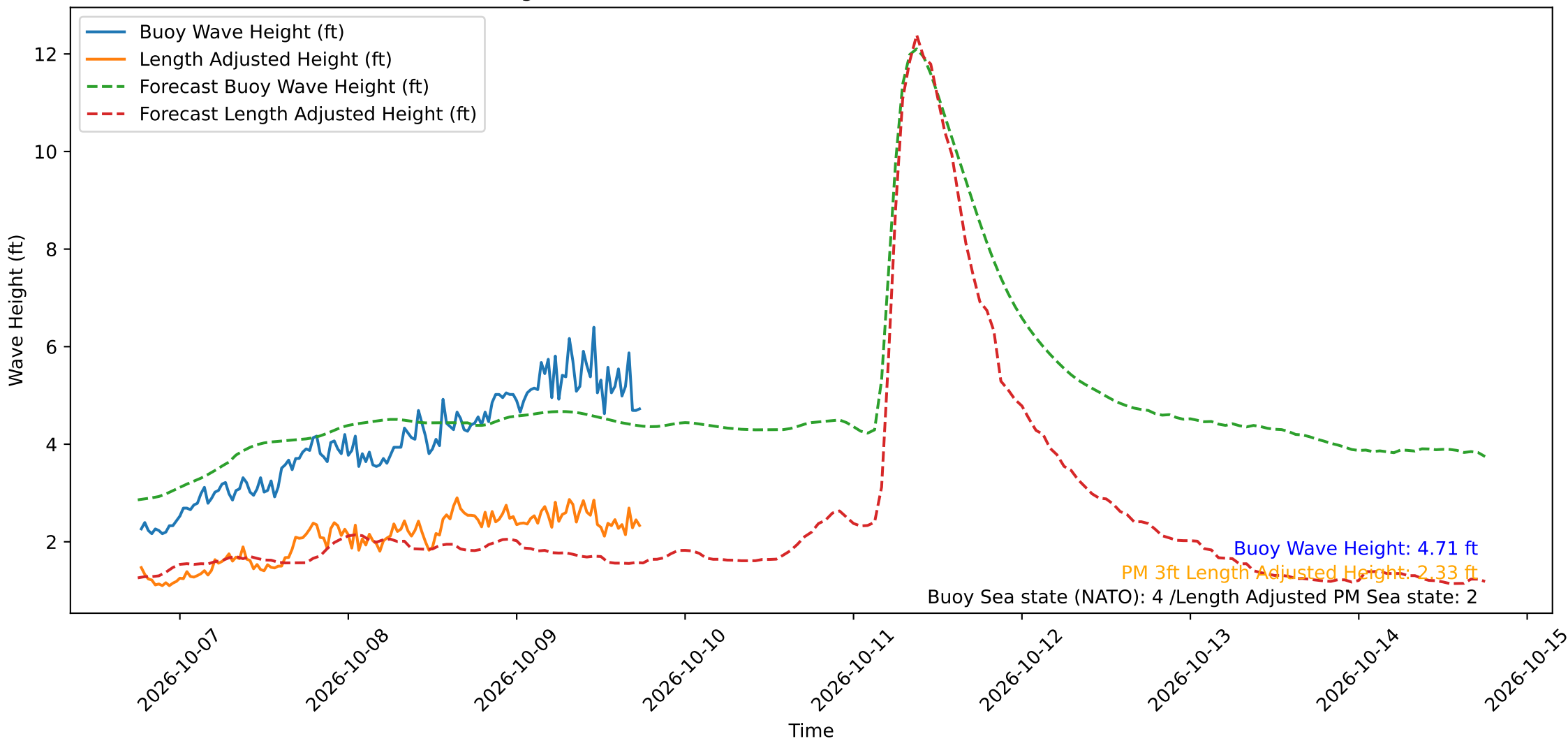
Wave Heights over Time for Oceanside Harbor at 2026-10-09 18:20:29
