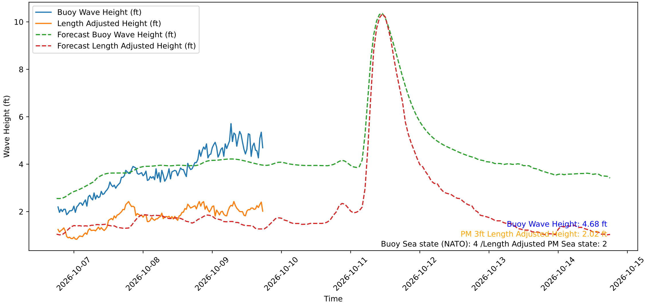
Wave Heights over Time for Red Beach at 2026-10-09 18:20:51
