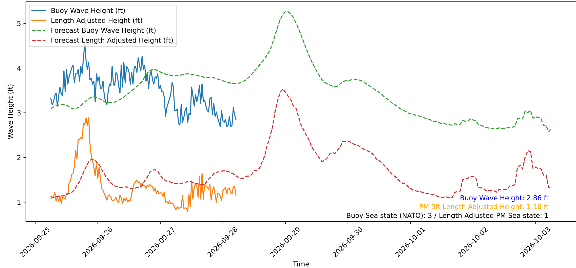
Wave Heights over Time for Green Beach at 2026-09-28 05:51:15
