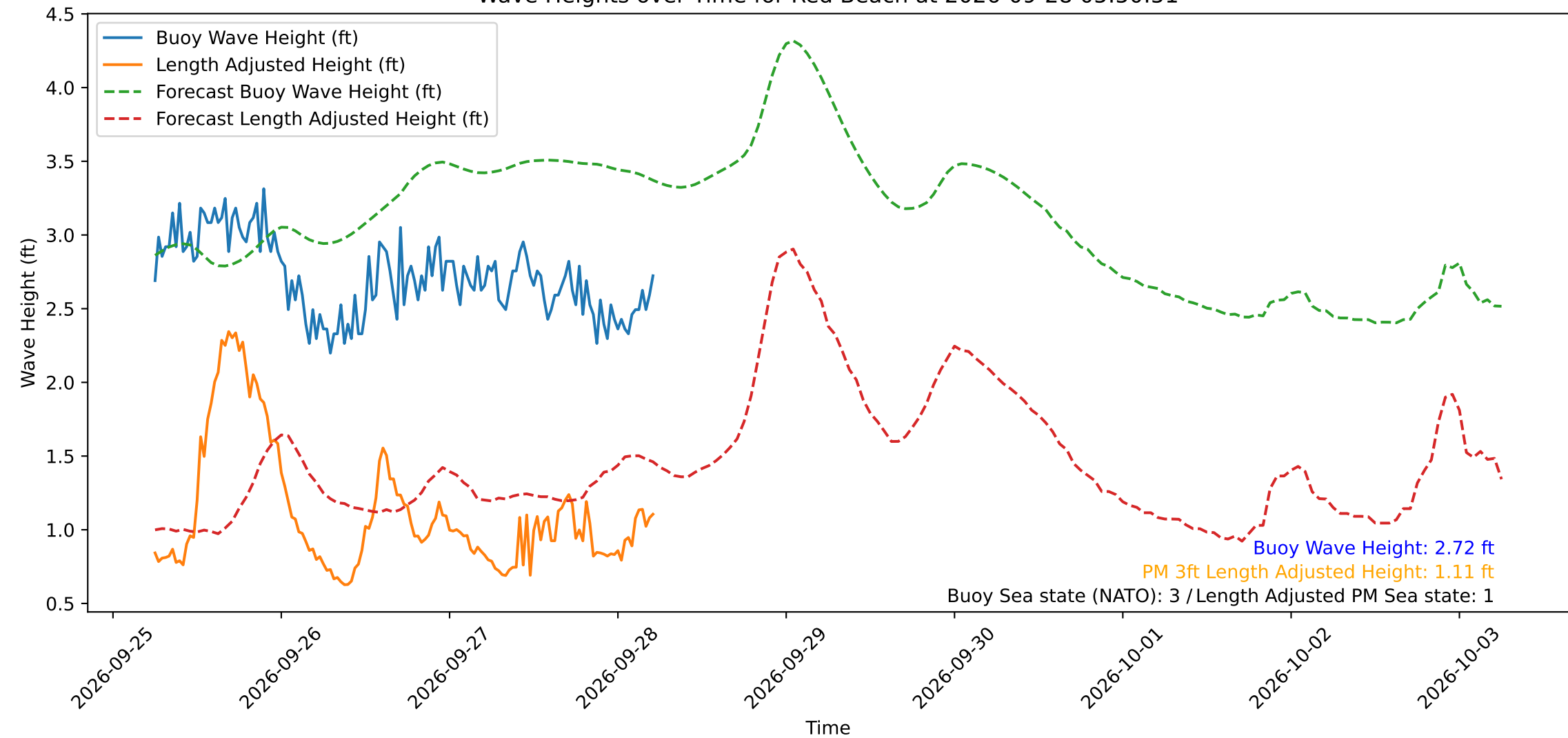
Wave Heights over Time for Red Beach at 2026-09-28 05:50:51
