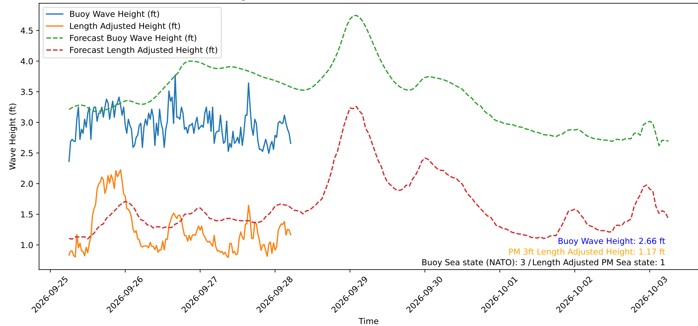
Wave Heights over Time for Oceanside Harbor at 2026-09-28 05:50:30
