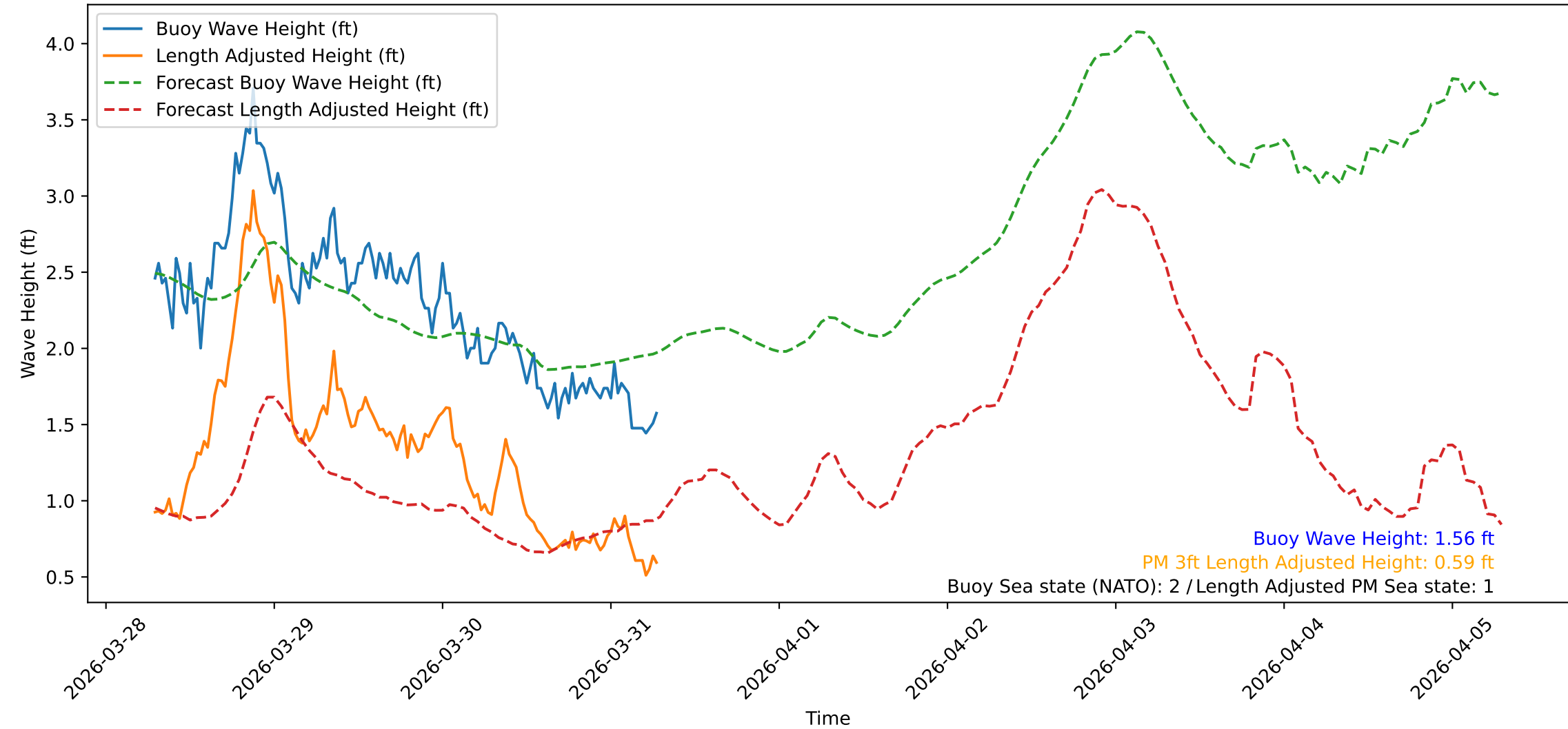
Wave Heights over Time for Green Beach at 2026-03-31 07:11:10
