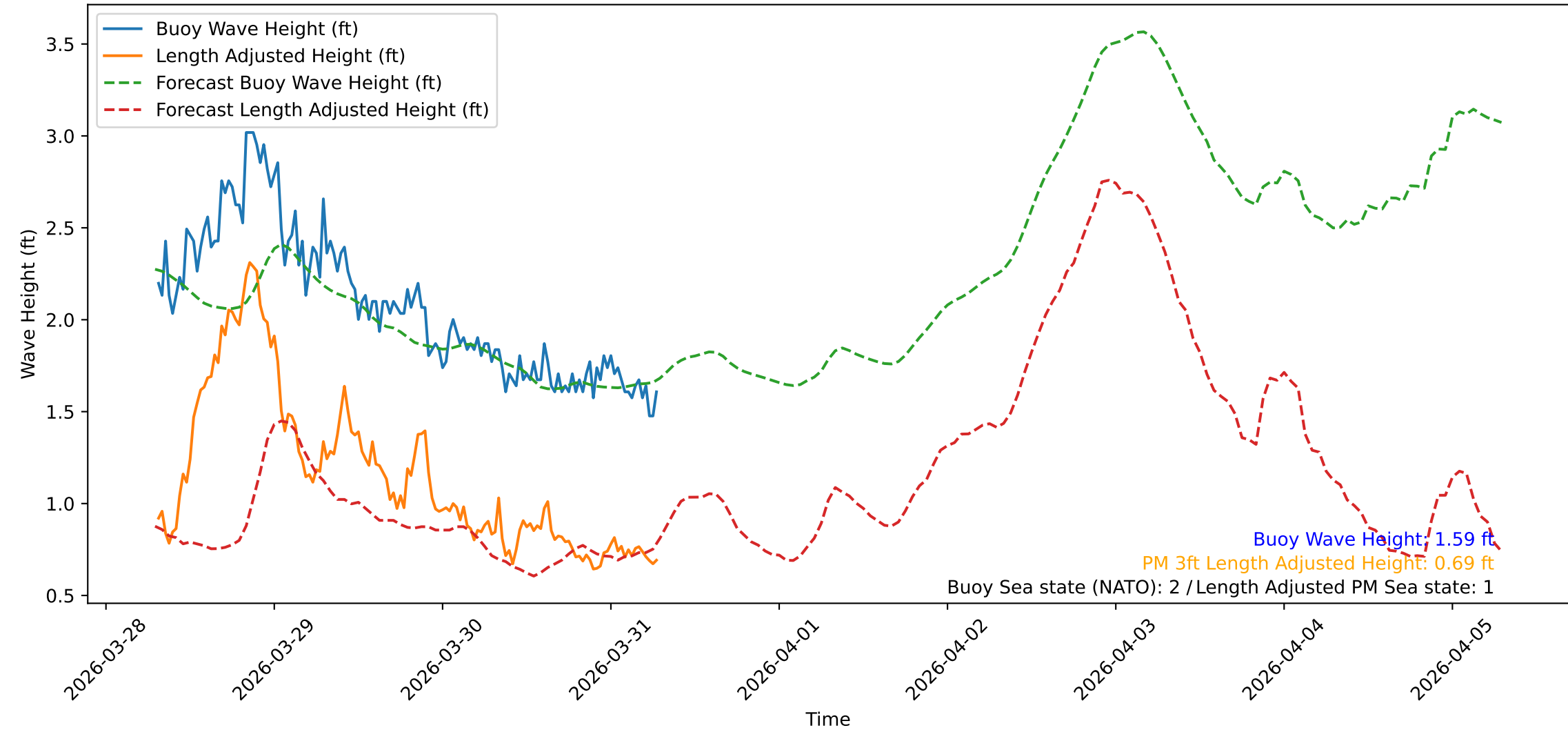
Wave Heights over Time for Red Beach at 2026-03-31 07:10:48
