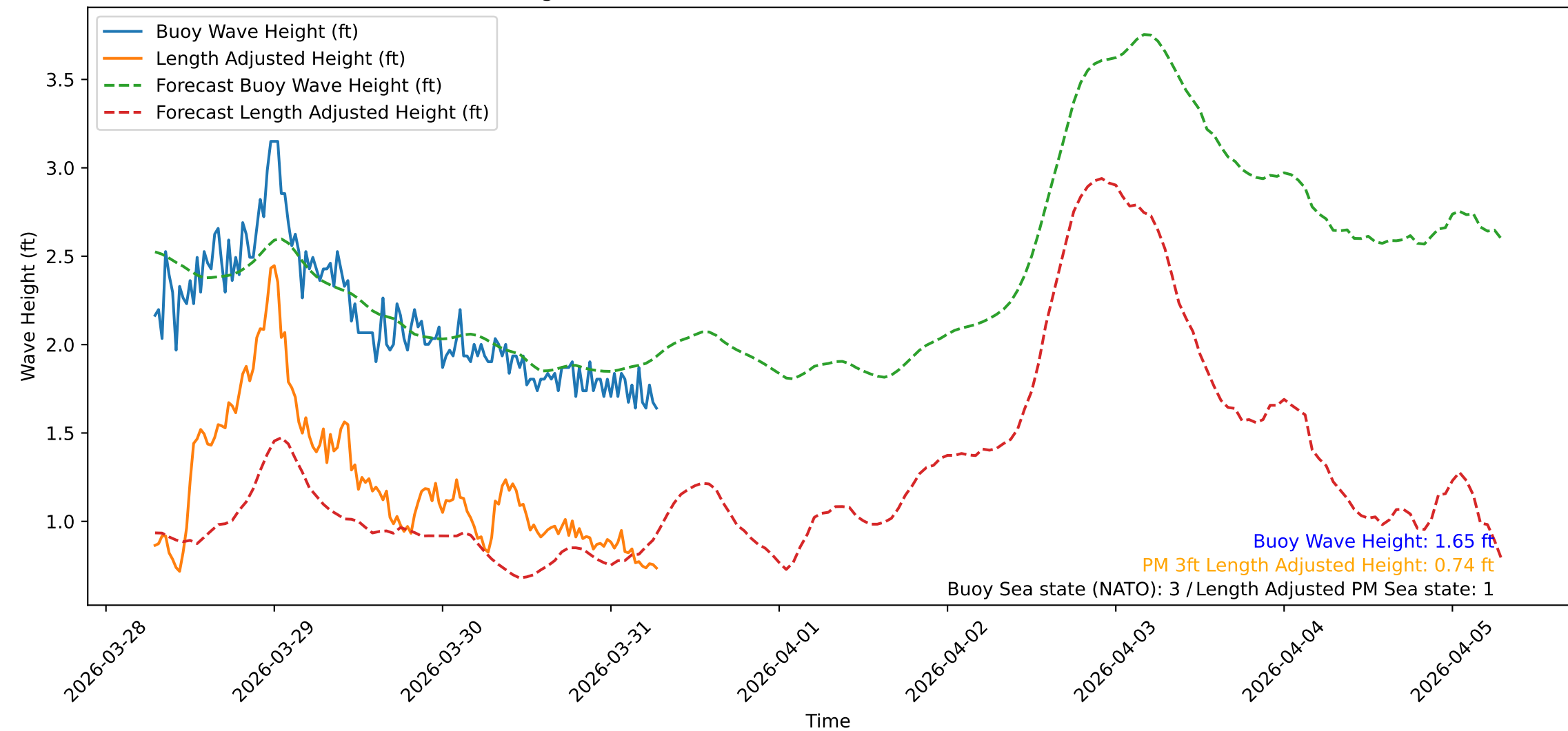
Wave Heights over Time for Oceanside Harbor at 2026-03-31 07:10:32
