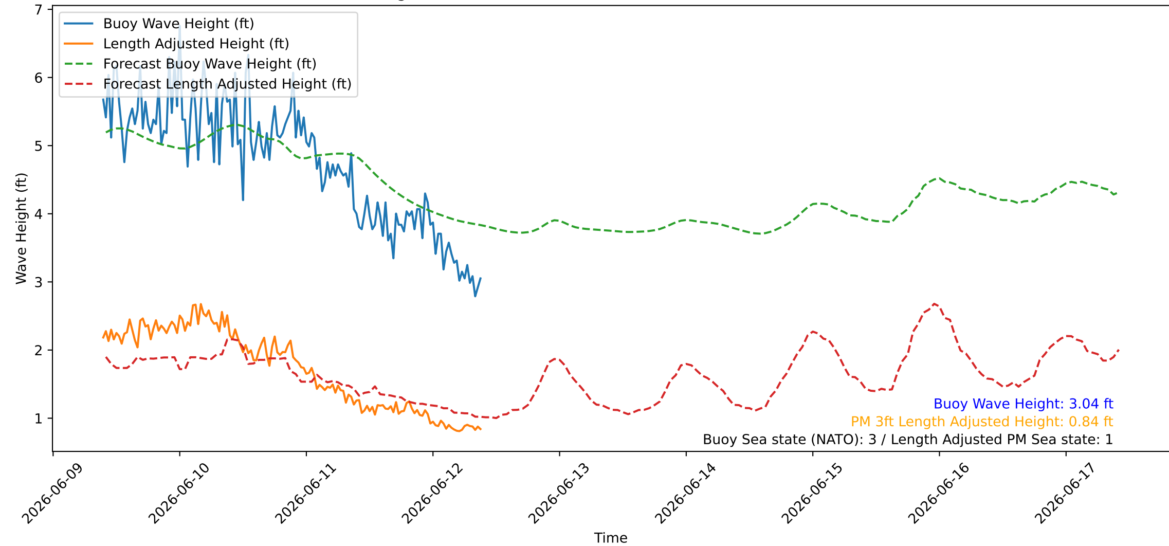
Wave Heights over Time for Oceanside Harbor at 2026-06-12 09:40:26
