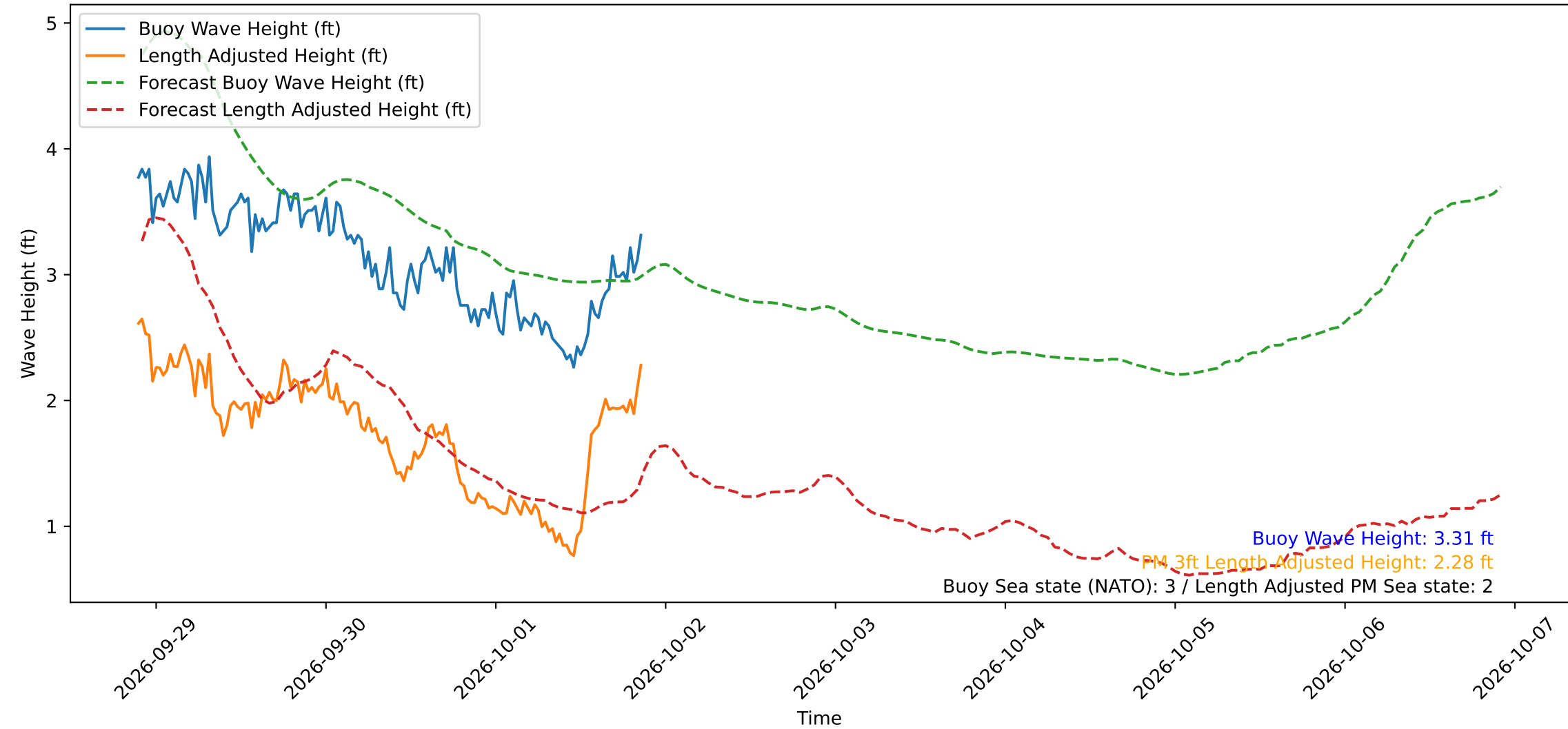
Wave Heights over Time for Oceanside Harbor at 2026-10-01 21:30:29
