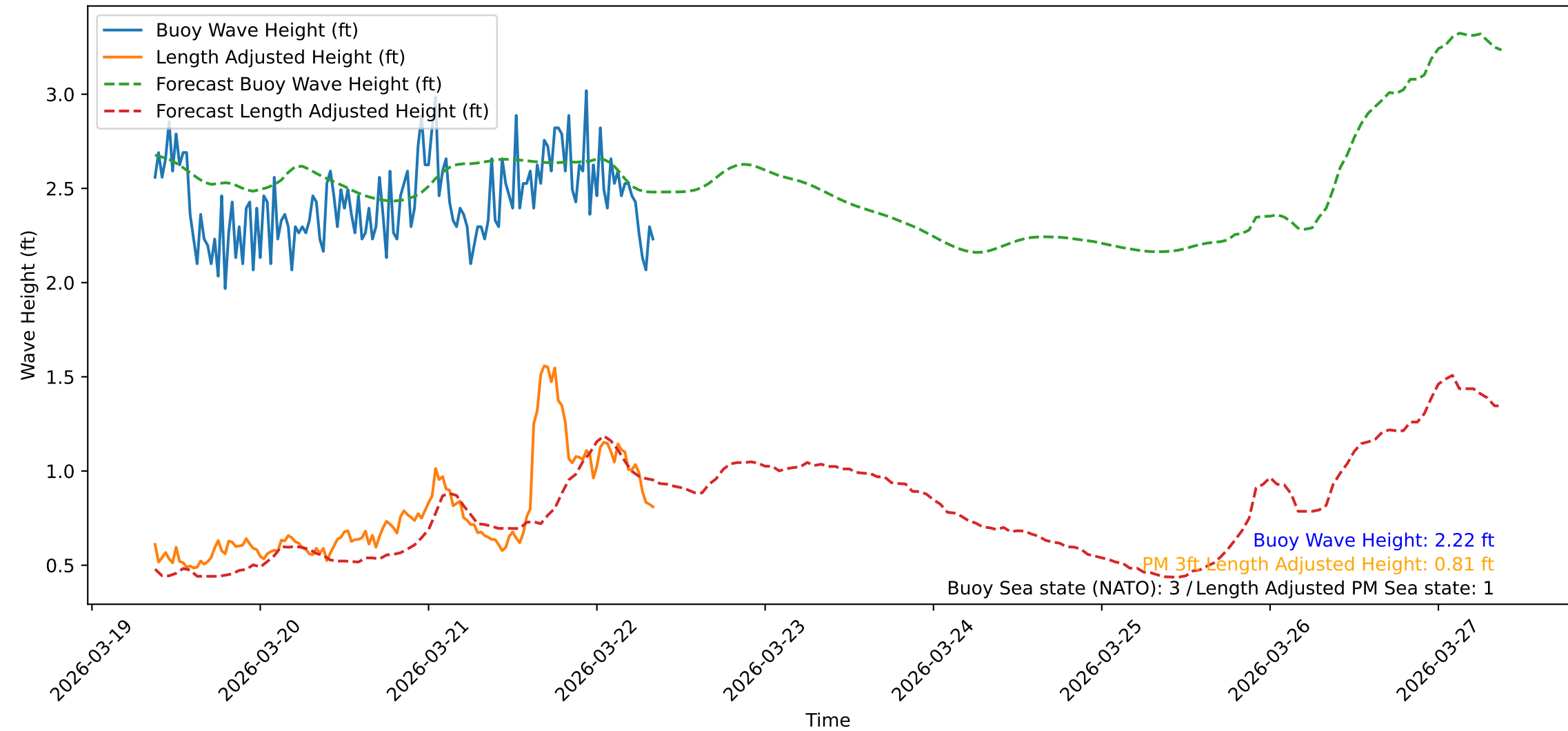
Wave Heights over Time for Oceanside Harbor at 2026-03-22 09:00:31
