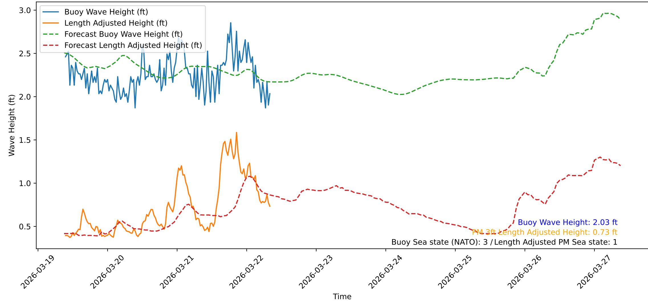
Wave Heights over Time for Red Beach at 2026-03-22 09:00:47
