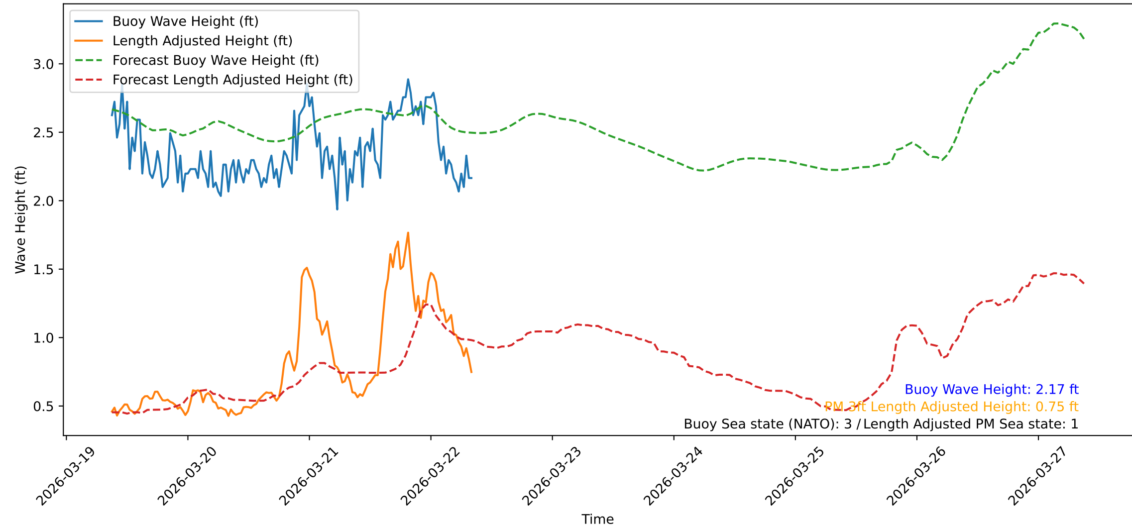
Wave Heights over Time for Green Beach at 2026-03-22 09:01:10
