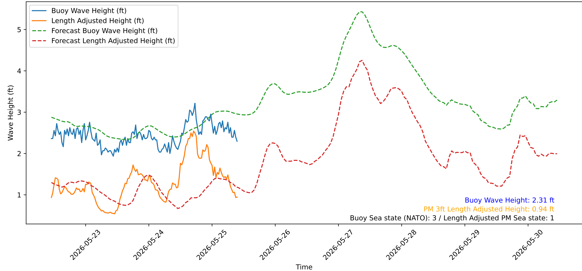
Wave Heights over Time for Red Beach at 2026-05-25 10:30:50
