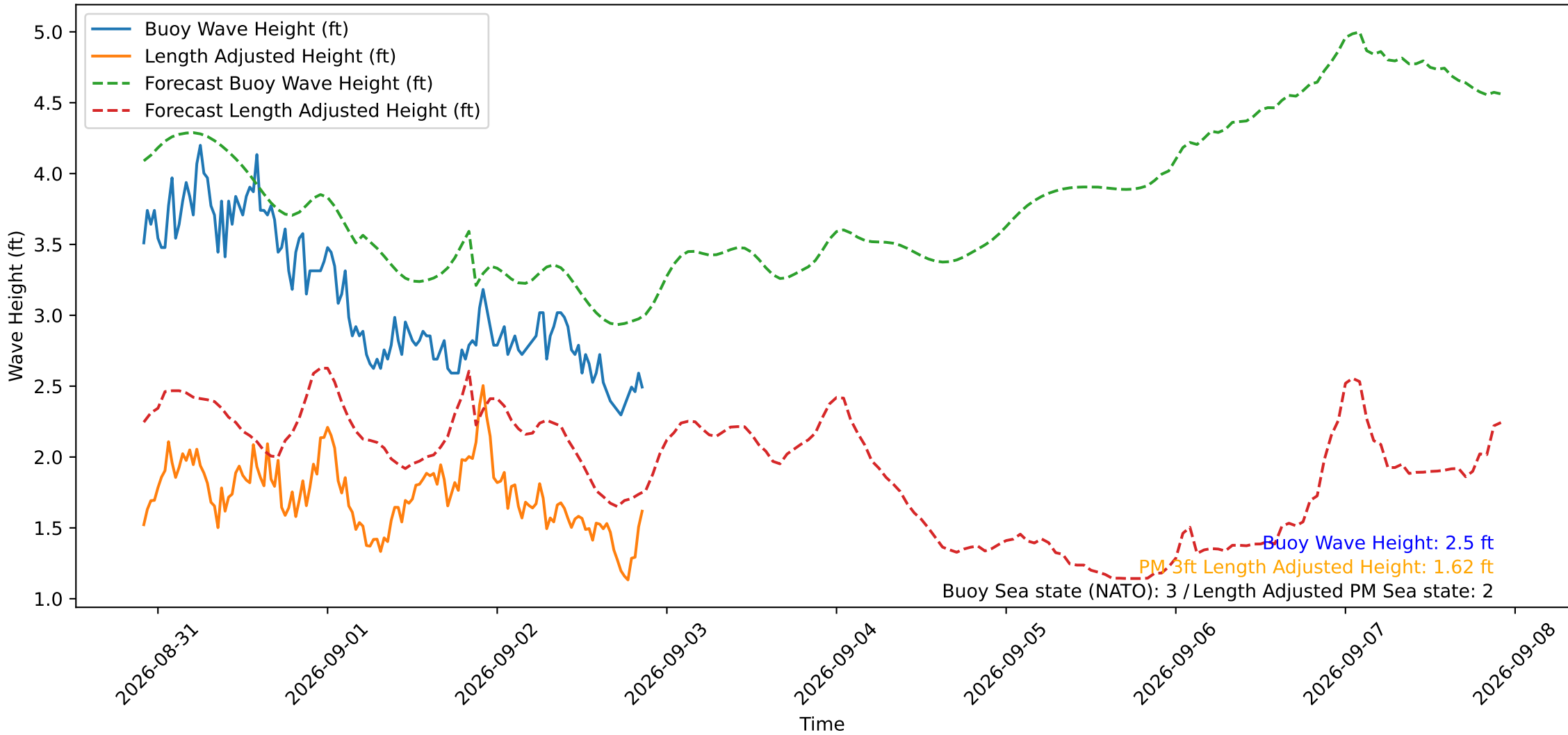
Wave Heights over Time for Red Beach at 2026-09-02 21:30:50
