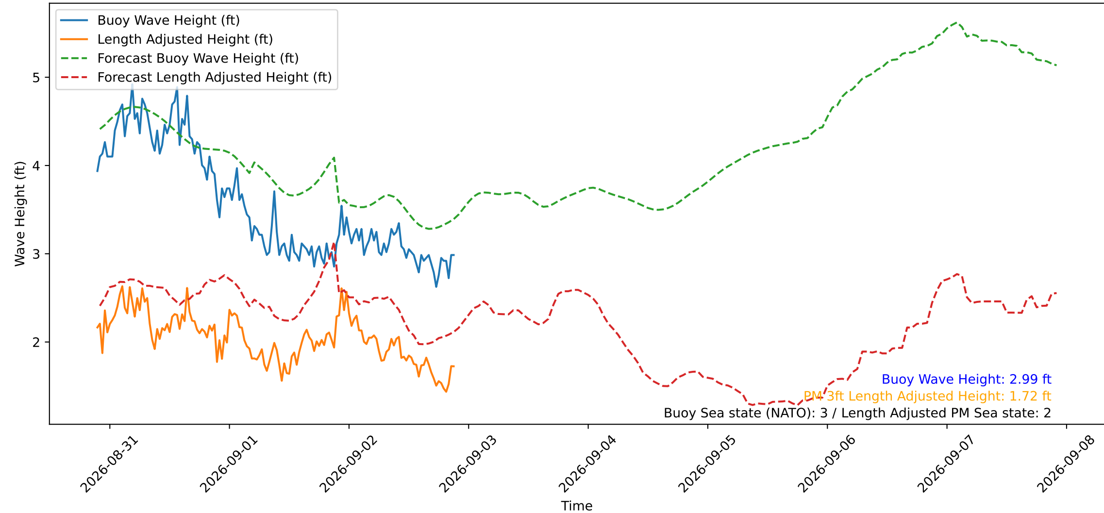
Wave Heights over Time for Oceanside Harbor at 2026-09-02 21:30:30
