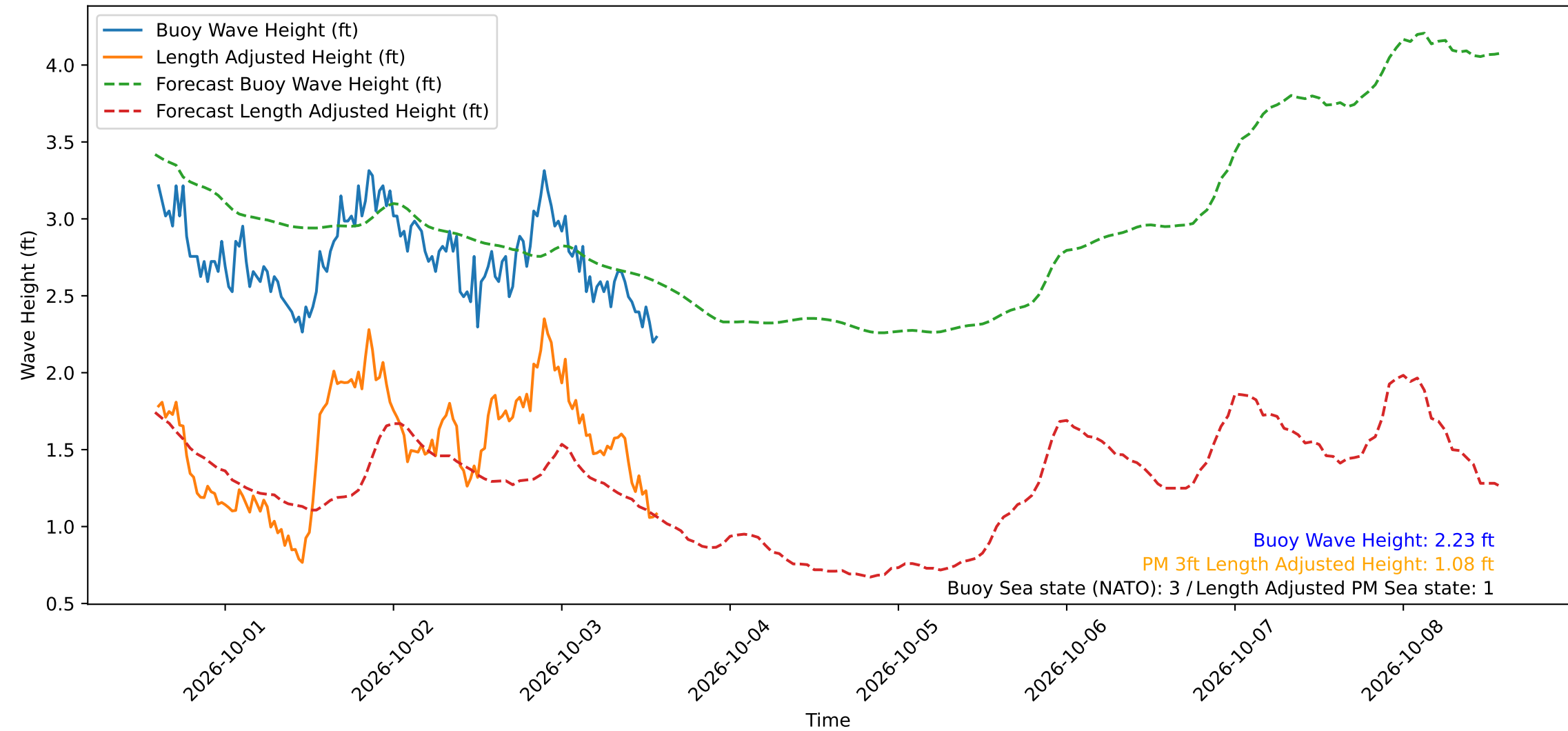
Wave Heights over Time for Oceanside Harbor at 2026-10-03 14:20:29
