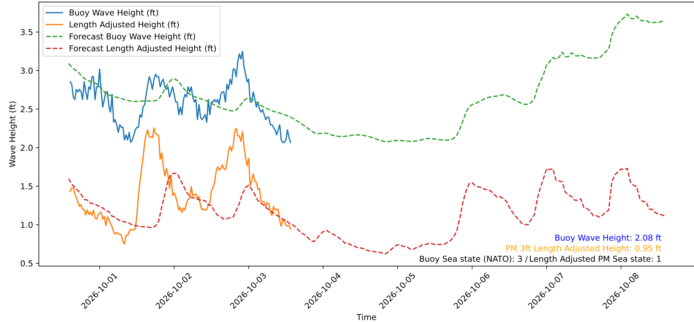
Wave Heights over Time for Red Beach at 2026-10-03 14:20:50
