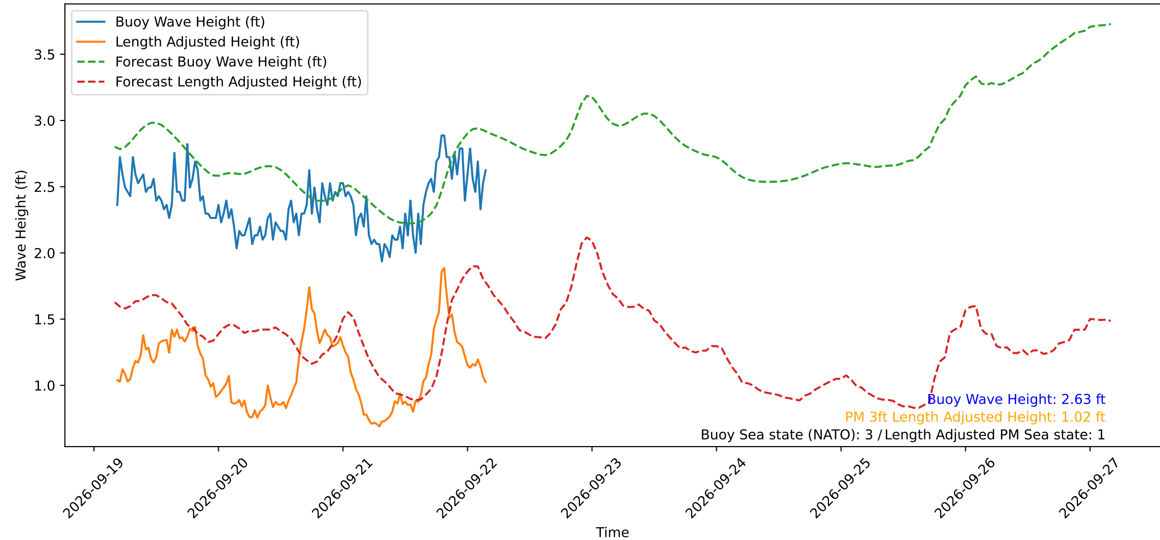
Wave Heights over Time for Red Beach at 2026-09-22 04:10:48
