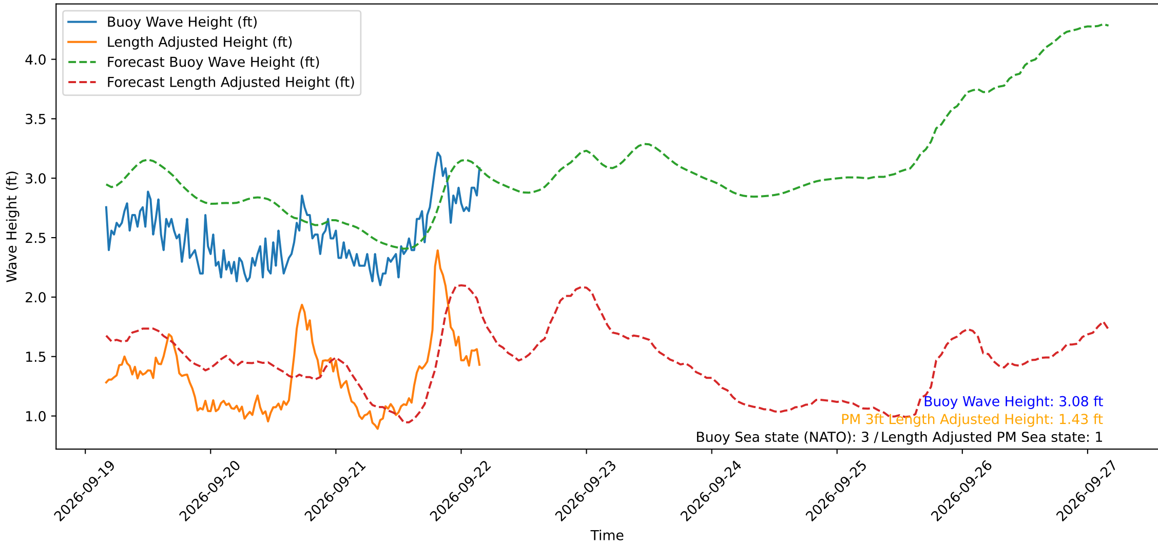
Wave Heights over Time for Oceanside Harbor at 2026-09-22 04:10:29
