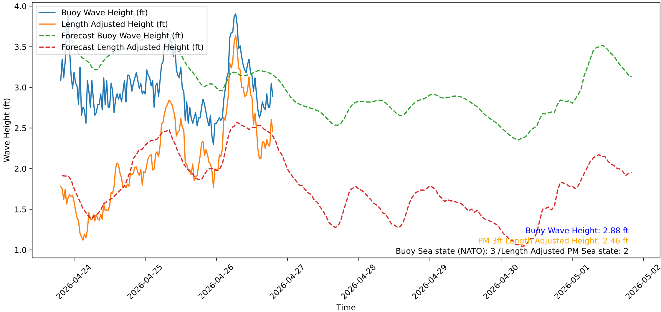
Wave Heights over Time for Oceanside Harbor at 2026-04-26 19:40:30
