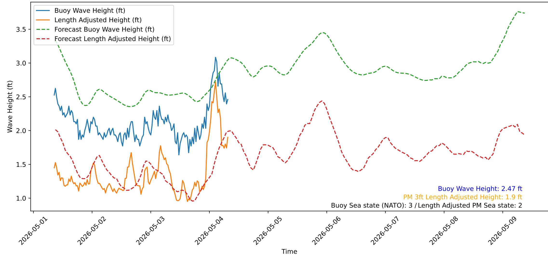
Wave Heights over Time for Oceanside Harbor at 2026-05-04 08:40:31
