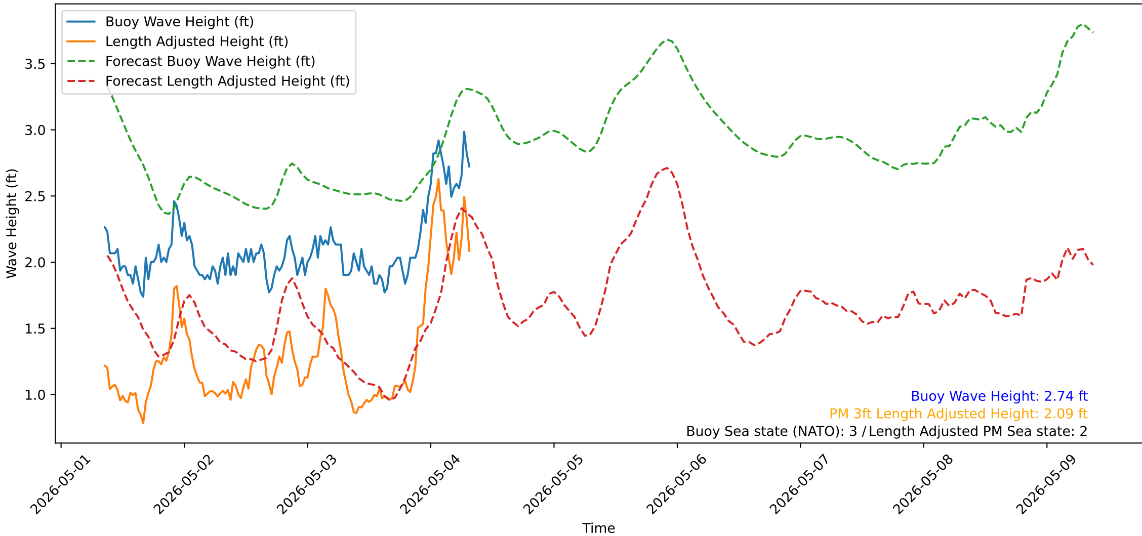
Wave Heights over Time for Green Beach at 2026-05-04 08:41:13
