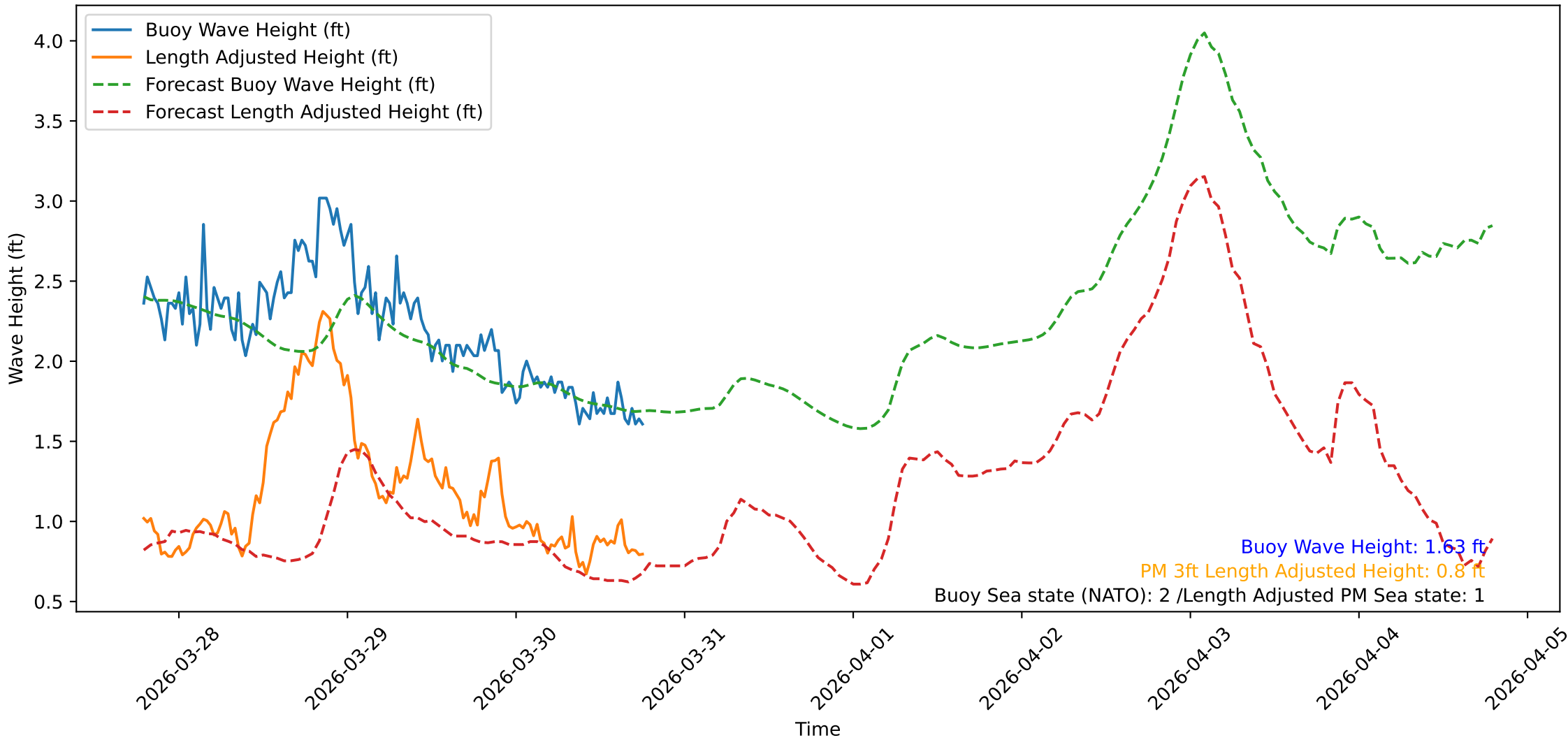
Wave Heights over Time for Red Beach at 2026-03-30 18:40:47
