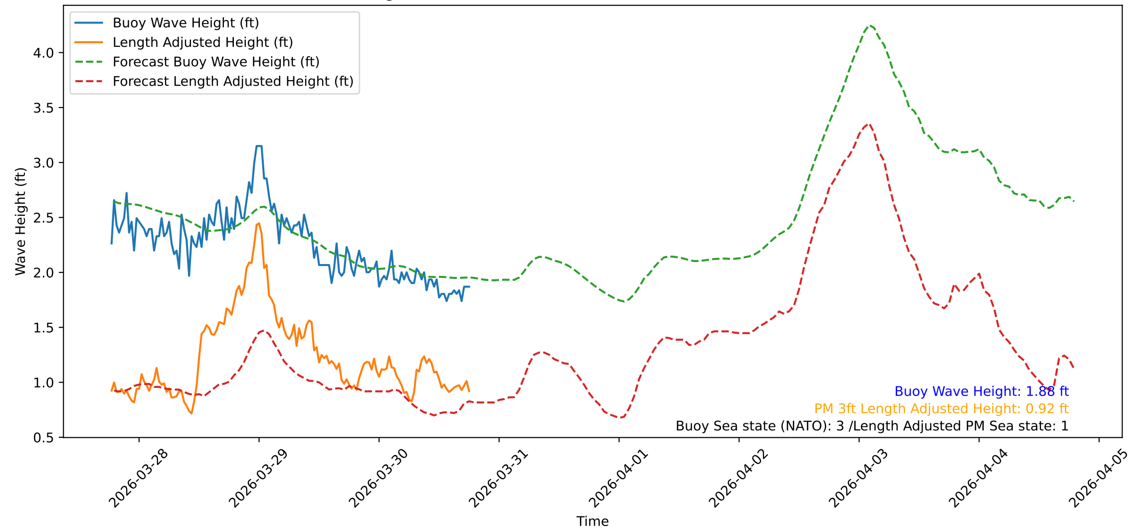
Wave Heights over Time for Oceanside Harbor at 2026-03-30 18:40:31
